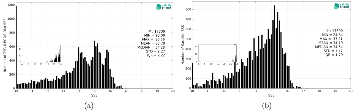
Figure 3: Histograms of SSS from TSG (LEGOS-DM) (a) and CCI SSS L4 Merged-OI v4.41 - 30-day running (ESA) (b) considering all match-up pairs per bins of 0.1 over the Congo river plume Pi-MEP region and for the full satellite product period.
