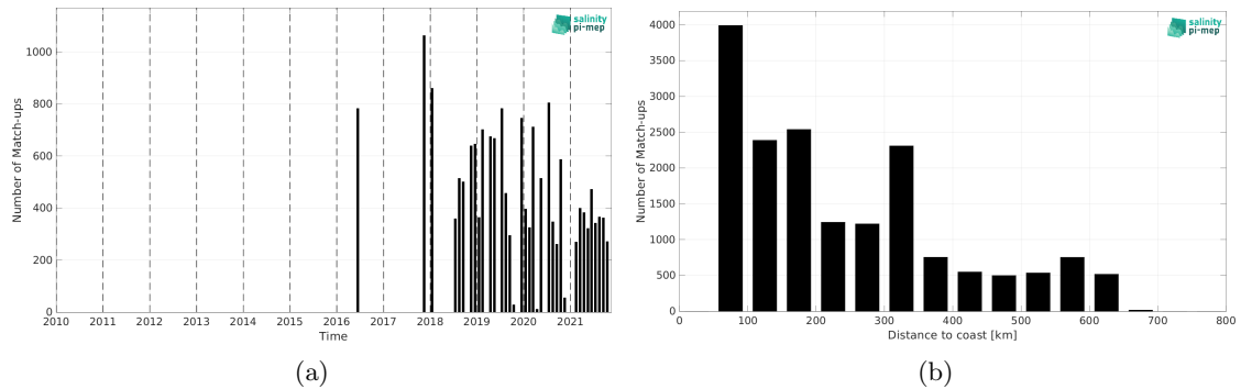
Figure 2: Number of match-ups between TSG (LEGOS-DM) and CCI SSS L4 Merged-OI v4.41 - 30-day running (ESA) SSS as a function of time (a) and as function of the distance to coast (b) over the Congo river plume Pi-MEP region and for the full satellite product period.
