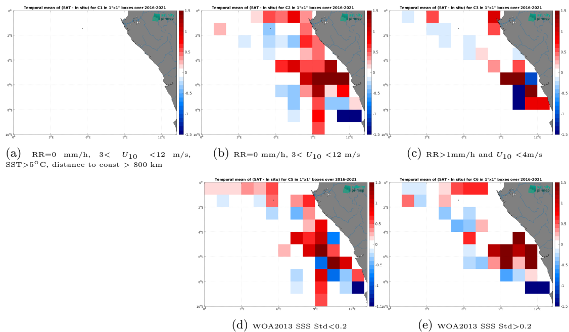
Figure 14: Temporal mean gridded over spatial boxes of size 1^\circ \times 1^\circ of \Delta SSS (CCI SSS L4 Merged-OI v4.41 - 30-day running (ESA) - TSG (LEGOS-DM)) for 5 different subdatasets corresponding to:RR=0 mm/h, 3 < U_{10} < 12 m/s, SST > 5^\circ\text{C} , distance to coast > 800 km (a), RR=0 mm/h, 3 < U_{10} < 12 m/s (b), RR > 1 mm/h and U_{10} < 4 m/s (c), WOA2013 SSS Std < 0.2 (d), WOA2013 SSS Std > 0.2 (e).
