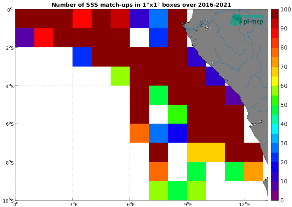
Figure 5: Number of SSS match-ups between TSG (LEGOS-DM) SSS and the CCI SSS L4 Merged-OI v4.41 - 30-day running (ESA) SSS product for the Congo river plume Pi-MEP region over 1^\circ \times 1^\circ boxes and for the full satellite product period.
