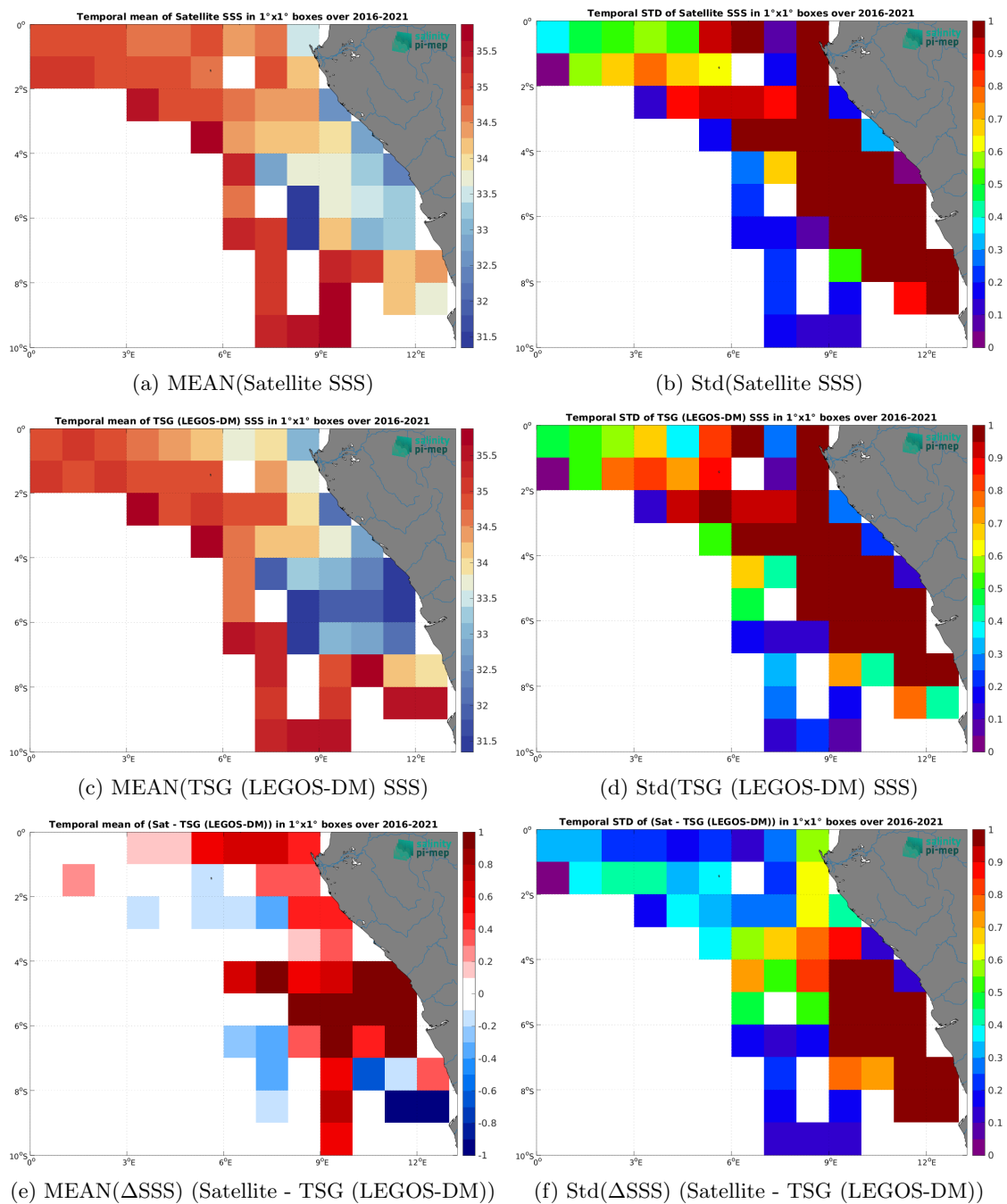
Figure 7: Temporal mean (left) and Std (right) of SSS from CCI SSS L4 Merged-OI v4.41 - 30-day running (ESA) (top), TSG (LEGOS-DM) (middle), and of \Delta SSS (Satellite - TSG (LEGOS-DM)). Only match-up pairs are used to generate these maps.
