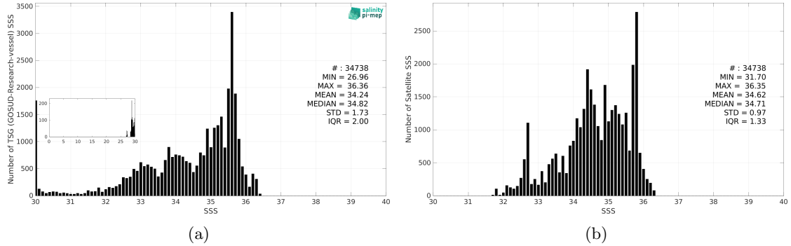
Figure 3: Histograms of SSS from TSG (GOSUD-Research-vessel) (a) and CCI SSS L4 Merged-OI v4.41 - 30-day running (ESA) (b) considering all match-up pairs per bins of 0.1 over the Congo river plume Pi-MEP region and for the full satellite product period.
