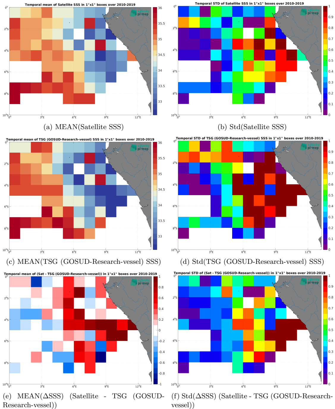
Figure 7: Temporal mean (left) and Std (right) of SSS from CCI SSS L4 Merged-OI v4.41 - 30-day running (ESA) (top), TSG (GOSUD-Research-vessel) (middle), and of \Delta SSS (Satellite - TSG (GOSUD-Research-vessel)). Only match-up pairs are used to generate these maps.
