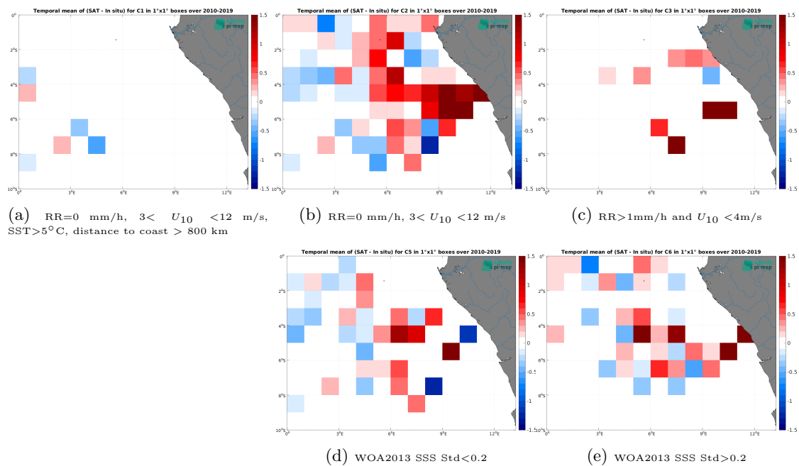
Figure 14: Temporal mean gridded over spatial boxes of size 1^\circ \times 1^\circ of \Delta SSS (CCI SSS L4 Merged-OI v4.41 - 30-day running (ESA) - TSG (GOSUD-Research-vessel)) for 5 different subdatasets corresponding to:RR=0 mm/h, 3 < U_{10} < 12 m/s, SST > 5^\circ\text{C} , distance to coast > 800 km (a), RR=0 mm/h, 3 < U_{10} < 12 m/s (b), RR > 1 mm/h and U_{10} < 4 m/s (c), WOA2013 SSS Std < 0.2 (d), WOA2013 SSS Std > 0.2 (e).
