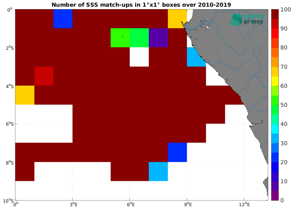
Figure 5: Number of SSS match-ups between TSG (GOSUD-Research-vessel) SSS and the CCI SSS L4 Merged-OI v4.41 - 30-day running (ESA) SSS product for the Congo river plume Pi-MEP region over 1^\circ \times 1^\circ boxes and for the full satellite product period.
