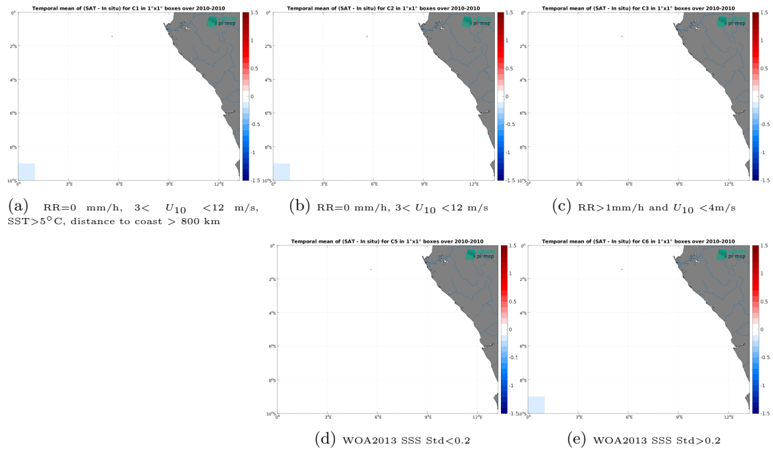
Figure 12: Temporal mean gridded over spatial boxes of size 1^\circ \times 1^\circ of \Delta SSS (CCI SSS L4 Merged-OI v4.4 - 7-day running (ESA) - TSG (SAMOS)) for 5 different subdatasets corresponding to:RR=0 mm/h, 3 < U_{10} < 12 m/s, SST > 5^\circ\text{C} , distance to coast > 800 km (a), RR=0 mm/h, 3 < U_{10} < 12 m/s (b), RR > 1 mm/h and U_{10} < 4 m/s (c), WOA2013 SSS Std < 0.2 (d), WOA2013 SSS Std > 0.2 (e).
