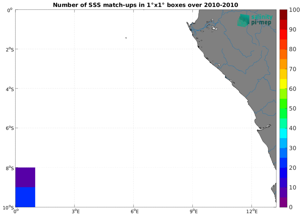
Figure 4: Number of SSS match-ups between TSG (SAMOS) SSS and the CCI SSS L4 Merged-OI v4.4 - 7-day running (ESA) SSS product for the Congo river plume Pi-MEP region over 1^\circ \times 1^\circ boxes and for the full satellite product period.
