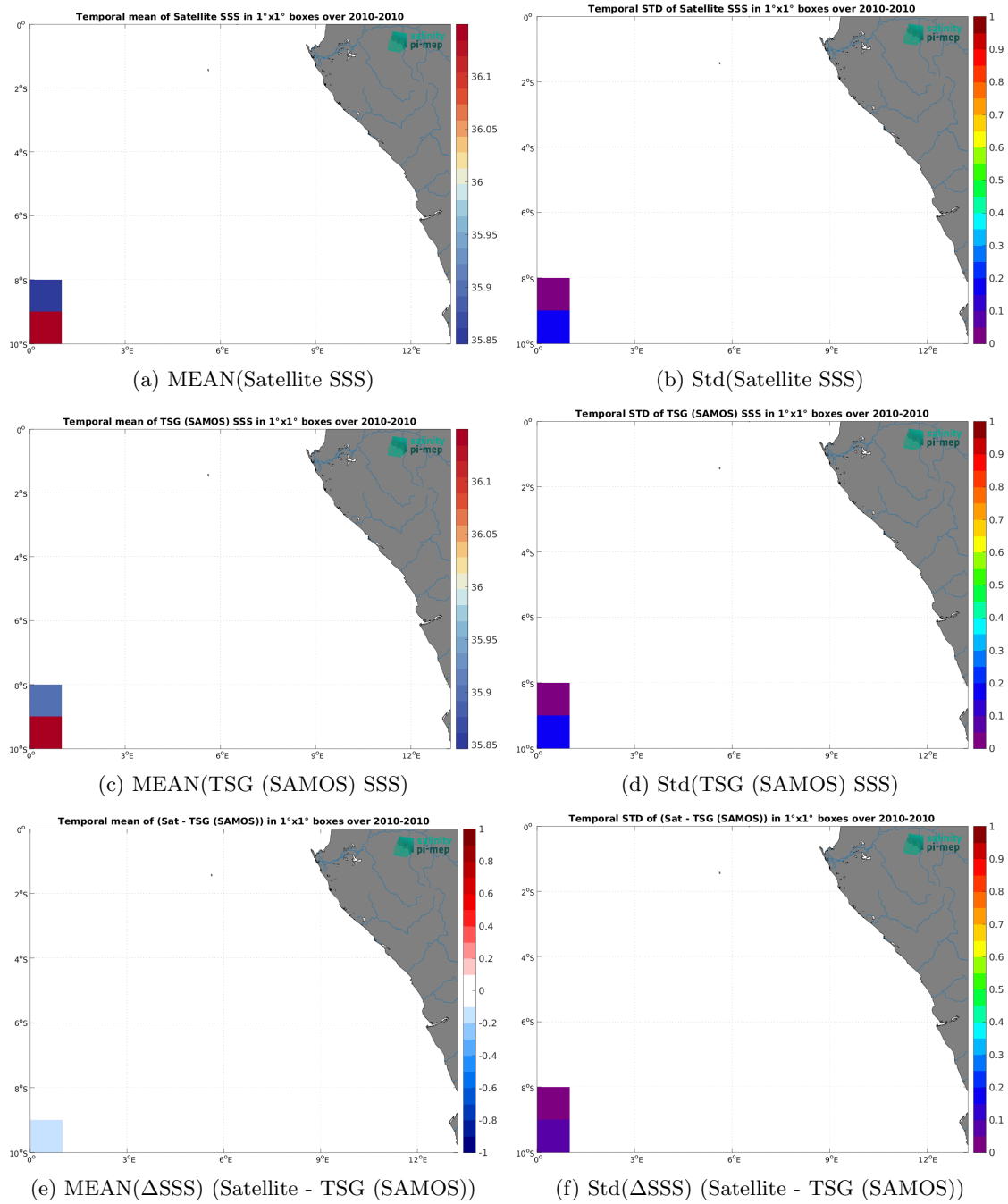
Figure 6: Temporal mean (left) and Std (right) of SSS from CCI SSS L4 Merged-OI v4.4 - 7-day running (ESA) (top), TSG (SAMOS) (middle), and of \Delta SSS (Satellite - TSG (SAMOS)). Only match-up pairs are used to generate these maps.
