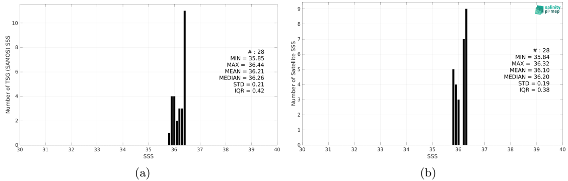
Figure 2: Histograms of SSS from TSG (SAMOS) (a) and CCI SSS L4 Merged-OI v4.4 - 7-day running (ESA) (b) considering all match-up pairs per bins of 0.1 over the Congo river plume Pi-MEP region and for the full satellite product period.
