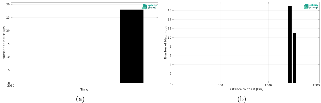
Figure 1: Number of match-ups between TSG (SAMOS) and CCI SSS L4 Merged-OI v4.4 - 7-day running (ESA) SSS as a function of time (a) and as function of the distance to coast (b) over the Congo river plume Pi-MEP region and for the full satellite product period.
