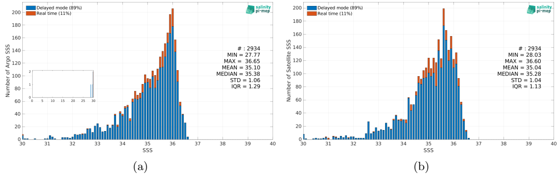
Figure 2: Histograms of SSS from Argo (a) and CCI SSS L4 Merged-OI v4.4 - 30-day running (ESA) (b) considering all match-up pairs per bins of 0.1 over the Congo river plume Pi-MEP region and for the full satellite product period.
