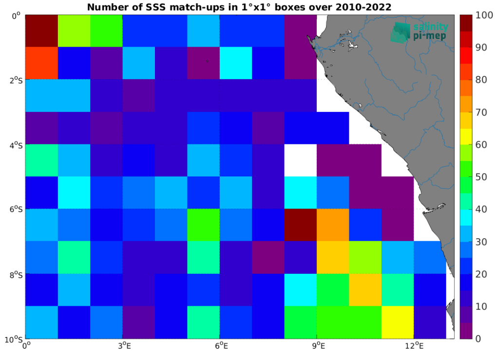
Figure 4: Number of SSS match-ups between Argo SSS and the CCI SSS L4 Merged-OI v4.4 - 30-day running (ESA) SSS product for the Congo river plume Pi-MEP region over 1^\circ \times 1^\circ boxes and for the full satellite product period.
