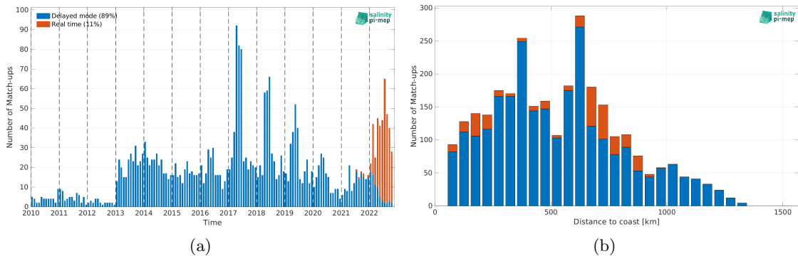
Figure 1: Number of match-ups between Argo and CCI SSS L4 Merged-OI v4.4 - 30-day running (ESA) SSS as a function of time (a) and as function of the distance to coast (b) over the Congo river plume Pi-MEP region and for the full satellite product period.
