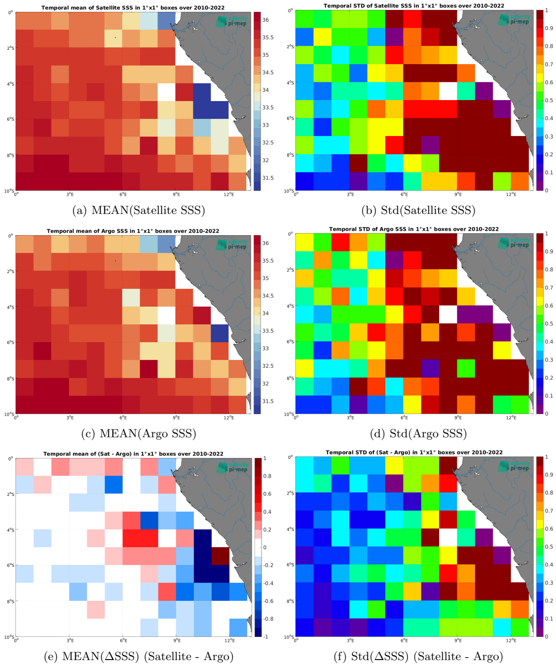
Figure 6: Temporal mean (left) and Std (right) of SSS from CCI SSS L4 Merged-OI v4.4 - 30-day running (ESA) (top), Argo (middle), and of \Delta SSS (Satellite - Argo). Only match-up pairs are used to generate these maps.
