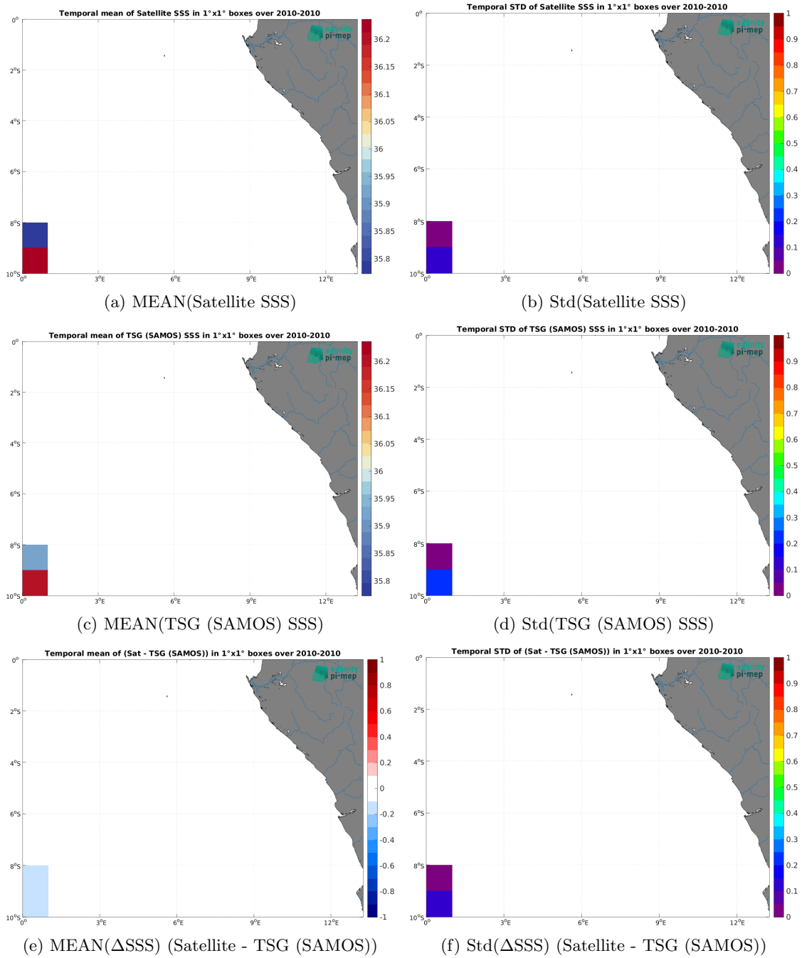
Figure 6: Temporal mean (left) and Std (right) of SSS from CCI SSS L4 Merged-OI v3.2 - 7-day running (ESA) (top), TSG (SAMOS) (middle), and of \Delta SSS (Satellite - TSG (SAMOS)). Only match-up pairs are used to generate these maps.
