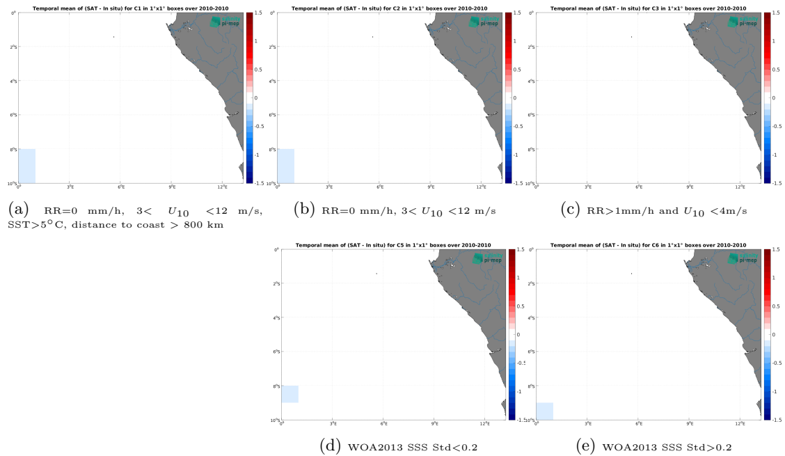
Figure 12: Temporal mean gridded over spatial boxes of size 1^\circ \times 1^\circ of \Delta SSS (CCI SSS L4 Merged-OI v3.2 - 7-day running (ESA) - TSG (SAMOS)) for 5 different subdatasets corresponding to:RR=0 mm/h, 3 < U_{10} < 12 m/s, SST >5^\circ C, distance to coast > 800 km (a), RR=0 mm/h, 3 < U_{10} < 12 m/s (b), RR >1 mm/h and U_{10} < 4 m/s (c), WOA2013 SSS Std <0.2 (d), WOA2013 SSS Std >0.2 (e).
