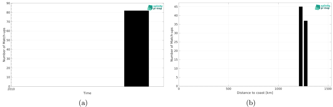
Figure 1: Number of match-ups between TSG (SAMOS) and CCI SSS L4 Merged-OI v3.2 - 7-day running (ESA) SSS as a function of time (a) and as function of the distance to coast (b) over the Congo river plume Pi-MEP region and for the full satellite product period.
