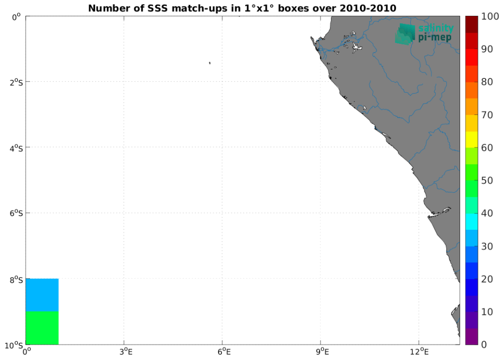
Figure 4: Number of SSS match-ups between TSG (SAMOS) SSS and the CCI SSS L4 Merged-OI v3.2 - 7-day running (ESA) SSS product for the Congo river plume Pi-MEP region over 1^\circ \times 1^\circ boxes and for the full satellite product period.
