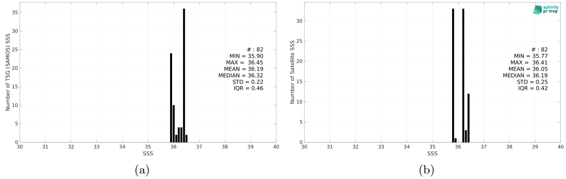
Figure 2: Histograms of SSS from TSG (SAMOS) (a) and CCI SSS L4 Merged-OI v3.2 - 7-day running (ESA) (b) considering all match-up pairs per bins of 0.1 over the Congo river plume Pi-MEP region and for the full satellite product period.
