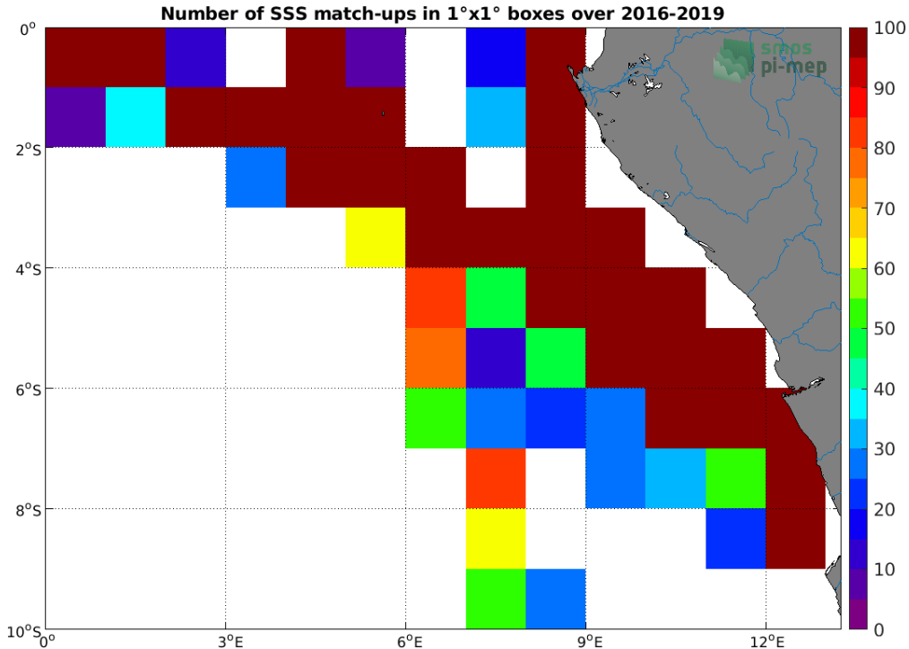
Figure 4: Number of SSS match-ups between TSG (LEGOS-DM) SSS and the CCI SSS L4 Merged-OI v3.2 - 7-day running (ESA) SSS product for the Congo river plume Pi-MEP region over 1°x1° boxes and for the full satellite product period.
