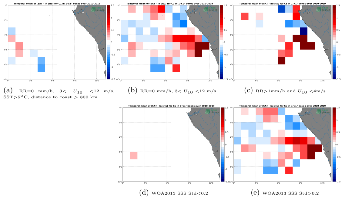
Figure 12: Temporal mean gridded over spatial boxes of size 1^\circ \times 1^\circ of \Delta SSS (CCI SSS L4 Merged-OI v3.2 - 7-day running (ESA) - TSG (GOSUD-Research-vessel)) for 5 different subdatasets corresponding to: RR=0 mm/h, 3 < U_{10} < 12 m/s, SST > 5^\circ\text{C} , distance to coast > 800 km (a), RR=0 mm/h, 3 < U_{10} < 12 m/s (b), RR > 1 mm/h and U_{10} < 4 m/s (c), WOA2013 SSS Std < 0.2 (d), WOA2013 SSS Std > 0.2 (e).
