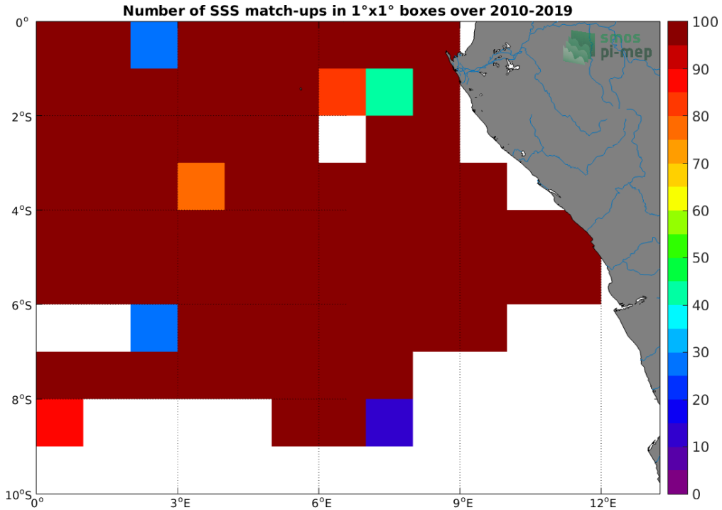
Figure 4: Number of SSS match-ups between TSG (GOSUD-Research-vessel) SSS and the CCI SSS L4 Merged-OI v3.2 - 7-day running (ESA) SSS product for the Congo river plume Pi-MEP region over 1^{\circ} \times 1^{\circ} boxes and for the full satellite product period.
