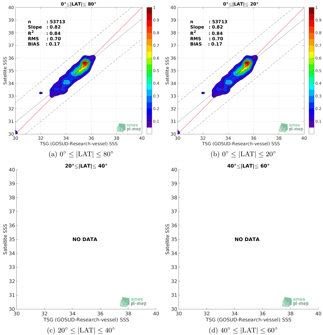
Figure 9: Contour maps of the concentration of CCI SSS L4 Merged-OI v3.2 - 7-day running (ESA) SSS ( y -axis) versus TSG (GOSUD-Research-vessel) SSS ( x -axis) at match-up pairs for different latitude bands. For each plot, the red line shows x=y . The black thin and dashed lines indicate a linear fit through the data cloud and the \pm 95\% confidence levels, respectively. The number match-up pairs n , the slope and R^2 coefficient of the linear fit, the root mean square (RMS) and the mean bias between satellite and in situ data are indicated for each latitude band in each plots.
