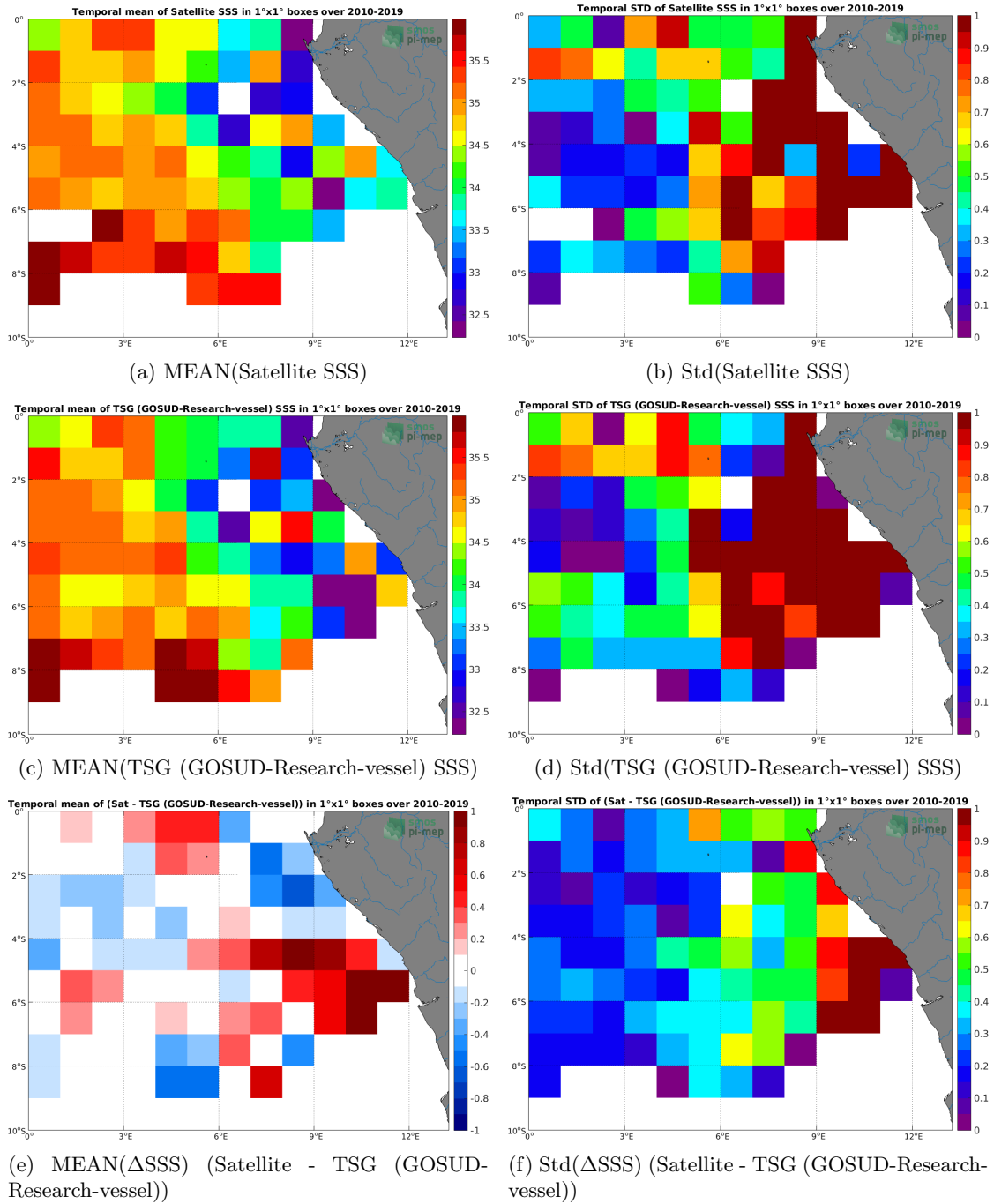
Figure 6: Temporal mean (left) and Std (right) of SSS from CCI SSS L4 Merged-OI v3.2 - 7-day running (ESA) (top), TSG (GOSUD-Research-vessel) (middle), and of \Delta SSS (Satellite - TSG (GOSUD-Research-vessel)). Only match-up pairs are used to generate these maps.
