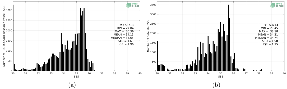
Figure 2: Histograms of SSS from TSG (GOSUD-Research-vessel) (a) and CCI SSS L4 Merged-OI v3.2 - 7-day running (ESA) (b) considering all match-up pairs per bins of 0.1 over the Congo river plume Pi-MEP region and for the full satellite product period.
