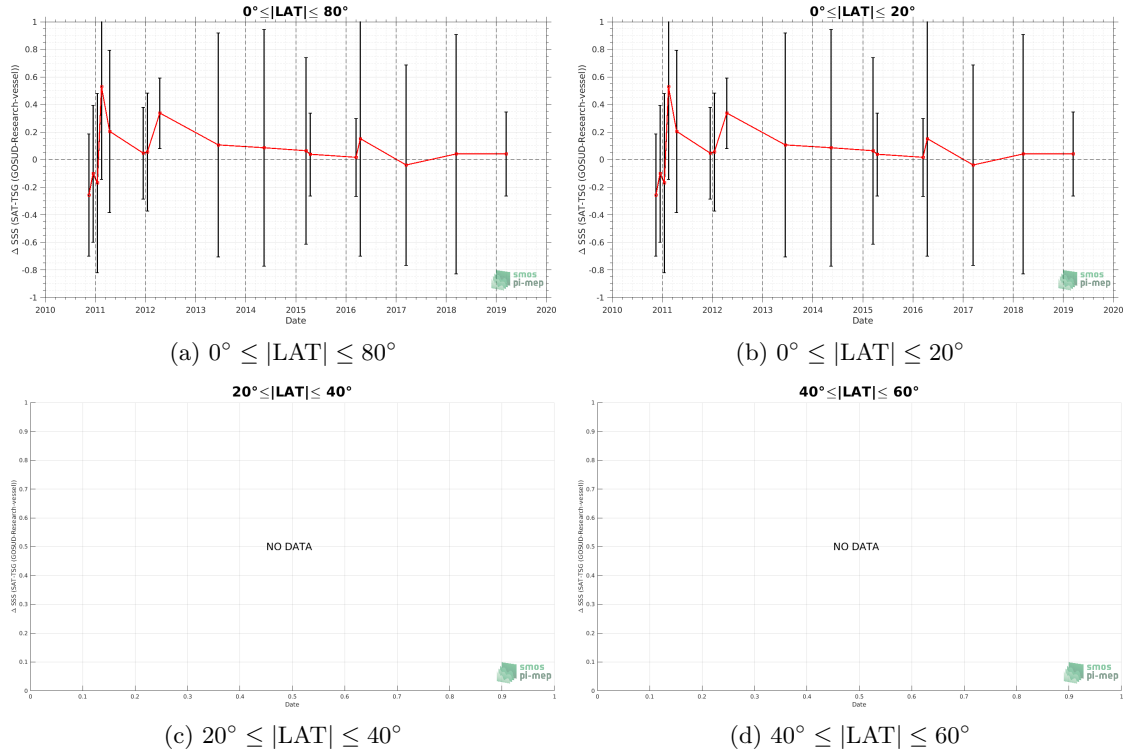
Figure 10: Monthly median (red curves) of \Delta SSS (Satellite - in situ ) between CCI SSS L4 Merged-OI v3.2 - 7-day running (ESA) and TSG (GOSUD-Research-vessel) SSS as function of time for all the collected Pi-MEP match-up pairs estimated over the Congo river plume Pi-MEP region and for the full satellite product period are shown for different latitude bands: (a) 80^\circ\text{S}-80^\circ\text{N} , (b) 20^\circ\text{S}-20^\circ\text{N} , (c) 40^\circ\text{S}-20^\circ\text{S} and 20^\circ\text{N}-40^\circ\text{N} and (d) 60^\circ\text{S}-40^\circ\text{S} and 40^\circ\text{N}-60^\circ\text{N} .
