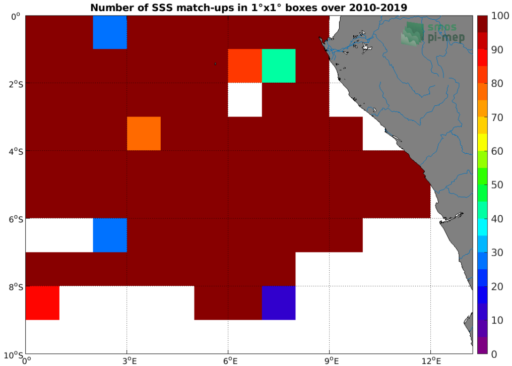
Figure 4: Number of SSS match-ups between TSG (GOSUD-Research-vessel) SSS and the CCI SSS L4 Merged-OI v3.2 - 7-day running (ESA) SSS product for the Congo river plume Pi-MEP region over 1°x1° boxes and for the full satellite product period.
