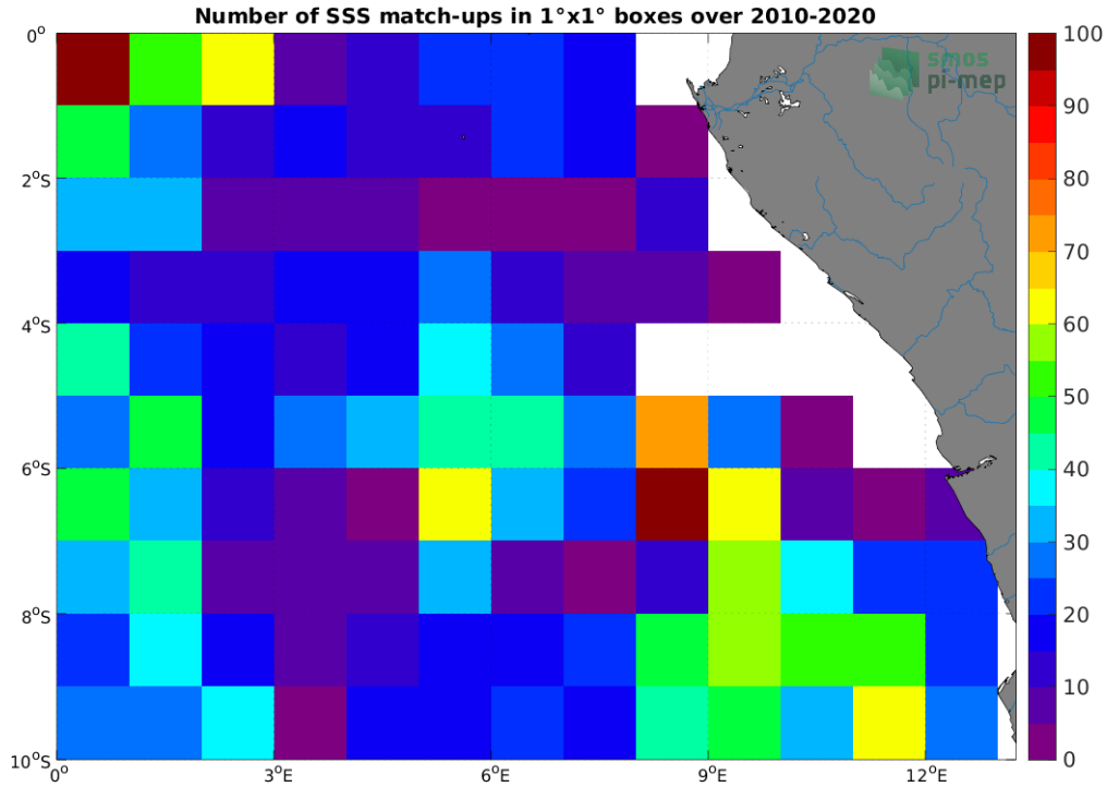
Figure 4: Number of SSS match-ups between Argo SSS and the CCI SSS L4 Merged-OI v3.2 - 7-day running (ESA) SSS product for the Congo river plume Pi-MEP region over 1^\circ \times 1^\circ boxes and for the full satellite product period.
