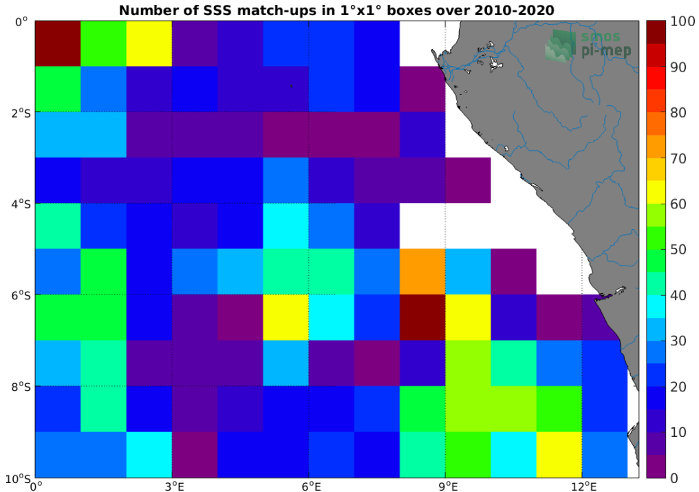
Figure 4: Number of SSS match-ups between Argo SSS and the CCI SSS L4 Merged-OI v3.2 - 7-day running (ESA) SSS product for the Congo river plume Pi-MEP region over 1°x1° boxes and for the full satellite product period.
