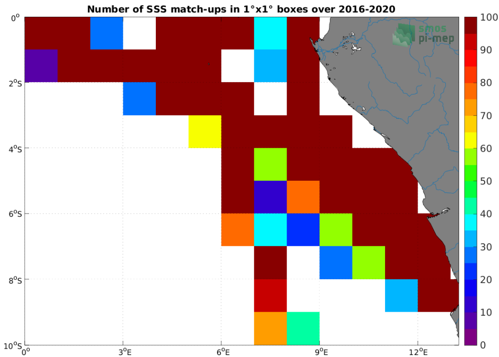
Figure 4: Number of SSS match-ups between TSG (LEGOS-DM) SSS and the CCI SSS L4 Merged-OI v3.2 - 30-day running (ESA) SSS product for the Congo river plume Pi-MEP region over 1^\circ \times 1^\circ boxes and for the full satellite product period.
