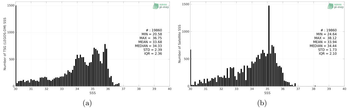
Figure 2: Histograms of SSS from TSG (LEGOS-DM) (a) and CCI SSS L4 Merged-OI v3.2 - 30-day running (ESA) (b) considering all match-up pairs per bins of 0.1 over the Congo river plume Pi-MEP region and for the full satellite product period.
