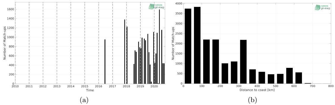
Figure 1: Number of match-ups between TSG (LEGOS-DM) and CCI SSS L4 Merged-OI v3.2 - 30-day running (ESA) SSS as a function of time (a) and as function of the distance to coast (b) over the Congo river plume Pi-MEP region and for the full satellite product period.
