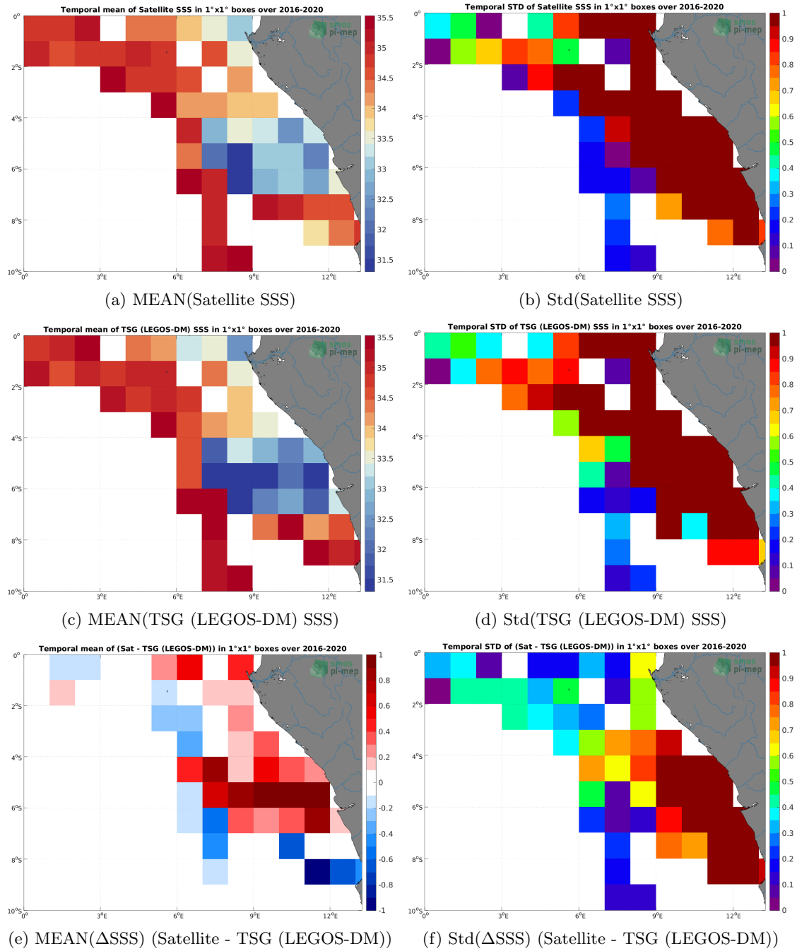
Figure 6: Temporal mean (left) and Std (right) of SSS from CCI SSS L4 Merged-OI v3.2 - 30-day running (ESA) (top), TSG (LEGOS-DM) (middle), and of \Delta SSS (Satellite - TSG (LEGOS-DM)). Only match-up pairs are used to generate these maps.
