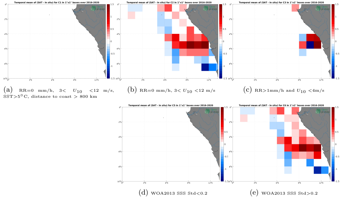
Figure 12: Temporal mean gridded over spatial boxes of size 1^{\circ}\times 1^{\circ} of \Delta\text{SSS} (CCI SSS L4 Merged-OI v3.2 - 30-day running (ESA) - TSG (LEGOS-DM)) for 5 different subdatasets corresponding to:RR=0 mm/h, 3 < U_{10} < 12 m/s, SST >5^{\circ}\text{C} , distance to coast > 800 km (a), RR=0 mm/h, 3 < U_{10} < 12 m/s (b), RR >1 mm/h and U_{10} < 4 m/s (c), WOA2013 SSS Std <0.2 (d), WOA2013 SSS Std >0.2 (e).
