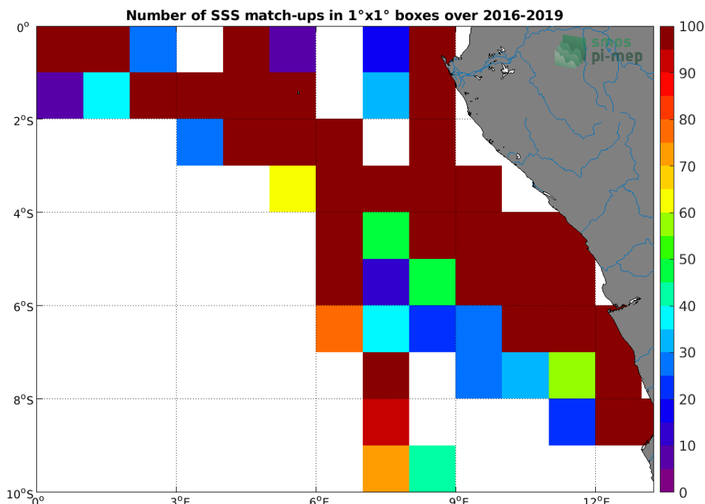
Figure 4: Number of SSS match-ups between TSG (LEGOS-DM) SSS and the CCI SSS L4 Merged-OI v3.2 - 30-day running (ESA) SSS product for the Congo river plume Pi-MEP region over 1°x1° boxes and for the full satellite product period.
