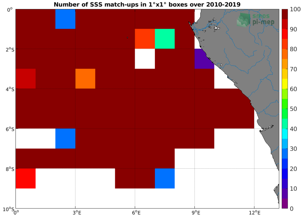
Figure 4: Number of SSS match-ups between TSG (GOSUD-Research-vessel) SSS and the CCI SSS L4 Merged-OI v3.2 - 30-day running (ESA) SSS product for the Congo river plume Pi-MEP region over 1°x1° boxes and for the full satellite product period.
