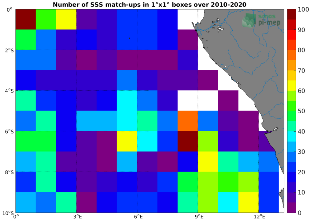
Figure 4: Number of SSS match-ups between Argo SSS and the CCI SSS L4 Merged-OI v3.2 - 30-day running (ESA) SSS product for the Congo river plume Pi-MEP region over 1^\circ \times 1^\circ boxes and for the full satellite product period.
