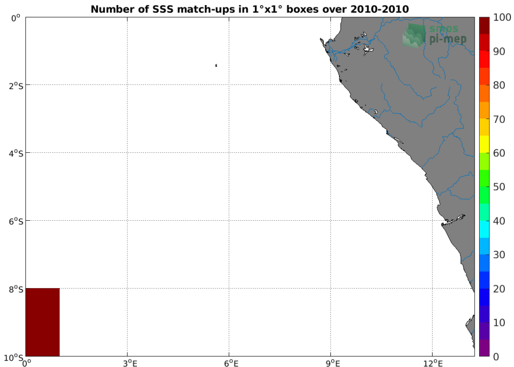
Figure 4: Number of SSS match-ups between TSG (SAMOS) SSS and the CCI SSS L4 Merged-OI v2.31 - 30-day running (ESA) SSS product for the Congo river plume Pi-MEP region over 1^\circ \times 1^\circ boxes and for the full satellite product period.
