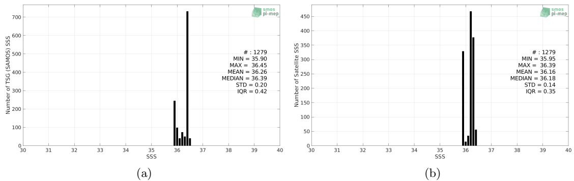
Figure 2: Histograms of SSS from TSG (SAMOS) (a) and CCI SSS L4 Merged-OI v2.31 - 30-day running (ESA) (b) considering all match-up pairs per bins of 0.1 over the Congo river plume Pi-MEP region and for the full satellite product period.
