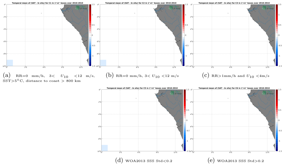
Figure 12: Temporal mean gridded over spatial boxes of size 1^\circ \times 1^\circ of \Delta SSS (CCI SSS L4 Merged-OI v2.31 - 30-day running (ESA) - TSG (SAMOS)) for 5 different subdatasets corresponding to: RR=0 mm/h, 3 < U_{10} < 12 m/s, SST >5^\circ C, distance to coast > 800 km (a), RR=0 mm/h, 3 < U_{10} < 12 m/s (b), RR >1 mm/h and U_{10} < 4 m/s (c), WOA2013 SSS Std <0.2 (d), WOA2013 SSS Std >0.2 (e).
