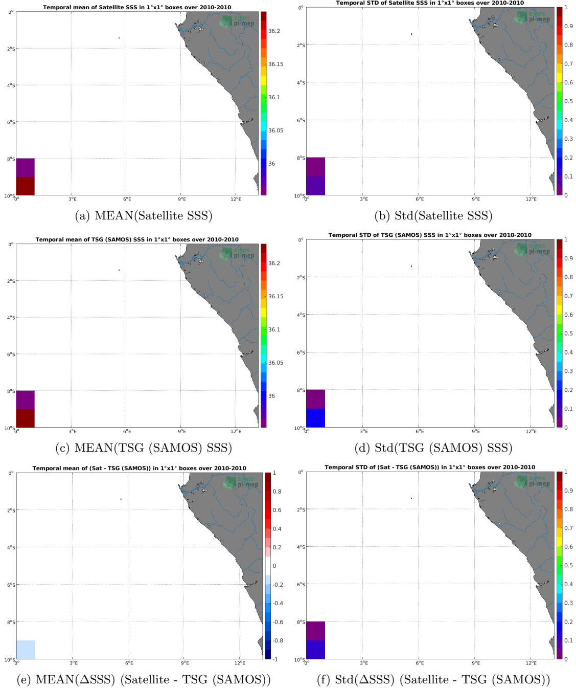
Figure 6: Temporal mean (left) and Std (right) of SSS from CCI SSS L4 Merged-OI v2.31 - 30-day running (ESA) (top), TSG (SAMOS) (middle), and of \Delta SSS (Satellite - TSG (SAMOS)). Only match-up pairs are used to generate these maps.
