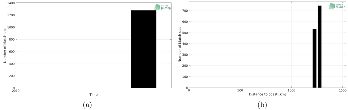
Figure 1: Number of match-ups between TSG (SAMOS) and CCI SSS L4 Merged-OI v2.31 - 30-day running (ESA) SSS as a function of time (a) and as function of the distance to coast (b) over the Congo river plume Pi-MEP region and for the full satellite product period.
