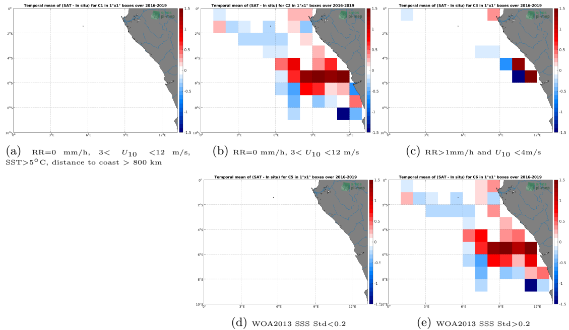
Figure 12: Temporal mean gridded over spatial boxes of size 1^{\circ}\times 1^{\circ} of \Delta\text{SSS} (CCI SSS L4 Merged-OI v2.31 - 30-day running (ESA) - TSG (LEGOS-DM)) for 5 different subdatasets corresponding to:RR=0 mm/h, 3 < U_{10} < 12 m/s, SST >5^{\circ}\text{C} , distance to coast > 800 km (a), RR=0 mm/h, 3 < U_{10} < 12 m/s (b), RR >1 mm/h and U_{10} < 4 m/s (c), WOA2013 SSS Std <0.2 (d), WOA2013 SSS Std >0.2 (e).
