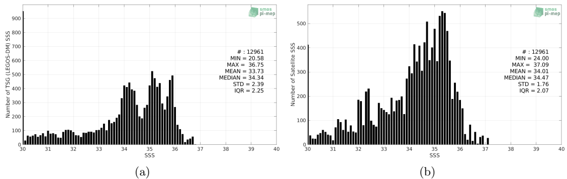
Figure 2: Histograms of SSS from TSG (LEGOS-DM) (a) and CCI SSS L4 Merged-OI v2.31 - 30-day running (ESA) (b) considering all match-up pairs per bins of 0.1 over the Congo river plume Pi-MEP region and for the full satellite product period.
