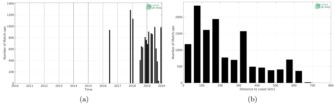
Figure 1: Number of match-ups between TSG (LEGOS-DM) and CCI SSS L4 Merged-OI v2.31 - 30-day running (ESA) SSS as a function of time (a) and as function of the distance to coast (b) over the Congo river plume Pi-MEP region and for the full satellite product period.
