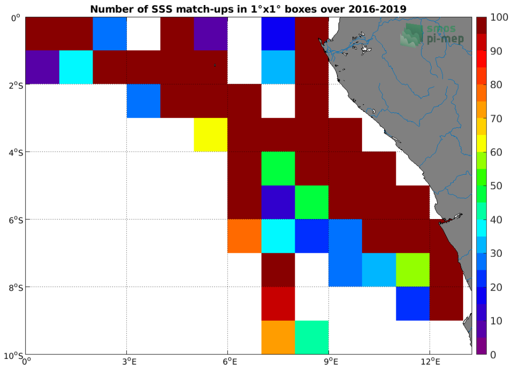
Figure 4: Number of SSS match-ups between TSG (LEGOS-DM) SSS and the CCI SSS L4 Merged-OI v2.31 - 30-day running (ESA) SSS product for the Congo river plume Pi-MEP region over 1^\circ \times 1^\circ boxes and for the full satellite product period.
