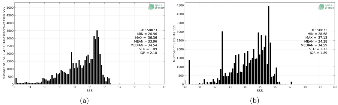
Figure 2: Histograms of SSS from TSG (GOSUD-Research-vessel) (a) and CCI SSS L4 Merged-OI v2.31 - 30-day running (ESA) (b) considering all match-up pairs per bins of 0.1 over the Congo river plume Pi-MEP region and for the full satellite product period.
