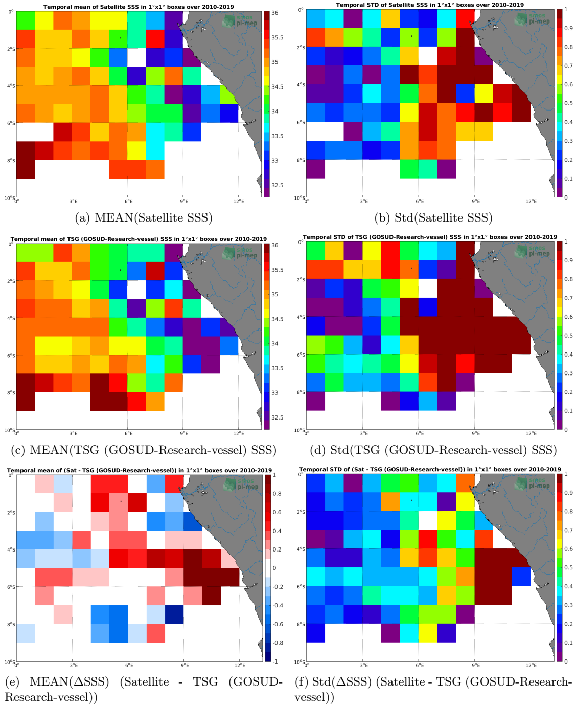
Figure 6: Temporal mean (left) and Std (right) of SSS from CCI SSS L4 Merged-OI v2.31 - 30-day running (ESA) (top), TSG (GOSUD-Research-vessel) (middle), and of \Delta SSS (Satellite - TSG (GOSUD-Research-vessel)). Only match-up pairs are used to generate these maps.
