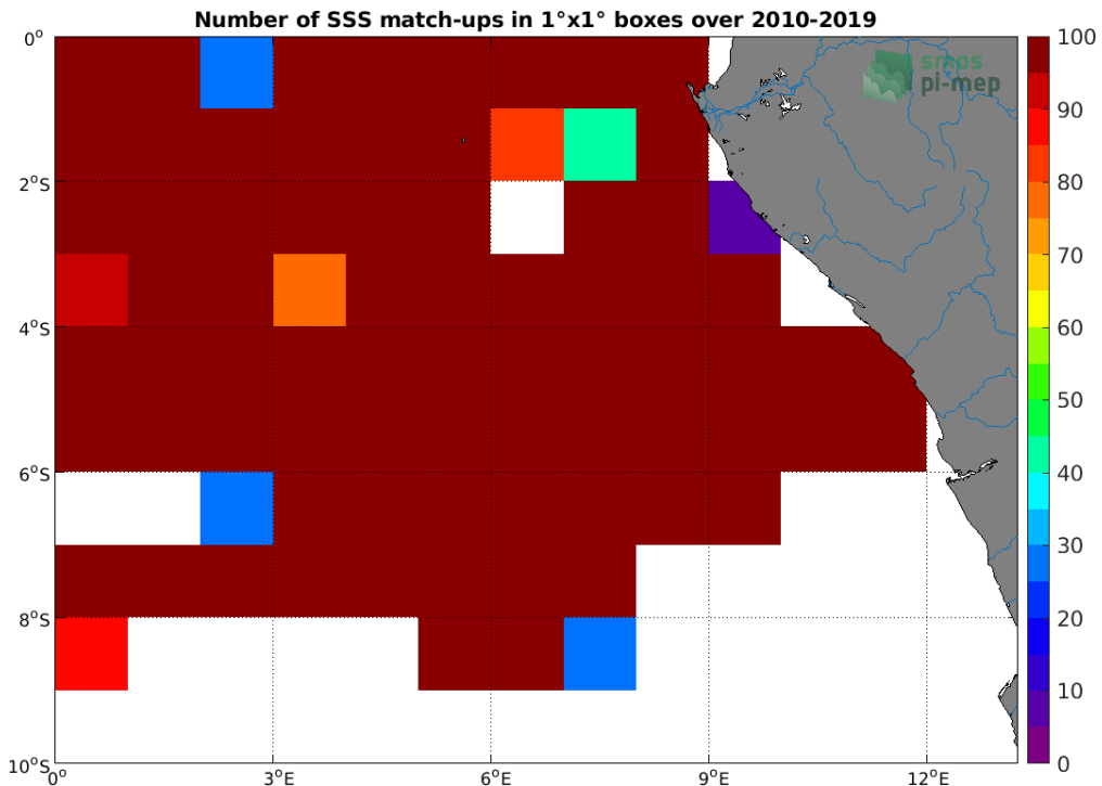
Figure 4: Number of SSS match-ups between TSG (GOSUD-Research-vessel) SSS and the CCI SSS L4 Merged-OI v2.31 - 30-day running (ESA) SSS product for the Congo river plume Pi-MEP region over 1^\circ \times 1^\circ boxes and for the full satellite product period.
