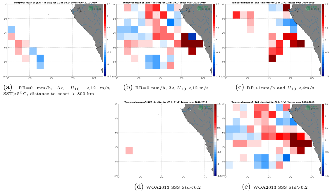
Figure 12: Temporal mean gridded over spatial boxes of size 1^\circ \times 1^\circ of \Delta SSS (CCI SSS L4 Merged-OI v2.31 - 30-day running (ESA) - TSG (GOSUD-Research-vessel)) for 5 different subdatasets corresponding to:RR=0 mm/h, 3 < U_{10} < 12 m/s, SST >5^\circ\text{C} , distance to coast > 800 km (a), RR=0 mm/h, 3 < U_{10} < 12 m/s (b), RR >1 mm/h and U_{10} < 4 m/s (c), WOA2013 SSS Std <0.2 (d), WOA2013 SSS Std >0.2 (e).
