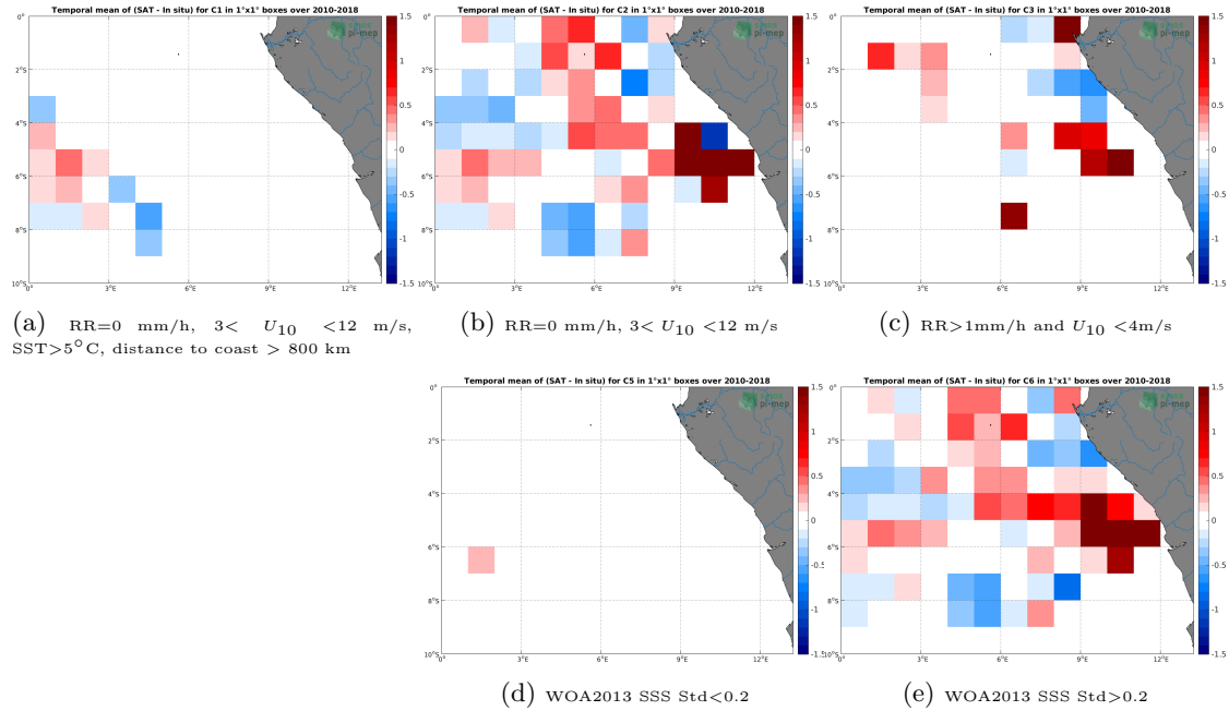
Figure 12: Temporal mean gridded over spatial boxes of size 1^{\circ}\times 1^{\circ} of \Delta SSS (CCI L4 Merged-OI v2.31 - 30-day running (ESA) - TSG (GOSUD-Research-vessel)) for 5 different subdatasets corresponding to:RR=0 mm/h, 3 < U_{10} < 12 m/s, SST > 5^{\circ}\text{C} , distance to coast > 800 km (a), RR=0 mm/h, 3 < U_{10} < 12 m/s (b), RR > 1 mm/h and U_{10} < 4 m/s (c), WOA2013 SSS Std < 0.2 (d), WOA2013 SSS Std > 0.2 (e).
