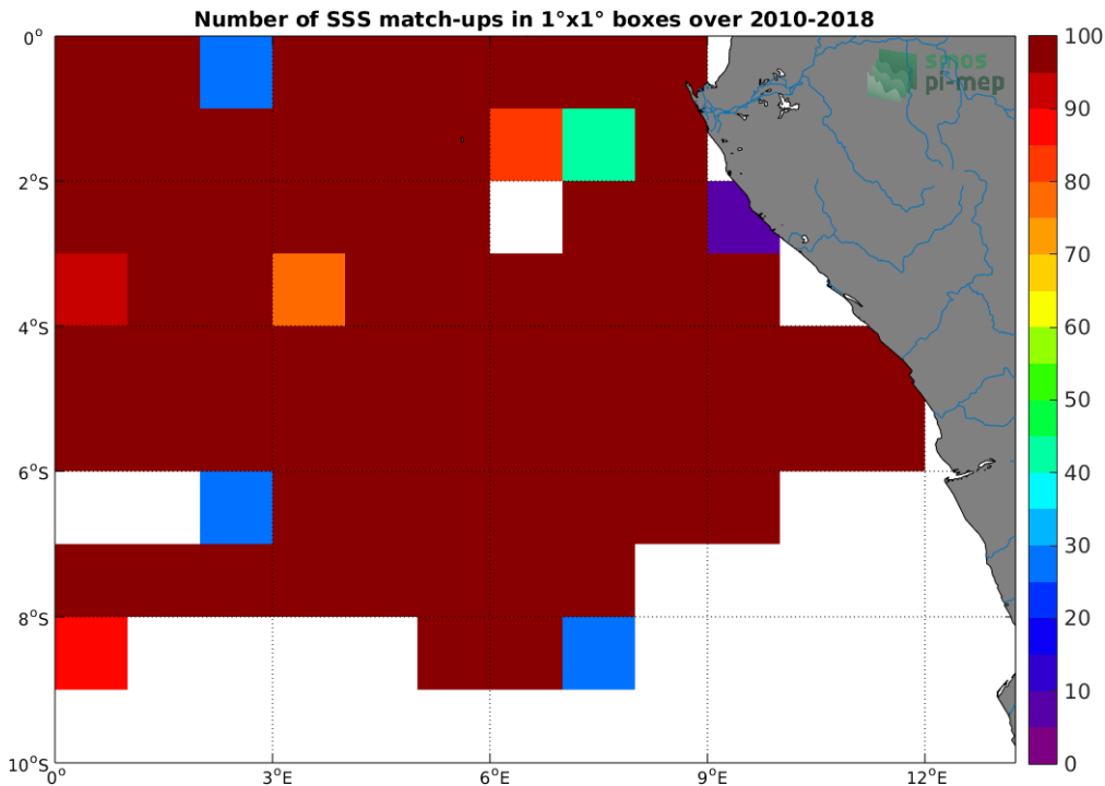
Figure 4: Number of SSS match-ups between TSG (GOSUD-Research-vessel) SSS and the CCI L4 Merged-OI v2.31 - 30-day running (ESA) SSS product for the Congo river plume Pi-MEP region over 1°x1° boxes and for the full satellite product period.
