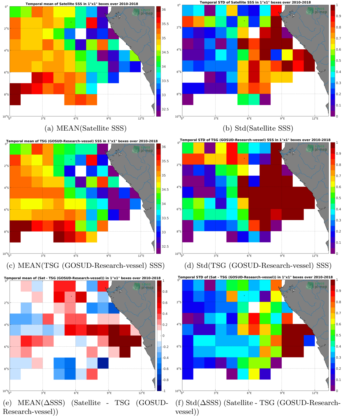
Figure 6: Temporal mean (left) and Std (right) of SSS from CCI L4 Merged-OI v2.31 - 30-day running (ESA) (top), TSG (GOSUD-Research-vessel) (middle), and of \Delta SSS (Satellite - TSG (GOSUD-Research-vessel)). Only match-up pairs are used to generate these maps.
