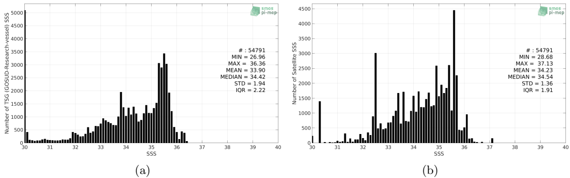
Figure 2: Histograms of SSS from TSG (GOSUD-Research-vessel) (a) and CCI L4 Merged-OI v2.31 - 30-day running (ESA) (b) considering all match-up pairs per bins of 0.1 over the Congo river plume Pi-MEP region and for the full satellite product period.
