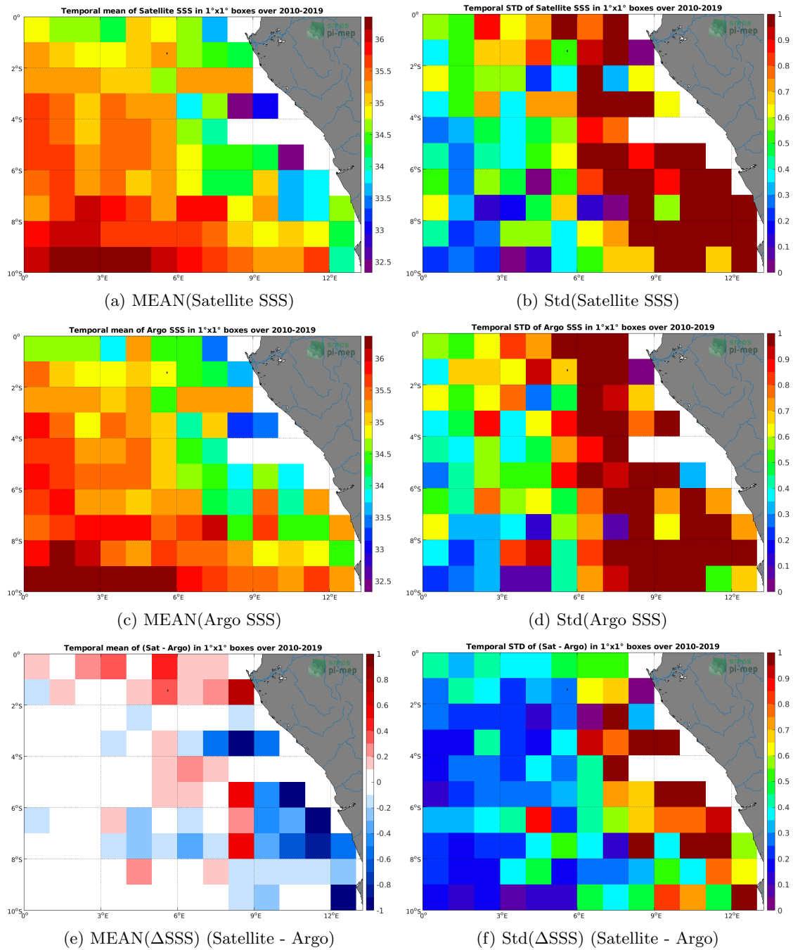
Figure 6: Temporal mean (left) and Std (right) of SSS from CCI SSS L4 Merged-OI v2.31 - 30-day running (ESA) (top), Argo (middle), and of \Delta SSS (Satellite - Argo). Only match-up pairs are used to generate these maps.
