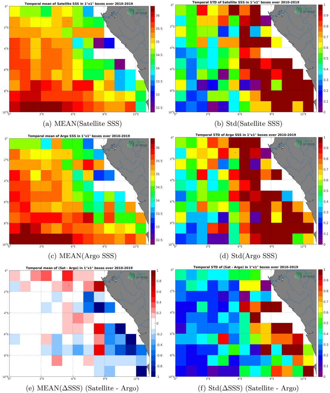
Figure 6: Temporal mean (left) and Std (right) of SSS from CCI L4 Merged-OI v2.31 - 30-day running (ESA) (top), Argo (middle), and of \Delta SSS (Satellite - Argo). Only match-up pairs are used to generate these maps.
