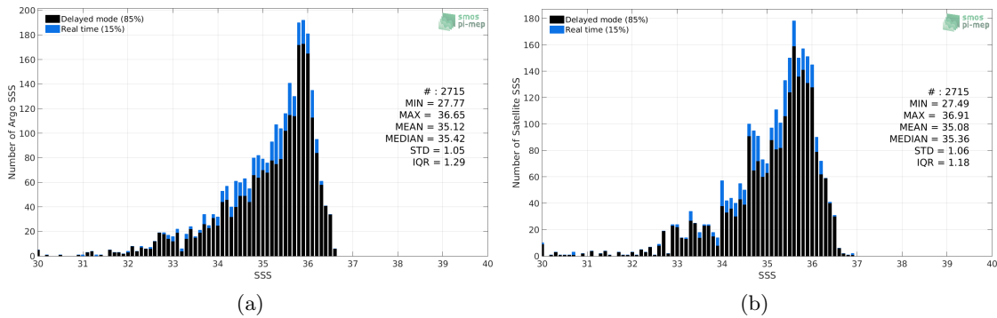
Figure 2: Histograms of SSS from Argo (a) and CCI L4 Merged-OI v2.31 - 30-day running (ESA) (b) considering all match-up pairs per bins of 0.1 over the Congo river plume Pi-MEP region and for the full satellite product period.
