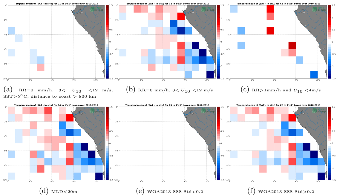
Figure 12: Temporal mean gridded over spatial boxes of size 1^\circ \times 1^\circ of \Delta SSS (CCI L4 Merged-OI v2.31 - 30-day running (ESA) - Argo) for 6 different subdatasets corresponding to:RR=0 mm/h, 3 < U_{10} < 12 m/s, SST >5^\circ\text{C} , distance to coast > 800 km (a), RR=0 mm/h, 3 < U_{10} < 12 m/s (b), RR >1 mm/h and U_{10} < 4 m/s (c),MLD <20 m (d),WOA2013 SSS Std <0.2 (e),WOA2013 SSS Std >0.2 (f).
