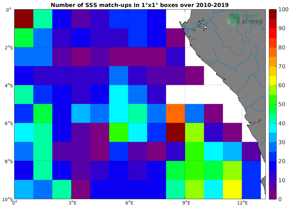
Figure 4: Number of SSS match-ups between Argo SSS and the CCI L4 Merged-OI v2.31 - 30-day running (ESA) SSS product for the Congo river plume Pi-MEP region over 1°x1° boxes and for the full satellite product period.
