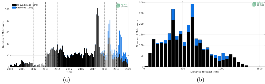
Figure 1: Number of match-ups between Argo and CCI L4 Merged-OI v2.31 - 30-day running (ESA) SSS as a function of time (a) and as function of the distance to coast (b) over the Congo river plume Pi-MEP region and for the full satellite product period.
