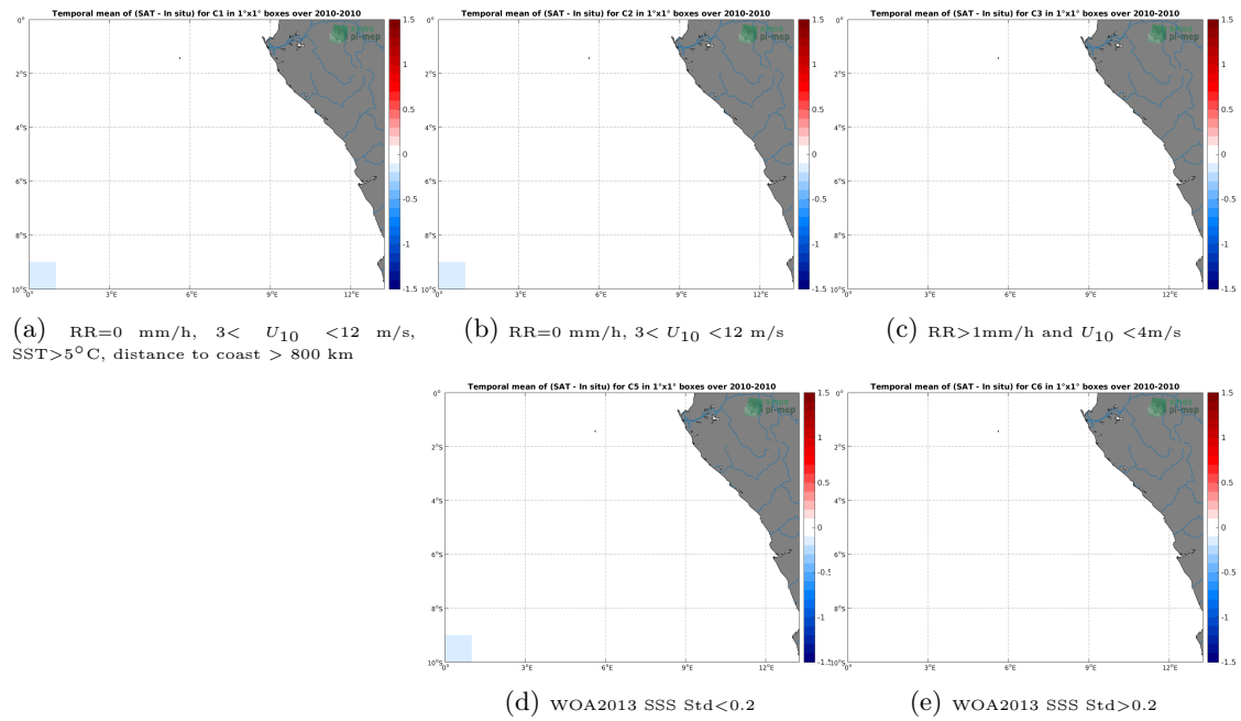
Figure 12: Temporal mean gridded over spatial boxes of size 1^\circ \times 1^\circ of \Delta SSS (CCI L4 Merged-OI v1.8 - 7-day running (ESA) - TSG-SAMOS) for 5 different subdatasets corresponding to:RR=0 mm/h, 3 < U_{10} < 12 m/s, SST > 5^\circ C , distance to coast > 800 km (a), RR=0 mm/h, 3 < U_{10} < 12 m/s (b), RR >1 mm/h and U_{10} < 4 m/s (c), WOA2013 SSS Std <0.2 (d), WOA2013 SSS Std >0.2 (e).
