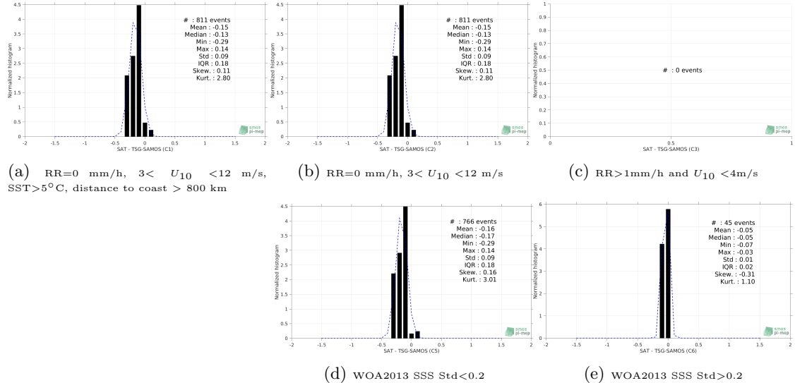
Figure 13: Normalized histogram of \Delta\text{SSS} (CCI L4 Merged-OI v1.8 - 7-day running (ESA) - TSG-SAMOS) for 5 different subdatasets corresponding to: RR=0 mm/h, 3 < U_{10} < 12 m/s, SST >5^{\circ}\text{C} , distance to coast > 800 km (a), RR=0 mm/h, 3 < U_{10} < 12 m/s (b), RR >1 mm/h and U_{10} < 4 m/s (c), WOA2013 SSS Std <0.2 (d), WOA2013 SSS Std >0.2 (e).
