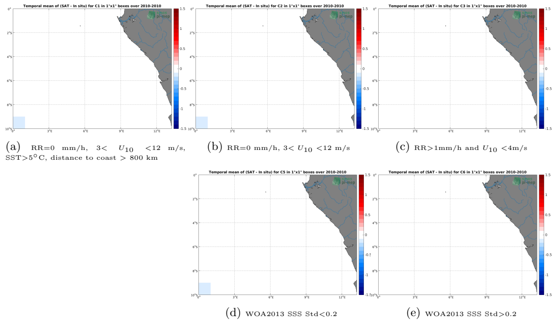
Figure 12: Temporal mean gridded over spatial boxes of size 1^\circ \times 1^\circ of \Delta SSS (CCI-L4-ESA-MERGED-OI-V1.8-7DAY-RUNNING - TSG-SAMOS) for 5 different subdatasets corresponding to:RR=0 mm/h, 3 < U_{10} < 12 m/s, SST > 5^\circ\text{C} , distance to coast > 800 km (a), RR=0 mm/h, 3 < U_{10} < 12 m/s (b), RR > 1 mm/h and U_{10} < 4 m/s (c), WOA2013 SSS Std < 0.2 (d), WOA2013 SSS Std > 0.2 (e).
