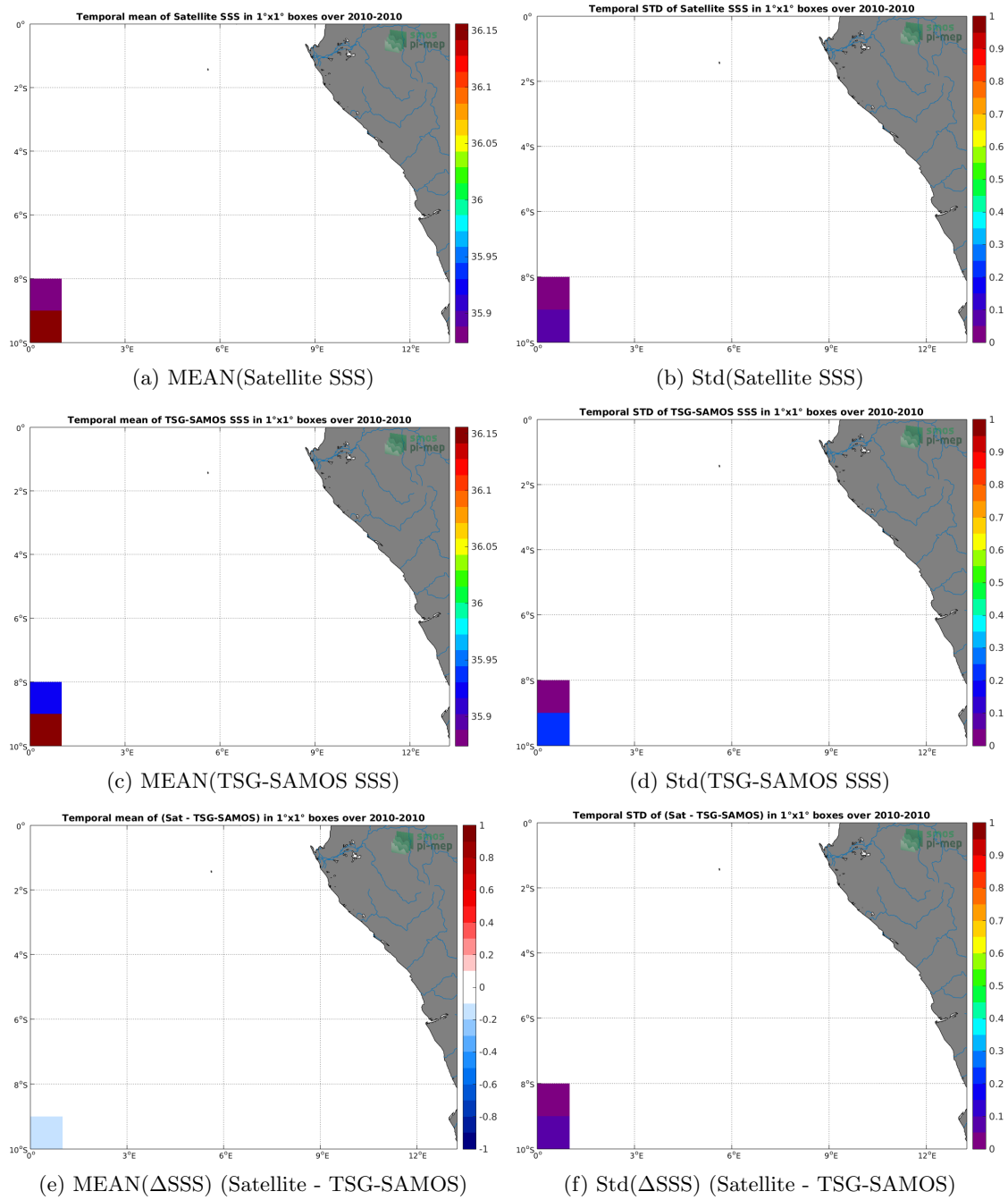
Figure 6: Temporal mean (left) and Std (right) of SSS from CCI-L4-ESA-MERGED-OI-V1.8-7DAY-RUNNING (top), TSG-SAMOS (middle), and of \Delta SSS (Satellite - TSG-SAMOS). Only match-up pairs are used to generate these maps.
