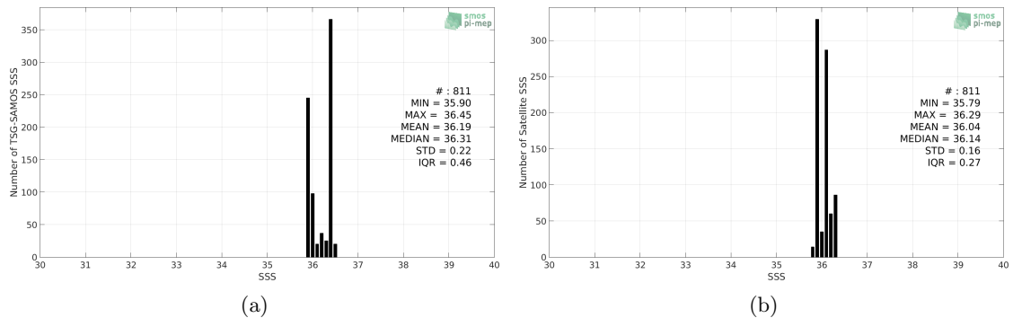
Figure 2: Histograms of SSS from TSG-SAMOS (a) and CCI-L4-ESA-MERGED-OI-V1.8-7DAY-RUNNING (b) considering all match-up pairs per bins of 0.1 over the Congo river plume Pi-MEP region and for the full satellite product period.
