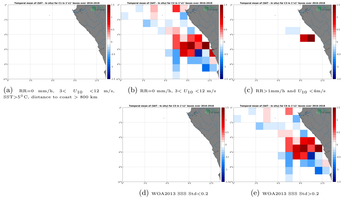
Figure 12: Temporal mean gridded over spatial boxes of size 1^\circ \times 1^\circ of \Delta SSS (CCI L4 Merged-OI v1.8 - 7-day running (ESA) - TSG-LEGOS-DM) for 5 different subdatasets corresponding to:RR=0 mm/h, 3 < U_{10} < 12 m/s, SST > 5^\circ\text{C} , distance to coast > 800 km (a), RR=0 mm/h, 3 < U_{10} < 12 m/s (b), RR > 1 mm/h and U_{10} < 4 m/s (c), WOA2013 SSS Std < 0.2 (d), WOA2013 SSS Std > 0.2 (e).
