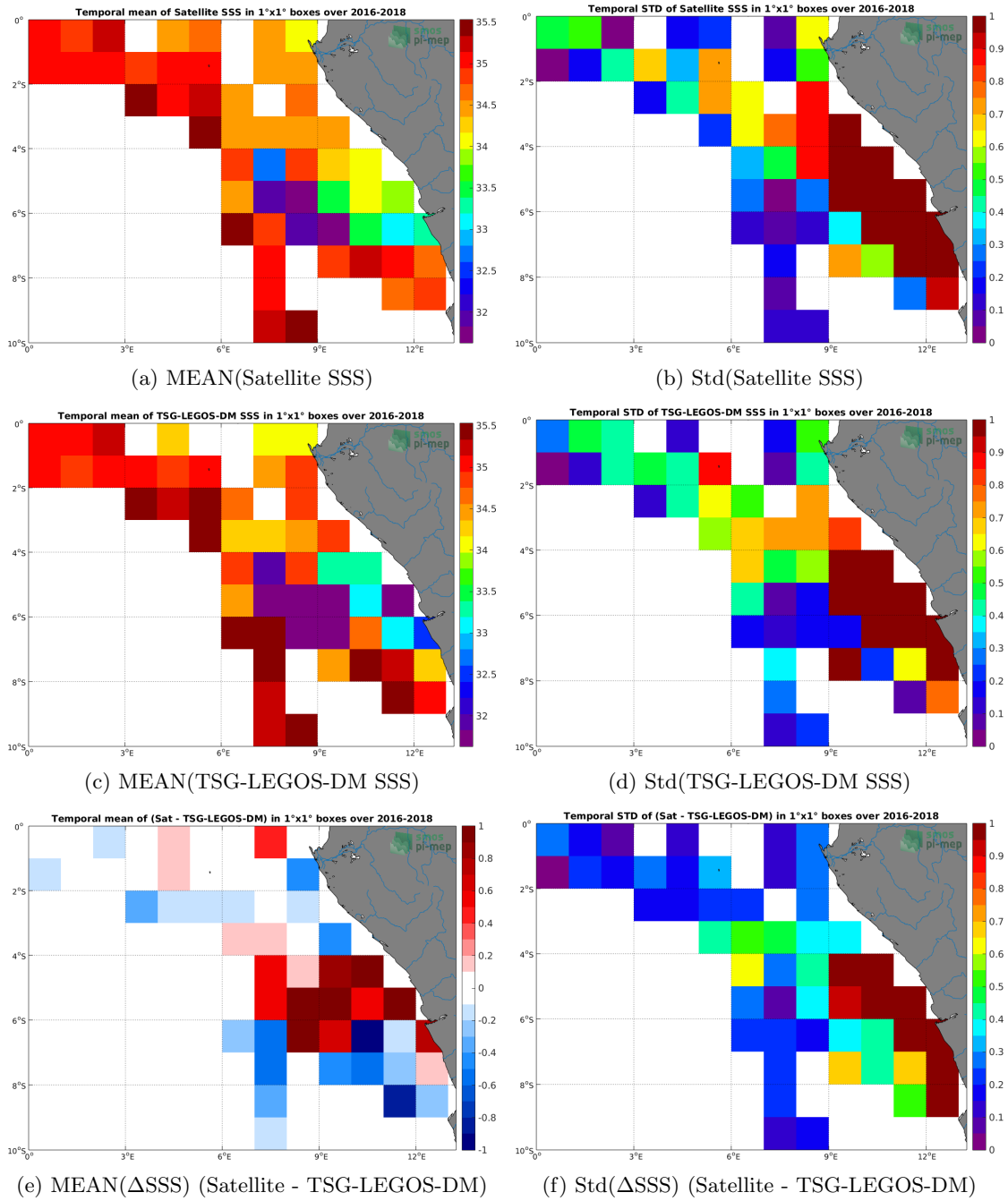
Figure 6: Temporal mean (left) and Std (right) of SSS from CCI L4 Merged-OI v1.8 - 7-day running (ESA) (top), TSG-LEGOS-DM (middle), and of \Delta SSS (Satellite - TSG-LEGOS-DM). Only match-up pairs are used to generate these maps.
