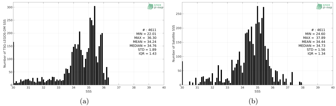
Figure 2: Histograms of SSS from TSG-LEGOS-DM (a) and CCI L4 Merged-OI v1.8 - 7-day running (ESA) (b) considering all match-up pairs per bins of 0.1 over the Congo river plume Pi-MEP region and for the full satellite product period.
