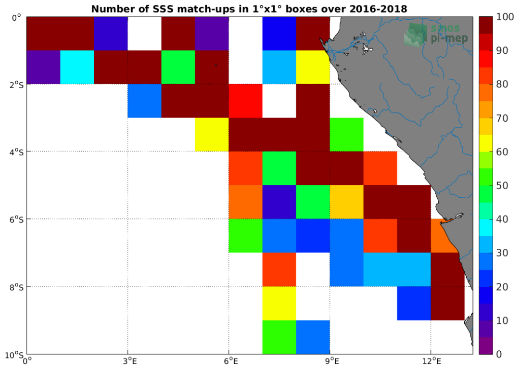
Figure 4: Number of SSS match-ups between TSG-LEGOS-DM SSS and the CCI L4 Merged-OI v1.8 - 7-day running (ESA) SSS product for the Congo river plume Pi-MEP region over 1°x1° boxes and for the full satellite product period.
