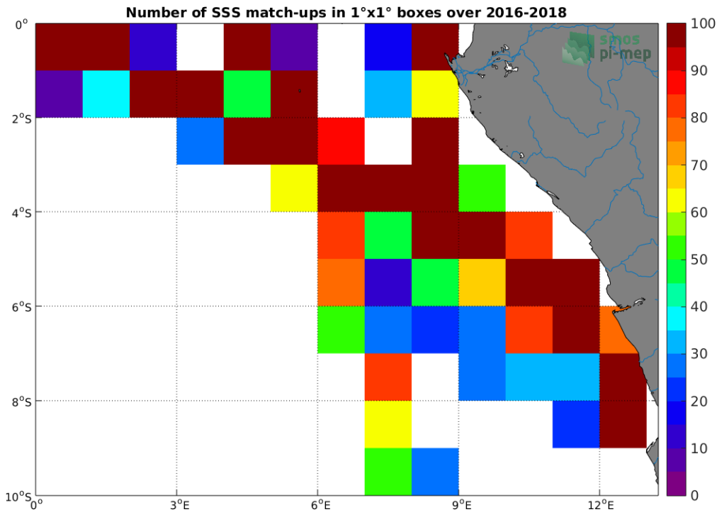
Figure 4: Number of SSS match-ups between TSG-LEGOS-DM SSS and the CCI-L4-ESA-MERGED-OI-V1.8-7DAY-RUNNING SSS product for the Congo river plume Pi-MEP region over 1°x1° boxes and for the full satellite product period.
