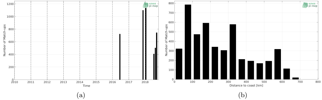
Figure 1: Number of match-ups between TSG-LEGOS-DM and CCI-L4-ESA-MERGED-OI-V1.8-7DAY-RUNNING SSS as a function of time (a) and as function of the distance to coast (b) over the Congo river plume Pi-MEP region and for the full satellite product period.
