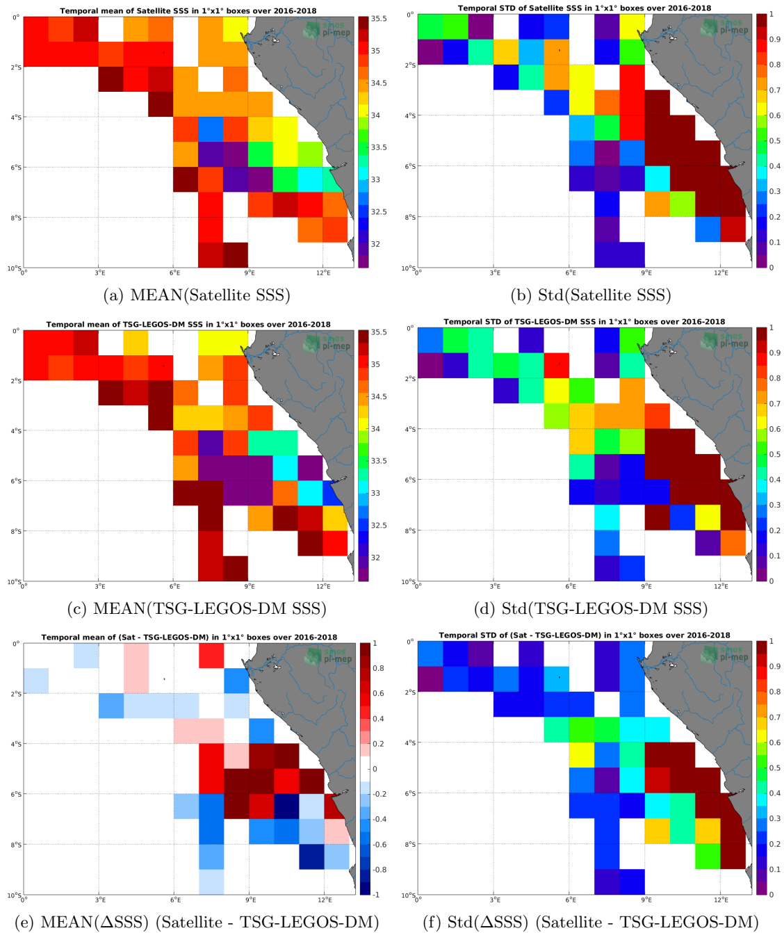
Figure 6: Temporal mean (left) and Std (right) of SSS from CCI-L4-ESA-MERGED-OI-V1.8-7DAY-RUNNING (top), TSG-LEGOS-DM (middle), and of \Delta SSS (Satellite - TSG-LEGOS-DM). Only match-up pairs are used to generate these maps.
