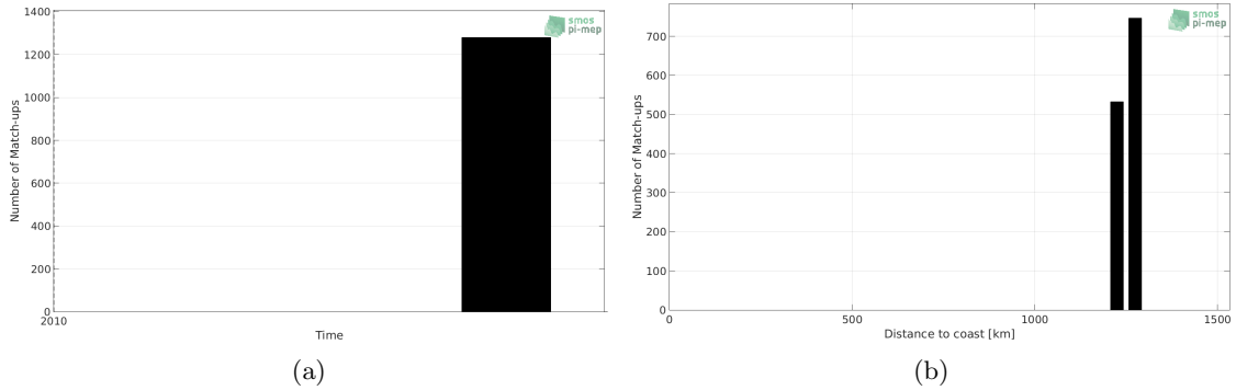
Figure 1: Number of match-ups between TSG-SAMOS and CCI L4 Merged-OI v1.8 - 30-day running (ESA) SSS as a function of time (a) and as function of the distance to coast (b) over the Congo river plume Pi-MEP region and for the full satellite product period.
