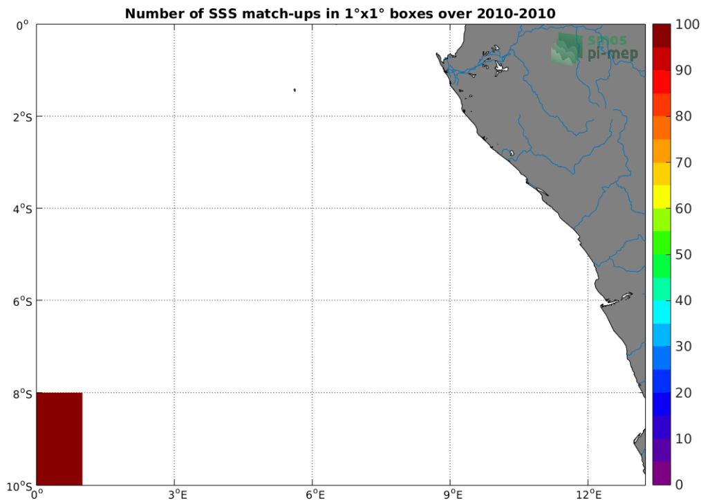
Figure 4: Number of SSS match-ups between TSG-SAMOS SSS and the CCI L4 Merged-OI v1.8 - 30-day running (ESA) SSS product for the Congo river plume Pi-MEP region over 1^\circ \times 1^\circ boxes and for the full satellite product period.
