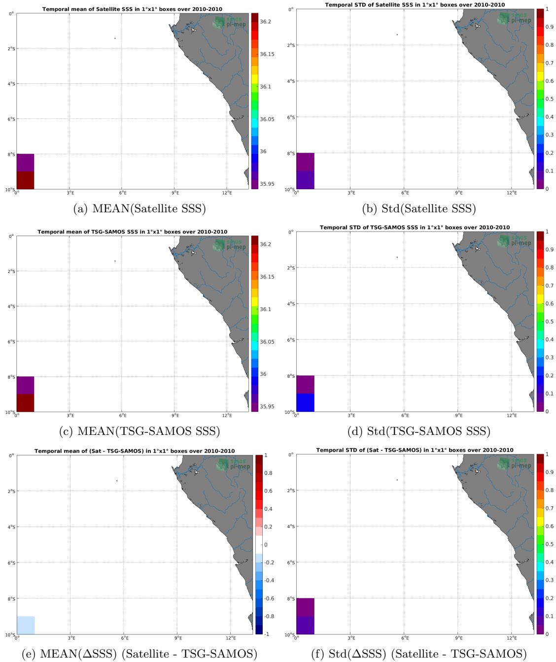
Figure 6: Temporal mean (left) and Std (right) of SSS from CCI L4 Merged-OI v1.8 - 30-day running (ESA) (top), TSG-SAMOS (middle), and of \Delta SSS (Satellite - TSG-SAMOS). Only match-up pairs are used to generate these maps.
