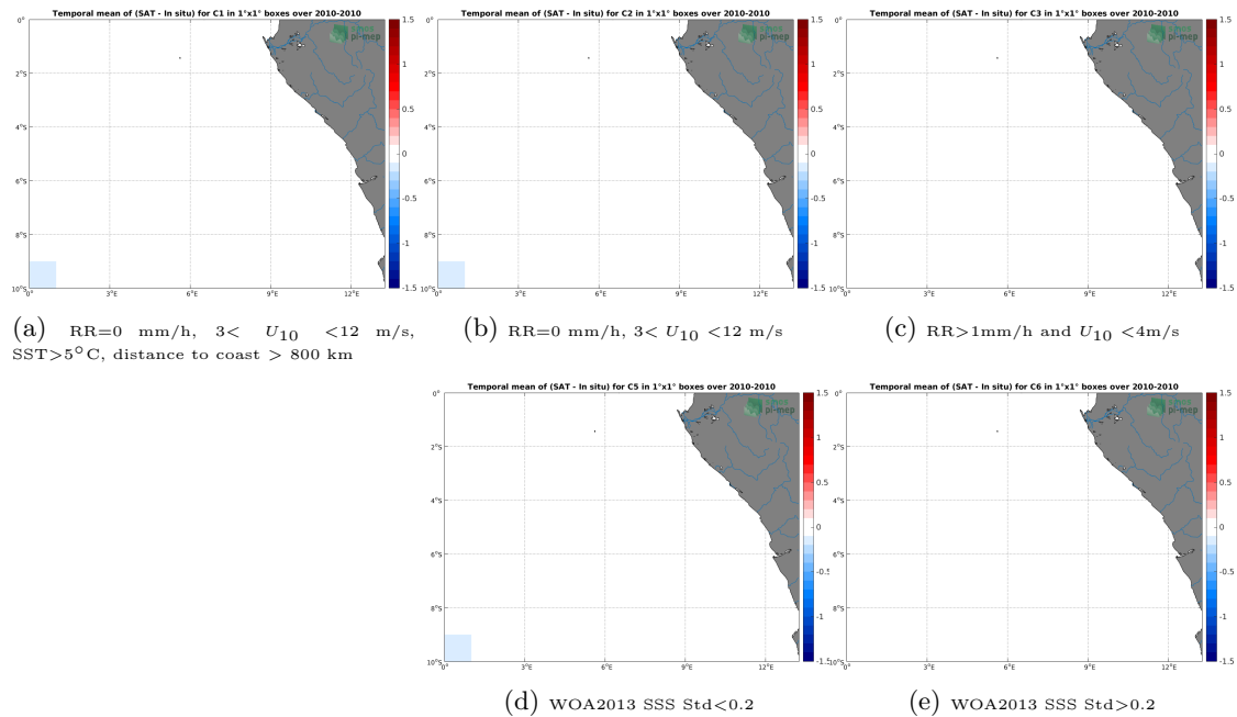
Figure 12: Temporal mean gridded over spatial boxes of size 1^\circ \times 1^\circ of \Delta SSS (CCI L4 Merged-OI v1.8 - 30-day running (ESA) - TSG-SAMOS) for 5 different subdatasets corresponding to:RR=0 mm/h, 3 < U_{10} < 12 m/s, SST > 5^\circ\text{C} , distance to coast > 800 km (a), RR=0 mm/h, 3 < U_{10} < 12 m/s (b), RR > 1 mm/h and U_{10} < 4 m/s (c), WOA2013 SSS Std < 0.2 (d), WOA2013 SSS Std > 0.2 (e).
