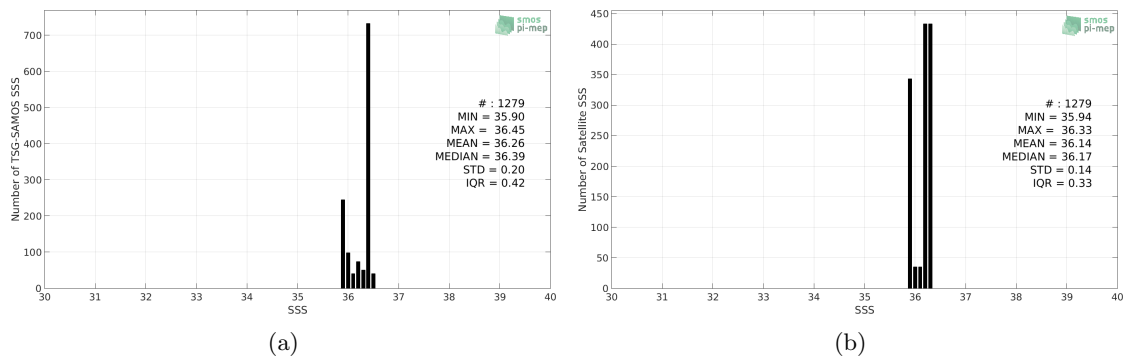
Figure 2: Histograms of SSS from TSG-SAMOS (a) and CCI-L4-ESA-MERGED-OI-V1.8-30DAY-RUNNING (b) considering all match-up pairs per bins of 0.1 over the Congo river plume Pi-MEP region and for the full satellite product period.
