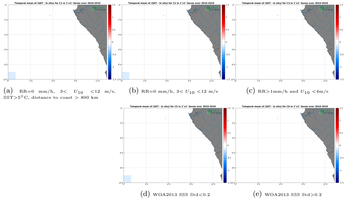
Figure 12: Temporal mean gridded over spatial boxes of size 1^\circ \times 1^\circ of \Delta SSS (CCI-L4-ESA-MERGED-OI-V1.8-30DAY-RUNNING - TSG-SAMOS) for 5 different subdatasets corresponding to:RR=0 mm/h, 3 < U_{10} < 12 m/s, SST > 5^\circ\text{C} , distance to coast > 800 km (a), RR=0 mm/h, 3 < U_{10} < 12 m/s (b), RR > 1 mm/h and U_{10} < 4 m/s (c), WOA2013 SSS Std < 0.2 (d), WOA2013 SSS Std > 0.2 (e).
