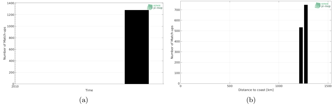
Figure 1: Number of match-ups between TSG-SAMOS and CCI-L4-ESA-MERGED-OI-V1.8-30DAY-RUNNING SSS as a function of time (a) and as function of the distance to coast (b) over the Congo river plume Pi-MEP region and for the full satellite product period.
