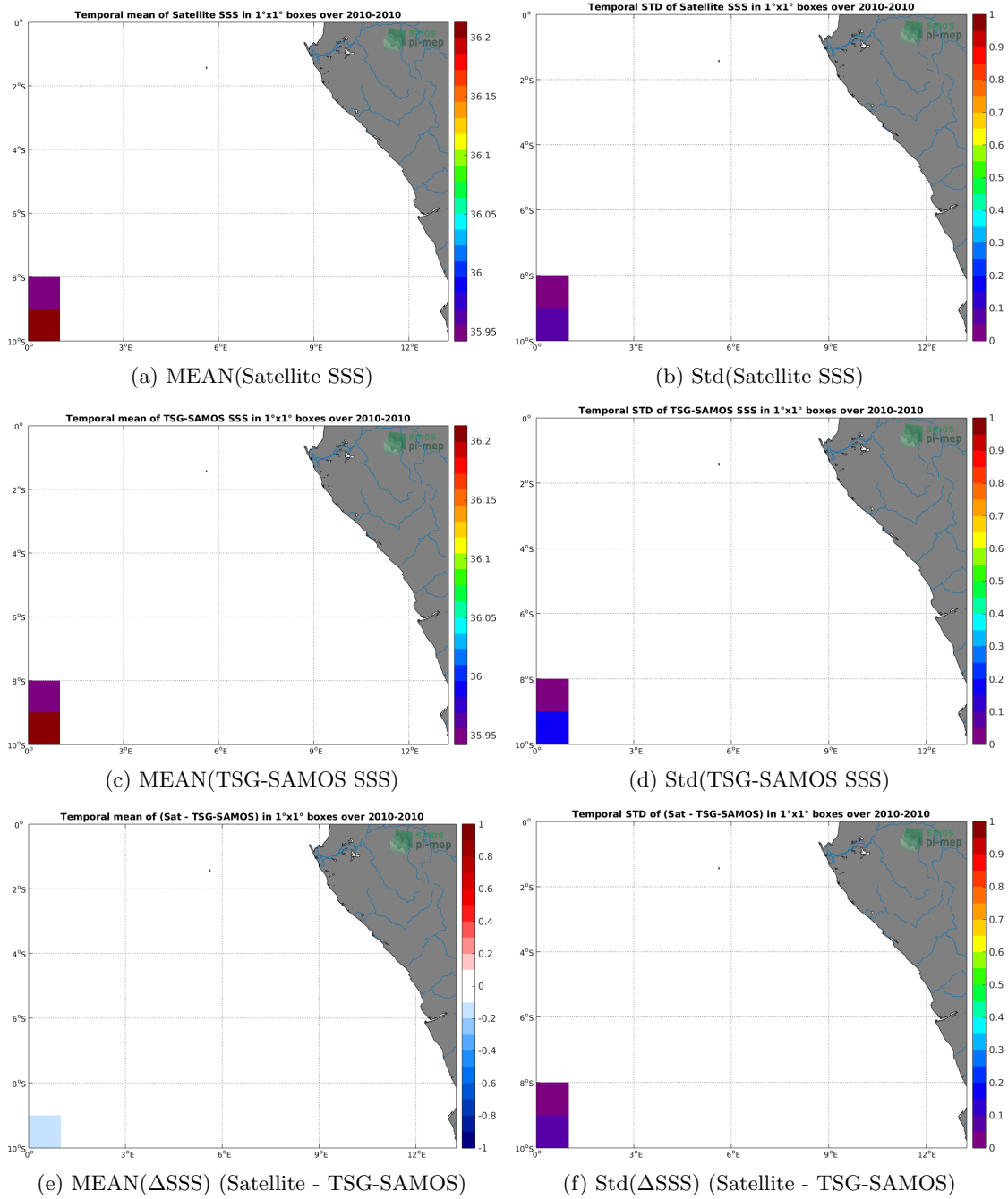
Figure 6: Temporal mean (left) and Std (right) of SSS from CCI-L4-ESA-MERGED-OI-V1.8-30DAY-RUNNING (top), TSG-SAMOS (middle), and of \Delta SSS (Satellite - TSG-SAMOS). Only match-up pairs are used to generate these maps.
