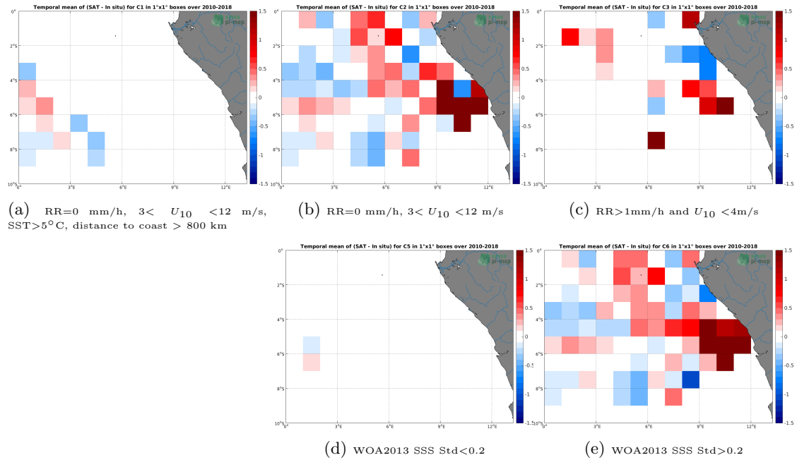
Figure 12: Temporal mean gridded over spatial boxes of size 1^\circ \times 1^\circ of \Delta SSS (CCI-L4-ESA-MERGED-OI-V1.8-30DAY-RUNNING - TSG-GOSUD-Research-vessel) for 5 different sub-datasets corresponding to: RR=0 mm/h, 3 < U_{10} < 12 m/s, SST >5^\circ\text{C} , distance to coast > 800 km (a), RR=0 mm/h, 3 < U_{10} < 12 m/s (b), RR >1 mm/h and U_{10} < 4 m/s (c), WOA2013 SSS Std <0.2 (d), WOA2013 SSS Std >0.2 (e).
