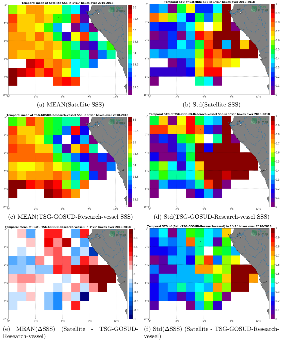
Figure 6: Temporal mean (left) and Std (right) of SSS from CCI-L4-ESA-MERGED-OI-V1.8-30DAY-RUNNING (top), TSG-GOSUD-Research-vessel (middle), and of \Delta SSS (Satellite - TSG-GOSUD-Research-vessel). Only match-up pairs are used to generate these maps.
