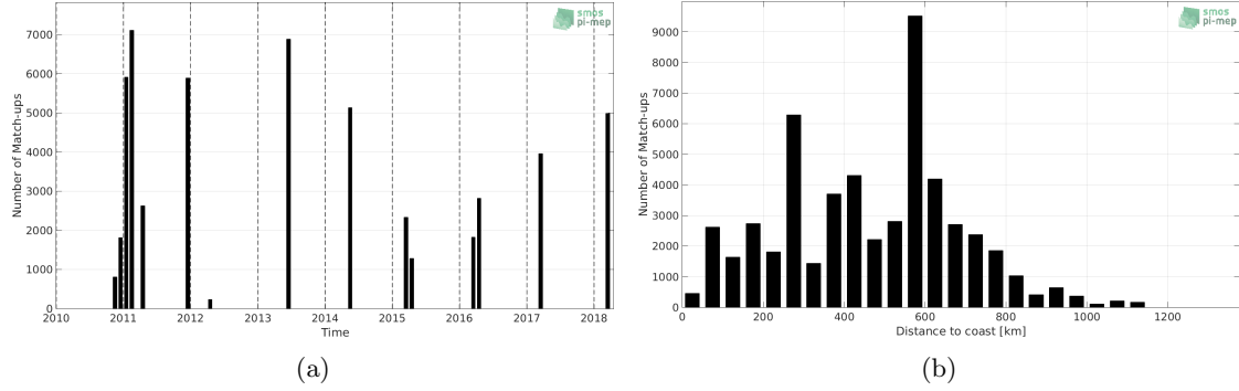
Figure 1: Number of match-ups between TSG-GOSUD-Research-vessel and CCI-L4-ESA-MERGED-OI-V1.8-30DAY-RUNNING SSS as a function of time (a) and as function of the distance to coast (b) over the Congo river plume Pi-MEP region and for the full satellite product period.
