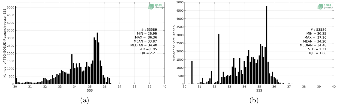
Figure 2: Histograms of SSS from TSG-GOSUD-Research-vessel (a) and CCI-L4-ESA-MERGED-OI-V1.8-30DAY-RUNNING (b) considering all match-up pairs per bins of 0.1 over the Congo river plume Pi-MEP region and for the full satellite product period.
