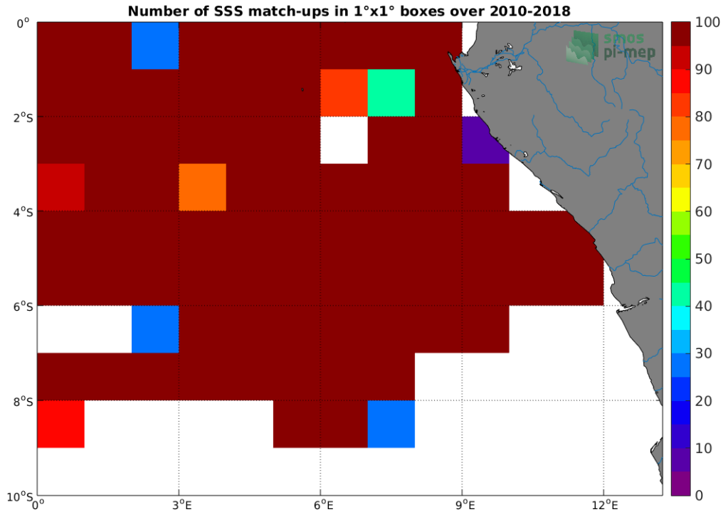
Figure 4: Number of SSS match-ups between TSG-GOSUD-Research-vessel SSS and the CCI-L4-ESA-MERGED-OI-V1.8-30DAY-RUNNING SSS product for the Congo river plume Pi-MEP region over 1^\circ \times 1^\circ boxes and for the full satellite product period.
