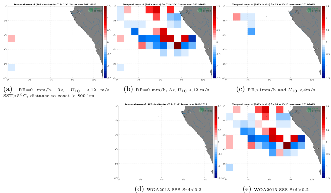
Figure 12: Temporal mean gridded over spatial boxes of size 1^\circ \times 1^\circ of \Delta SSS (Aquarius SSS L4 OI v5 - Weekly (IPRC) - TSG (GOSUD-Research-vessel)) for 5 different subdatasets corresponding to:RR=0 mm/h, 3 < U_{10} < 12 m/s, SST>5°C, distance to coast > 800 km (a), RR=0 mm/h, 3 < U_{10} < 12 m/s (b), RR>1mm/h and U_{10} < 4 m/s (c), WOA2013 SSS Std<0.2 (d), WOA2013 SSS Std>0.2 (e).
