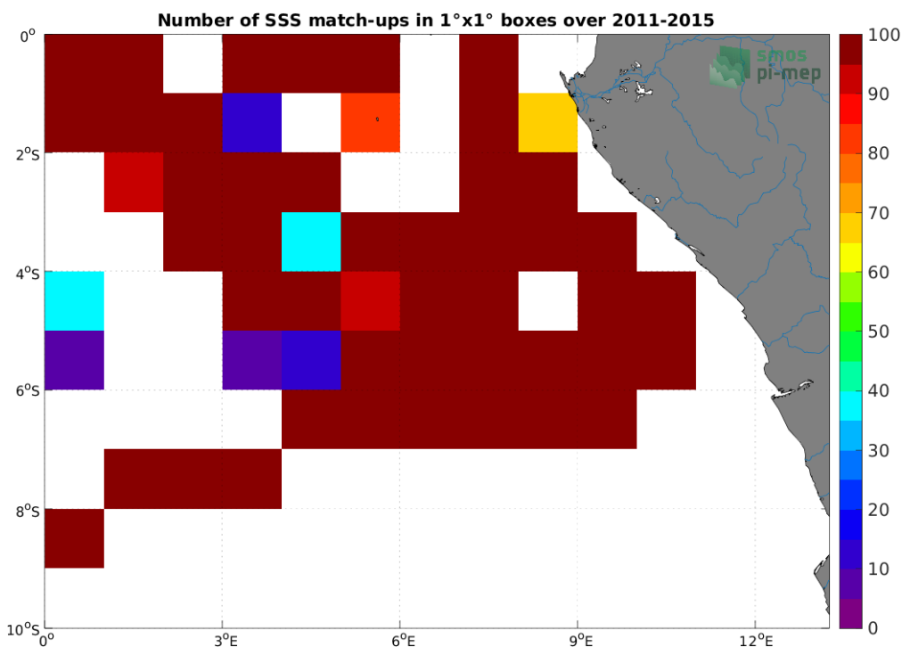
Figure 4: Number of SSS match-ups between TSG (GOSUD-Research-vessel) SSS and the Aquarius SSS L4 OI v5 - Weekly (IPRC) SSS product for the Congo river plume Pi-MEP region over 1^\circ \times 1^\circ boxes and for the full satellite product period.
