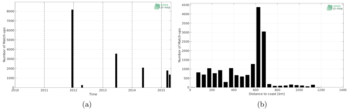
Figure 1: Number of match-ups between TSG-GOSUD-Research-vessel and Aquarius-L4-IPRC-V5-WEEKLY SSS as a function of time (a) and as function of the distance to coast (b) over the Congo river plume Pi-MEP region and for the full satellite product period.
