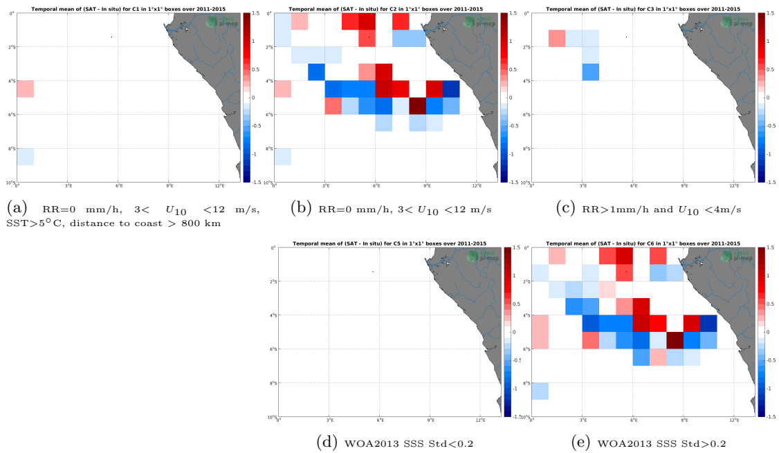
Figure 12: Temporal mean gridded over spatial boxes of size 1^\circ \times 1^\circ of \Delta SSS (Aquarius-L4-IPRC-V5-WEEKLY - TSG-GOSUD-Research-vessel) for 5 different subdatasets corresponding to: RR=0 mm/h, 3 < U_{10} < 12 m/s, SST > 5°C, distance to coast > 800 km (a), RR=0 mm/h, 3 < U_{10} < 12 m/s (b), RR > 1mm/h and U_{10} < 4 m/s (c), WOA2013 SSS Std < 0.2 (d), WOA2013 SSS Std > 0.2 (e).
