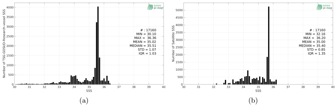
Figure 2: Histograms of SSS from TSG-GOSUD-Research-vessel (a) and Aquarius-L4-IPRC-V5-WEEKLY (b) considering all match-up pairs per bins of 0.1 over the Congo river plume Pi-MEP region and for the full satellite product period.
