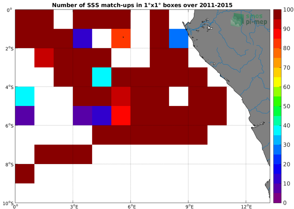
Figure 4: Number of SSS match-ups between TSG-GOSUD-Research-vessel SSS and the Aquarius-L4-IPRC-V5-WEEKLY SSS product for the Congo river plume Pi-MEP region over 1°x1° boxes and for the full satellite product period.
