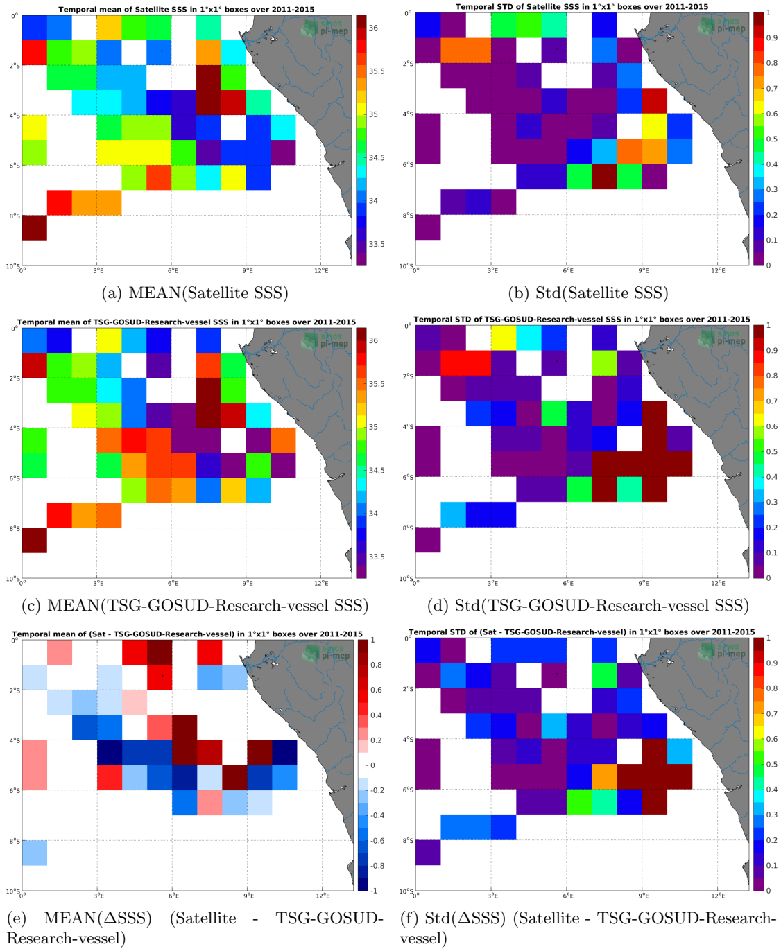
Figure 6: Temporal mean (left) and Std (right) of SSS from Aquarius-L4-IPRC-V5-WEEKLY (top), TSG-GOSUD-Research-vessel (middle), and of \Delta SSS (Satellite - TSG-GOSUD-Research-vessel). Only match-up pairs are used to generate these maps.
