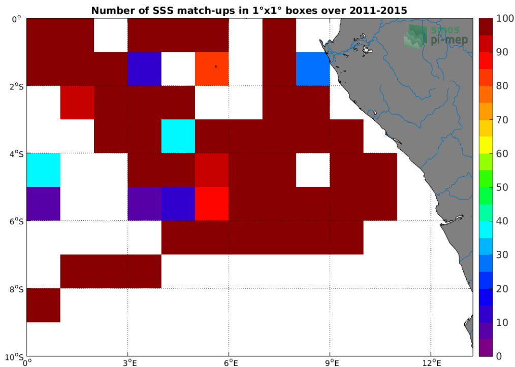
Figure 4: Number of SSS match-ups between TSG-GOSUD-Research-vessel SSS and the Aquarius-L4-IPRC-V5-WEEKLY SSS product for the Congo river plume Pi-MEP region over 1^\circ \times 1^\circ boxes and for the full satellite product period.
