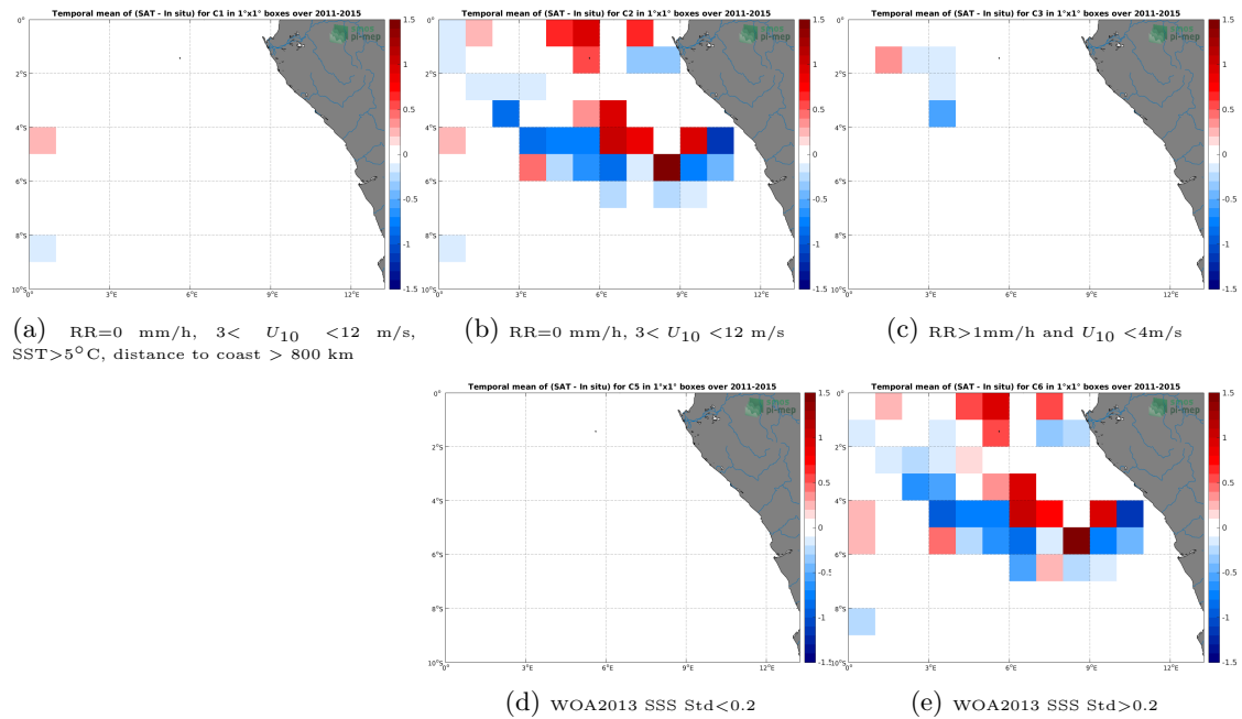
Figure 12: Temporal mean gridded over spatial boxes of size 1^\circ \times 1^\circ of \Delta SSS (Aquarius-L4-IPRC-V5-WEEKLY - TSG-GOSUD-Research-vessel) for 5 different subdatasets corresponding to:RR=0 mm/h, 3 < U_{10} < 12 m/s, SST >5^\circ C, distance to coast > 800 km (a), RR=0 mm/h, 3 < U_{10} < 12 m/s (b), RR >1 mm/h and U_{10} < 4 m/s (c), WOA2013 SSS Std <0.2 (d), WOA2013 SSS Std >0.2 (e).
