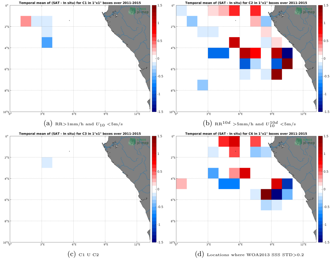
Figure 12: Temporal mean gridded over spatial boxes of size 1^\circ \times 1^\circ of \Delta SSS (Aquarius-L4-IPRC-V5-WEEKLY - TSG-GOSUD-Research-vessel) for 4 different subdatasets corresponding to: RR > 1\text{mm/h} and U_{10} < 5\text{m/s} (a), RR^{10d} > 5\text{mm/h} and U_{10}^{10d} < 5\text{m/s} (b), C1 \cup C2 (c), Locations where WOA2013 SSS STD > 0.2 (d).
