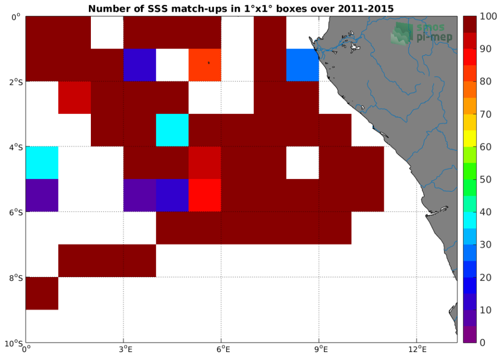
Figure 4: Number of SSS match-ups between TSG-GOSUD-Research-vessel SSS and the Aquarius-L4-IPRC-V5-WEEKLY SSS product for the Congo river plume Pi-MEP region over 1^{\circ} \times 1^{\circ} boxes and for the full satellite product period.
