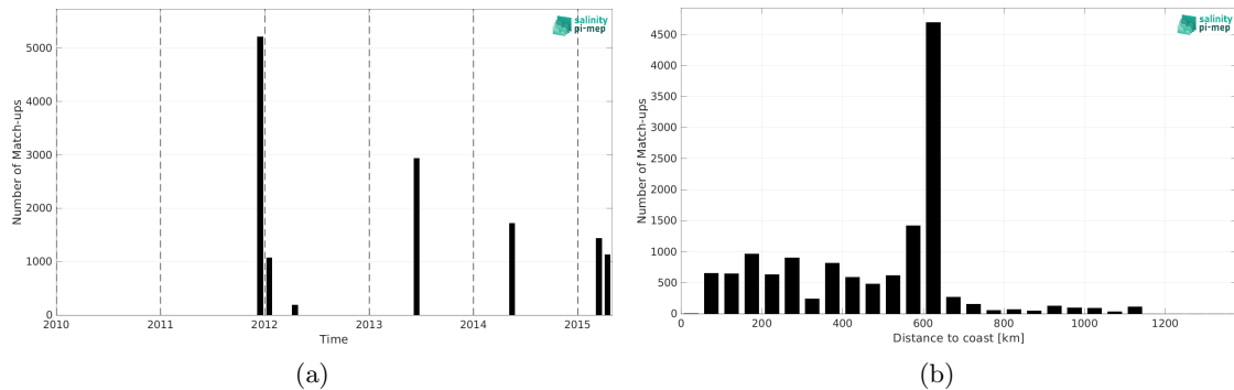
Figure 2: Number of match-ups between TSG (GOSUD-Research-vessel) and Aquarius SSS L4 OI v5 - Monthly (IPRC) SSS as a function of time (a) and as function of the distance to coast (b) over the Congo river plume Pi-MEP region and for the full satellite product period.
