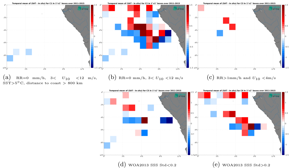
Figure 14: Temporal mean gridded over spatial boxes of size 1^\circ \times 1^\circ of \Delta SSS (Aquarius SSS L4 OI v5 - Monthly (IPRC) - TSG (GOSUD-Research-vessel)) for 5 different subdatasets corresponding to:RR=0 mm/h, 3 < U_{10} < 12 m/s, SST>5°C, distance to coast > 800 km (a), RR=0 mm/h, 3 < U_{10} < 12 m/s (b), RR>1mm/h and U_{10} < 4 m/s (c), WOA2013 SSS Std<0.2 (d), WOA2013 SSS Std>0.2 (e).
