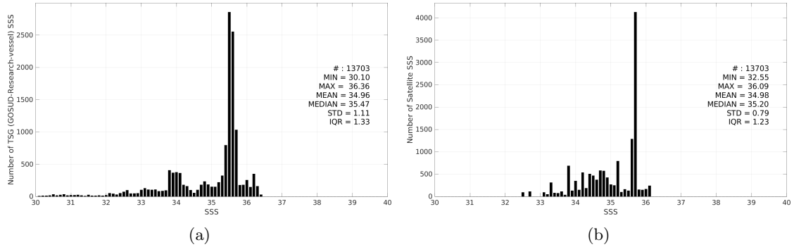
Figure 3: Histograms of SSS from TSG (GOSUD-Research-vessel) (a) and Aquarius SSS L4 OI v5 - Monthly (IPRC) (b) considering all match-up pairs per bins of 0.1 over the Congo river plume Pi-MEP region and for the full satellite product period.
