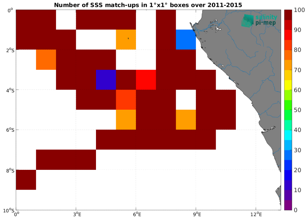
Figure 5: Number of SSS match-ups between TSG (GOSUD-Research-vessel) SSS and the Aquarius SSS L4 OI v5 - Monthly (IPRC) SSS product for the Congo river plume Pi-MEP region over 1^\circ \times 1^\circ boxes and for the full satellite product period.
