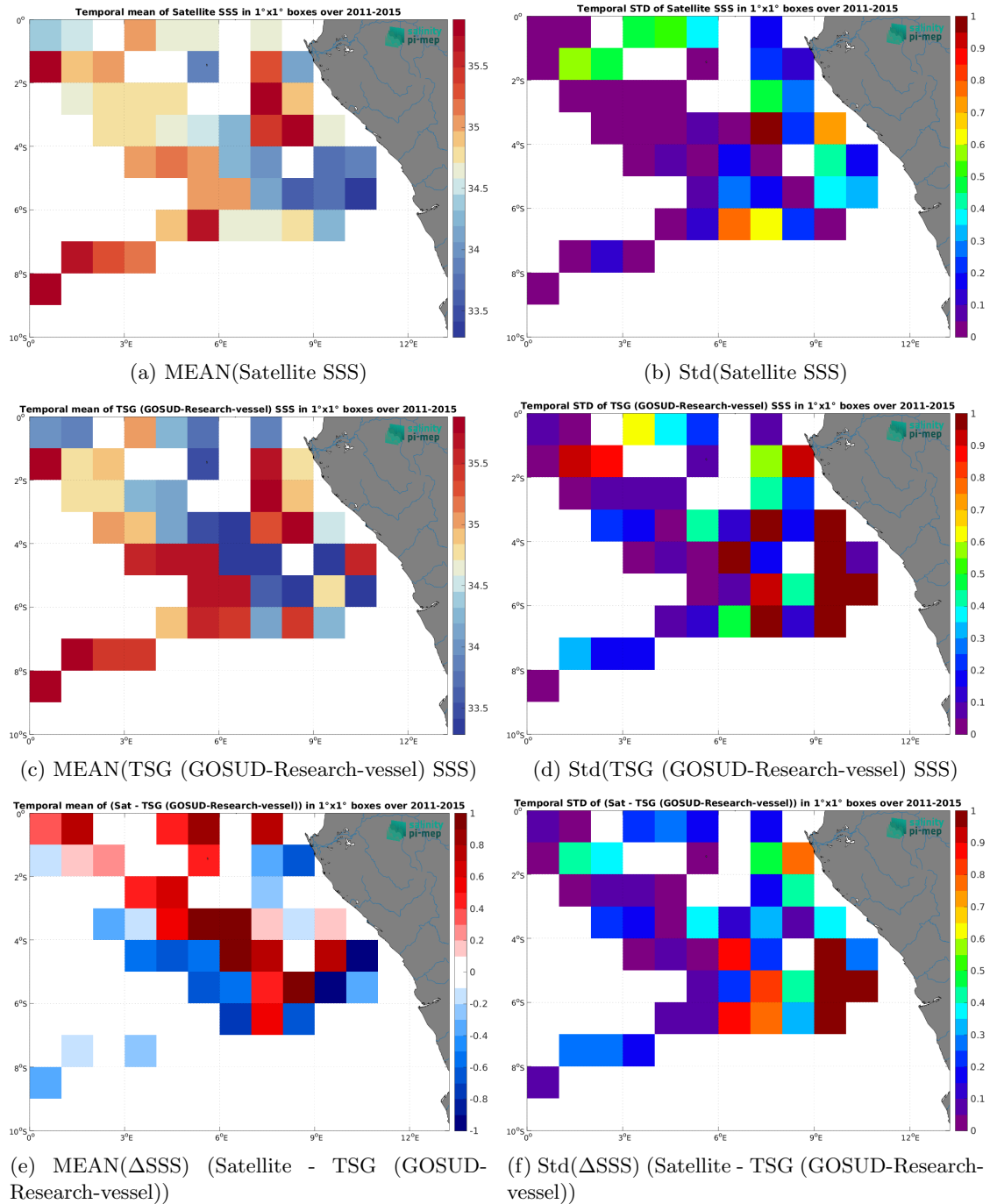
Figure 7: Temporal mean (left) and Std (right) of SSS from Aquarius SSS L4 OI v5 - Monthly (IPRC) (top), TSG (GOSUD-Research-vessel) (middle), and of \Delta SSS (Satellite - TSG (GOSUD-Research-vessel)). Only match-up pairs are used to generate these maps.
