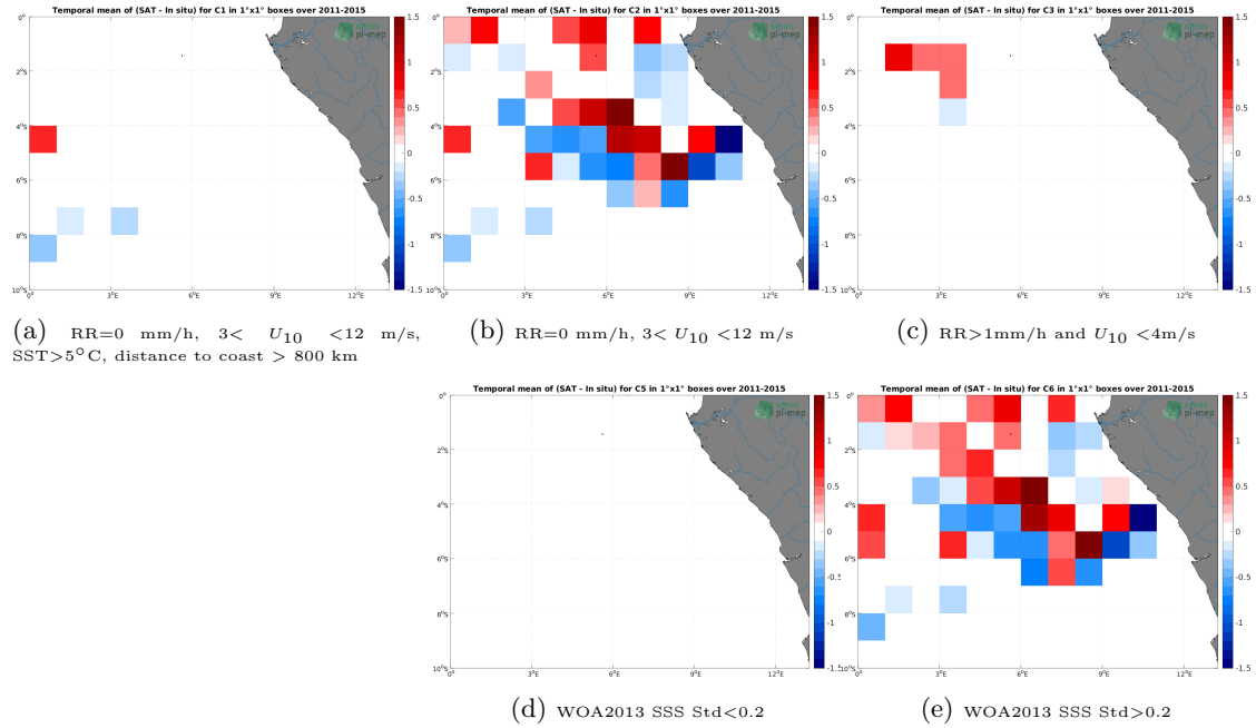
Figure 12: Temporal mean gridded over spatial boxes of size 1^{\circ}\times 1^{\circ} of \Delta SSS (Aquarius SSS L4 OI v5 - Monthly (IPRC) - TSG (GOSUD-Research-vessel)) for 5 different subdatasets corresponding to:RR=0 mm/h, 3 < U_{10} < 12 m/s, SST >5^{\circ}\text{C} , distance to coast > 800 km (a), RR=0 mm/h, 3 < U_{10} < 12 m/s (b), RR >1 mm/h and U_{10} < 4 m/s (c), WOA2013 SSS Std <0.2 (d), WOA2013 SSS Std >0.2 (e).
