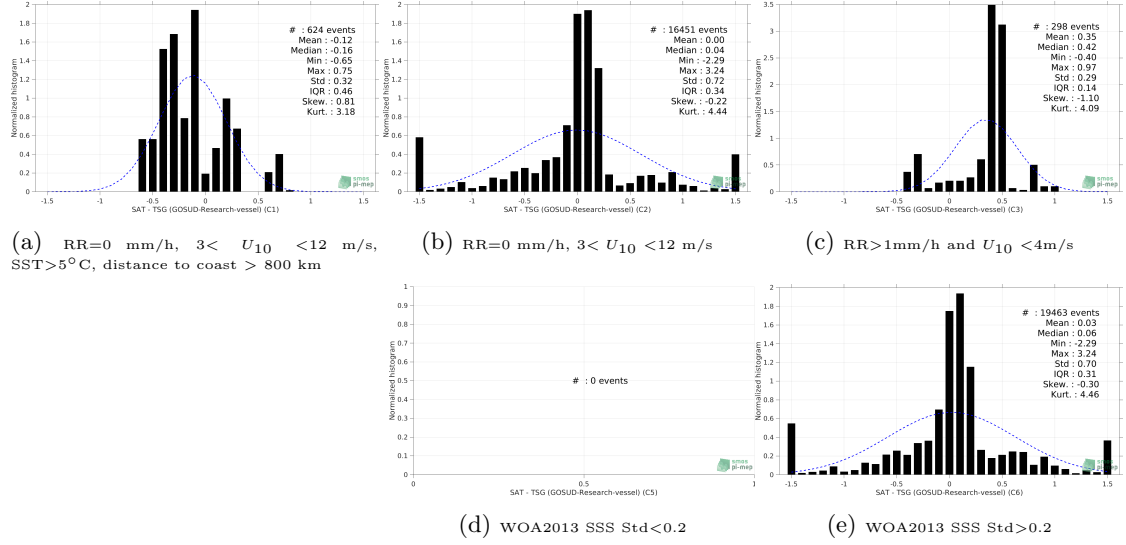
Figure 13: Normalized histogram of \Delta SSS (Aquarius SSS L4 OI v5 - Monthly (IPRC) - TSG (GOSUD-Research-vessel)) for 5 different subdatasets corresponding to: RR=0 mm/h, 3 < U_{10} < 12 m/s, SST > 5°C, distance to coast > 800 km (a), RR=0 mm/h, 3 < U_{10} < 12 m/s (b), RR > 1mm/h and U_{10} < 4 m/s (c), WOA2013 SSS Std < 0.2 (d), WOA2013 SSS Std > 0.2 (e).
