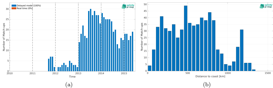
Figure 2: Number of match-ups between Argo and Aquarius SSS L4 OI v5 - Monthly (IPRC) SSS as a function of time (a) and as function of the distance to coast (b) over the Congo river plume Pi-MEP region and for the full satellite product period.
