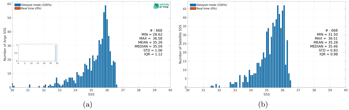
Figure 3: Histograms of SSS from Argo (a) and Aquarius SSS L4 OI v5 - Monthly (IPRC) (b) considering all match-up pairs per bins of 0.1 over the Congo river plume Pi-MEP region and for the full satellite product period.
