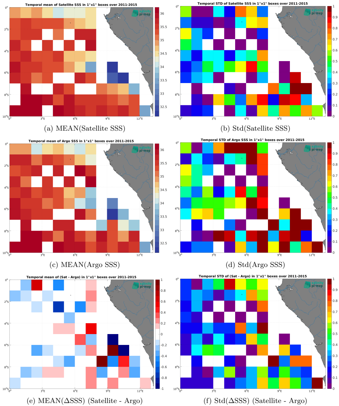
Figure 7: Temporal mean (left) and Std (right) of SSS from Aquarius SSS L4 OI v5 - Monthly (IPRC) (top), Argo (middle), and of \Delta SSS (Satellite - Argo). Only match-up pairs are used to generate these maps.
