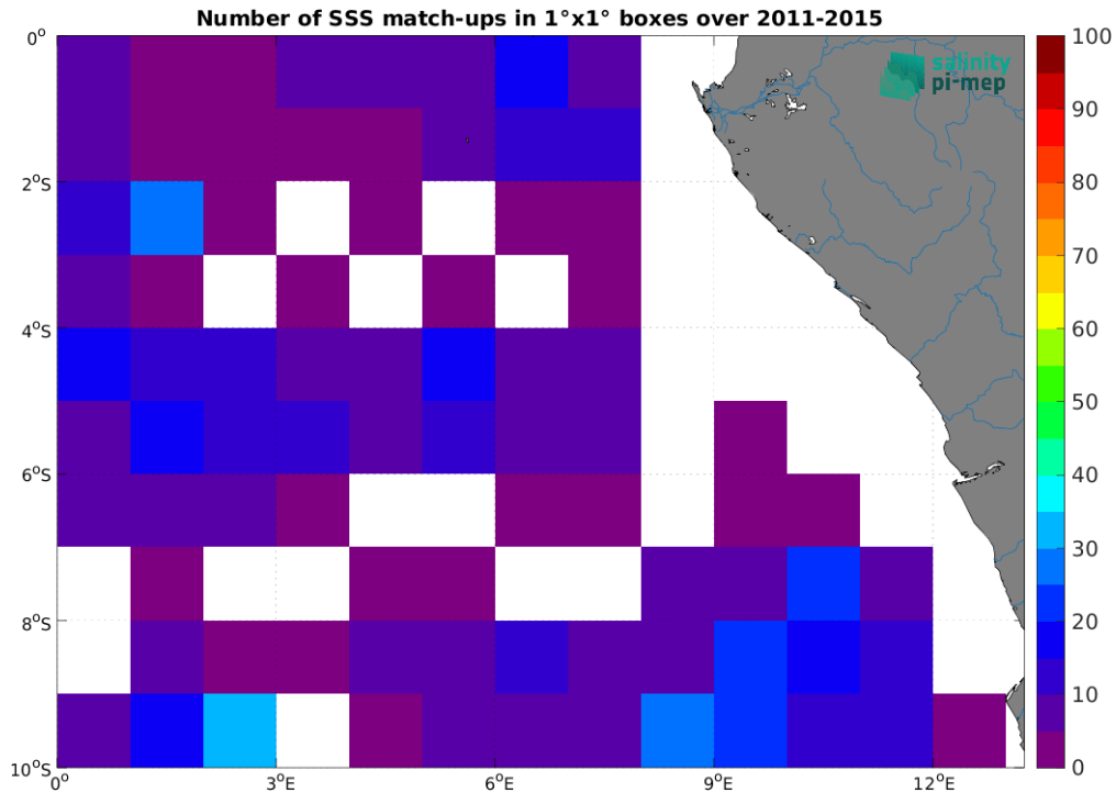
Figure 5: Number of SSS match-ups between Argo SSS and the Aquarius SSS L4 OI v5 - Monthly (IPRC) SSS product for the Congo river plume Pi-MEP region over 1^\circ \times 1^\circ boxes and for the full satellite product period.
