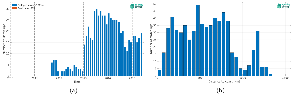
Figure 2: Number of match-ups between Argo and Aquarius SSS L4 OI v5 - Monthly (IPRC) SSS as a function of time (a) and as function of the distance to coast (b) over the Congo river plume Pi-MEP region and for the full satellite product period.
