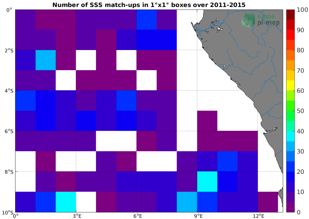
Figure 4: Number of SSS match-ups between Argo SSS and the Aquarius SSS L4 OI v5 - Monthly (IPRC) SSS product for the Congo river plume Pi-MEP region over 1°x1° boxes and for the full satellite product period.
