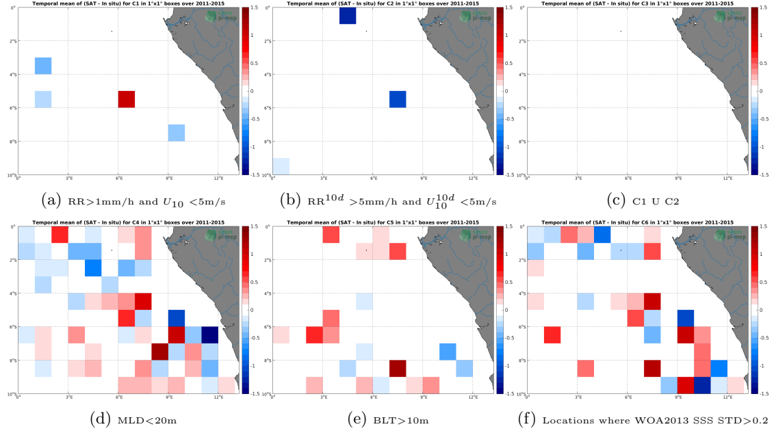
Figure 12: Temporal mean gridded over spatial boxes of size 1^\circ \times 1^\circ of \Delta SSS (Aquarius-L4-IPRC-V5-MONTHLY - Argo) for 6 different subdatasets corresponding to: RR > 1\text{mm/h} and U_{10} < 5\text{m/s} (a), RR^{10d} > 5\text{mm/h} and U_{10}^{10d} < 5\text{m/s} (b), C1 U C2 (c), MLD < 20\text{m} (d), BLT > 10\text{m} (e), Locations where WOA2013 SSS STD > 0.2 (f).
