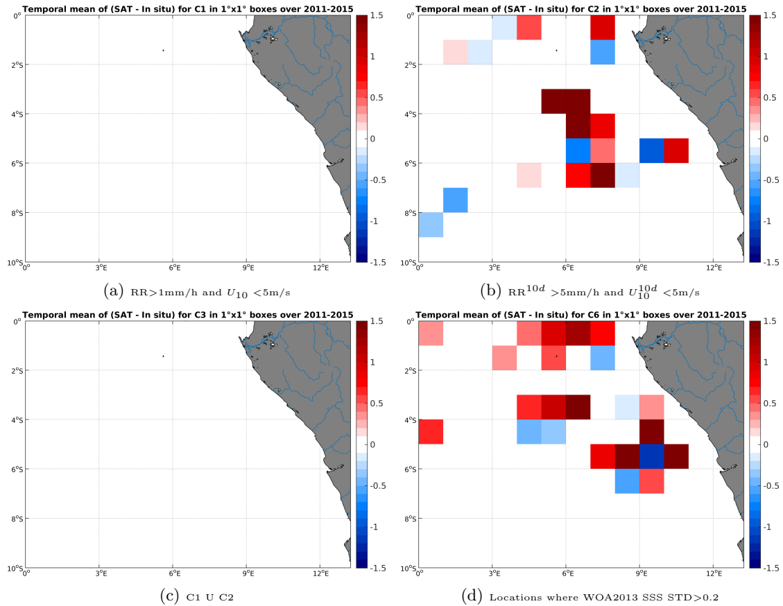
Figure 12: Temporal mean gridded over spatial boxes of size 1^\circ \times 1^\circ of \Delta SSS (Aquarius-L4-IPRC-V4-MONTHLY - TSG-GOSUD-Research-vessel) for 4 different subdatasets corresponding to: RR > 1mm/h and U_{10} < 5m/s (a), RR^{10d} > 5mm/h and U_{10}^{10d} < 5m/s (b), C1 \cup C2 (c), Locations where WOA2013 SSS STD > 0.2 (d).
