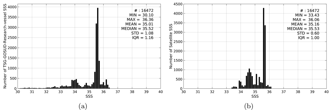
Figure 2: Histograms of SSS from TSG-GOSUD-Research-vessel (a) and Aquarius-L4-IPRC-V4-MONTHLY (b) considering all match-up pairs per bins of 0.1 over the Congo river plume Pi-MEP region and for the full satellite product period.
