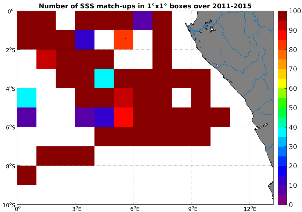
Figure 4: Number of SSS match-ups between TSG-GOSUD-Research-vessel SSS and the Aquarius-L4-IPRC-V4-MONTHLY SSS product for the Congo river plume Pi-MEP region over 1^\circ \times 1^\circ boxes and for the full satellite product period.
