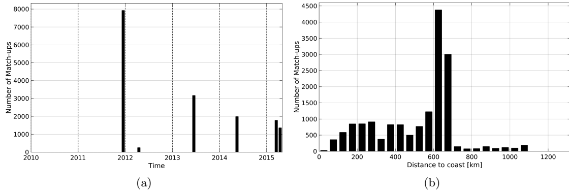
Figure 1: Number of match-ups between TSG-GOSUD-Research-vessel and Aquarius-L4-IPRC-V4-MONTHLY SSS as a function of time (a) and as function of the distance to coast (b) over the Congo river plume Pi-MEP region and for the full satellite product period.
