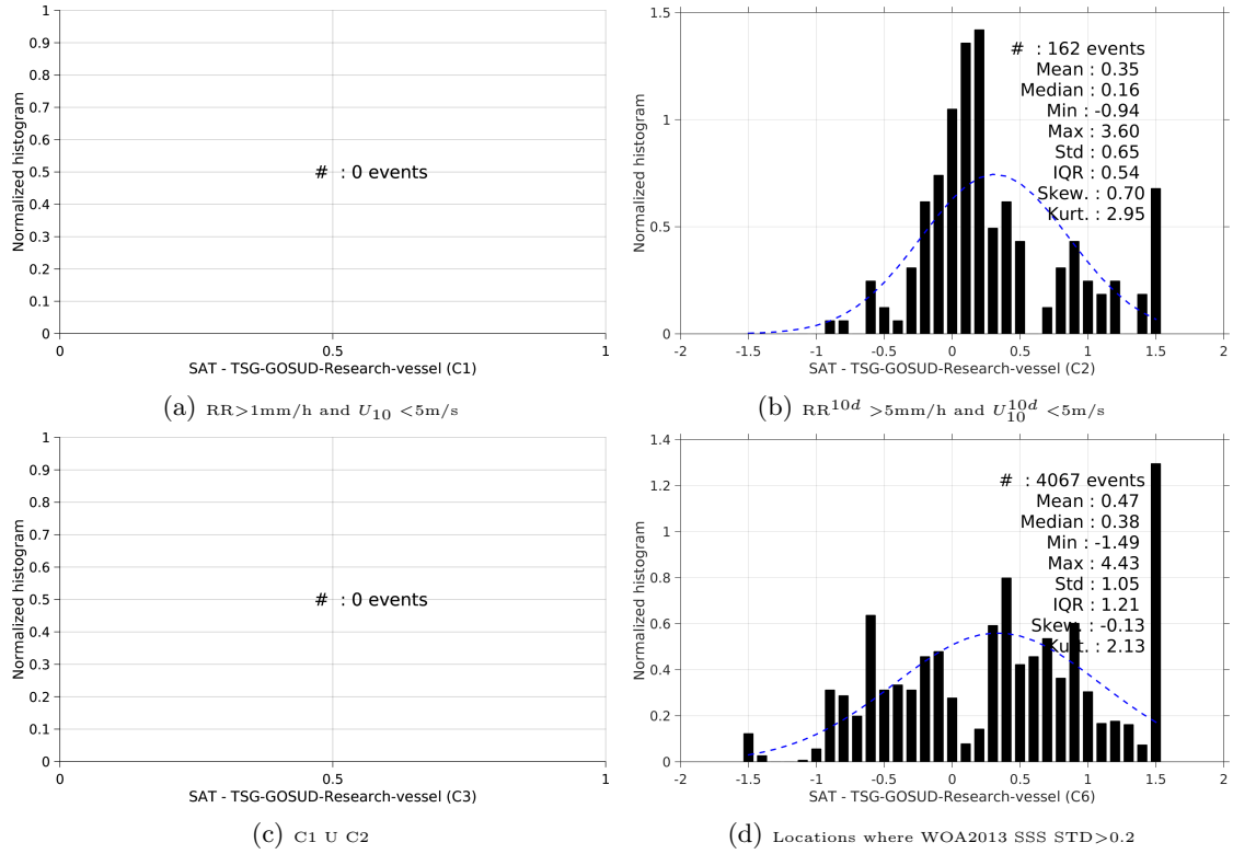
Figure 13: Normalized histogram of \Delta\text{SSS} (Aquarius-L4-IPRC-V4-MONTHLY - TSG-GOSUD-Research-vessel) for 6 different subdatasets corresponding to: RR > 1\text{mm/h} and U_{10} < 5\text{m/s} (a), RR^{10d} > 5\text{mm/h} and U_{10}^{10d} < 5\text{m/s} (b), C1 \cup C2 (c), Locations where WOA2013 SSS STD > 0.2 (d).
