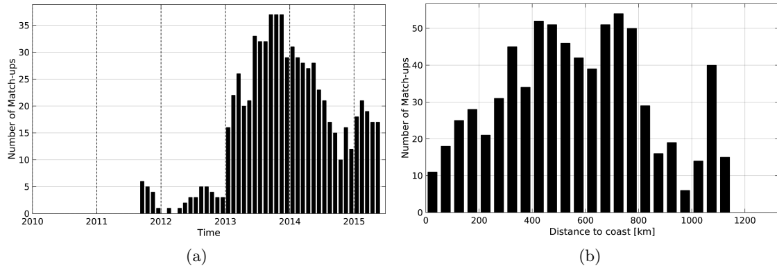
Figure 1: Number of match-ups between Argo and Aquarius-L4-IPRC-V4-MONTHLY SSS as a function of time (a) and as function of the distance to coast (b) over the Congo river plume Pi-MEP region and for the full satellite product period.
