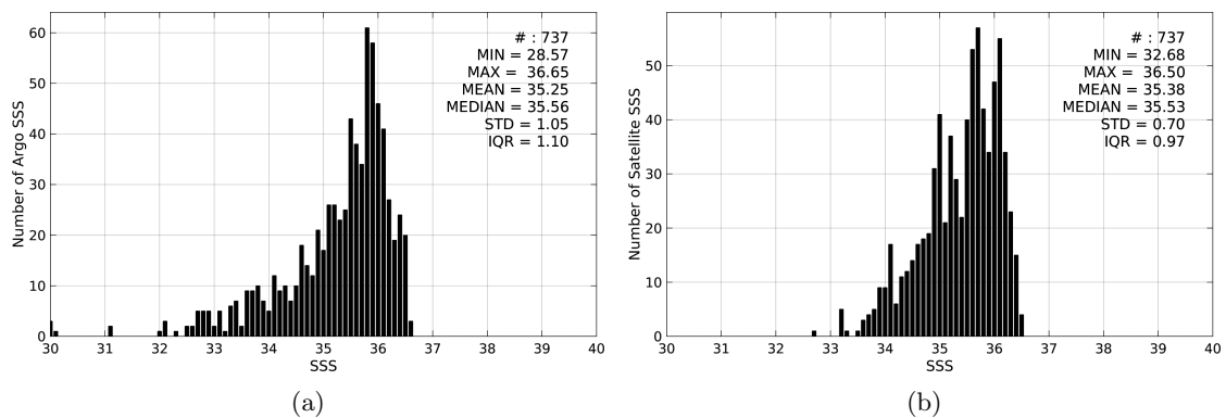
Figure 2: Histograms of SSS from Argo (a) and Aquarius-L4-IPRC-V4-MONTHLY (b) considering all match-up pairs per bins of 0.1 over the Congo river plume Pi-MEP region and for the full satellite product period.
