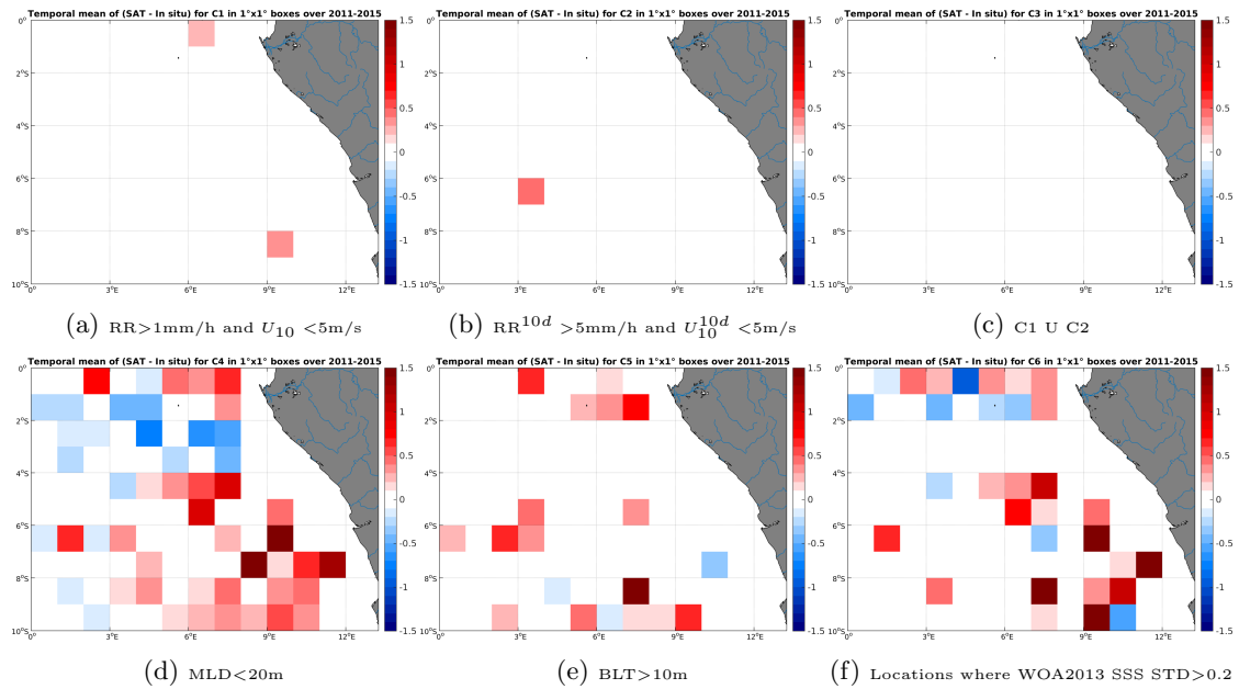
Figure 12: Temporal mean gridded over spatial boxes of size 1^\circ \times 1^\circ of \Delta SSS (Aquarius-L4-IPRC-V4-MONTHLY - Argo) for 6 different subdatasets corresponding to: RR > 1\text{mm/h} and U_{10} < 5\text{m/s} (a), RR^{10d} > 5\text{mm/h} and U_{10}^{10d} < 5\text{m/s} (b), C1 U C2 (c), MLD < 20\text{m} (d), BLT > 10\text{m} (e), Locations where WOA2013 SSS STD > 0.2 (f).
