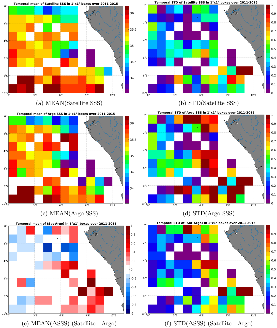
Figure 6: Temporal mean (left) and STD (right) of SSS from Aquarius-L4-IPRC-V4-MONTHLY (top), Argo (middle), and of \Delta SSS (Satellite - Argo). Only match-up pairs are used to generate these maps.
