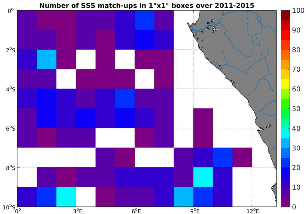
Figure 4: Number of SSS match-ups between Argo SSS and the Aquarius-L4-IPRC-V4-MONTHLY SSS product for the Congo river plume Pi-MEP region over 1^\circ \times 1^\circ boxes and for the full satellite product period.
