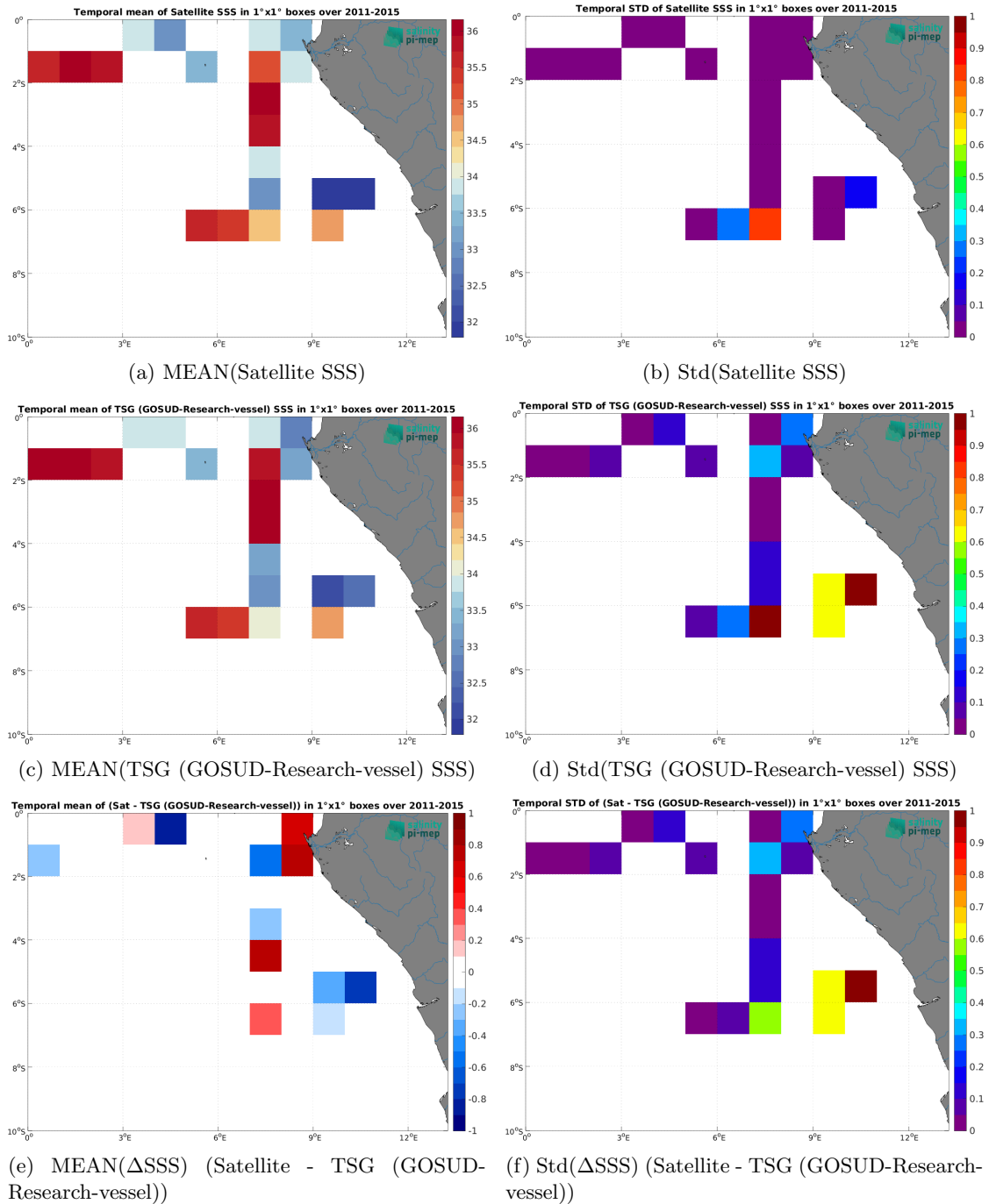
Figure 7: Temporal mean (left) and Std (right) of SSS from Aquarius SSS L3 OR v5 - 7-Day running (NASA-GSFC) (top), TSG (GOSUD-Research-vessel) (middle), and of \Delta SSS (Satellite - TSG (GOSUD-Research-vessel)). Only match-up pairs are used to generate these maps.
