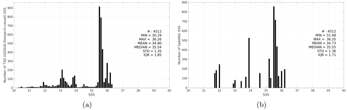
Figure 3: Histograms of SSS from TSG (GOSUD-Research-vessel) (a) and Aquarius SSS L3 OR v5 - 7-Day running (NASA-GSFC) (b) considering all match-up pairs per bins of 0.1 over the Congo river plume Pi-MEP region and for the full satellite product period.
