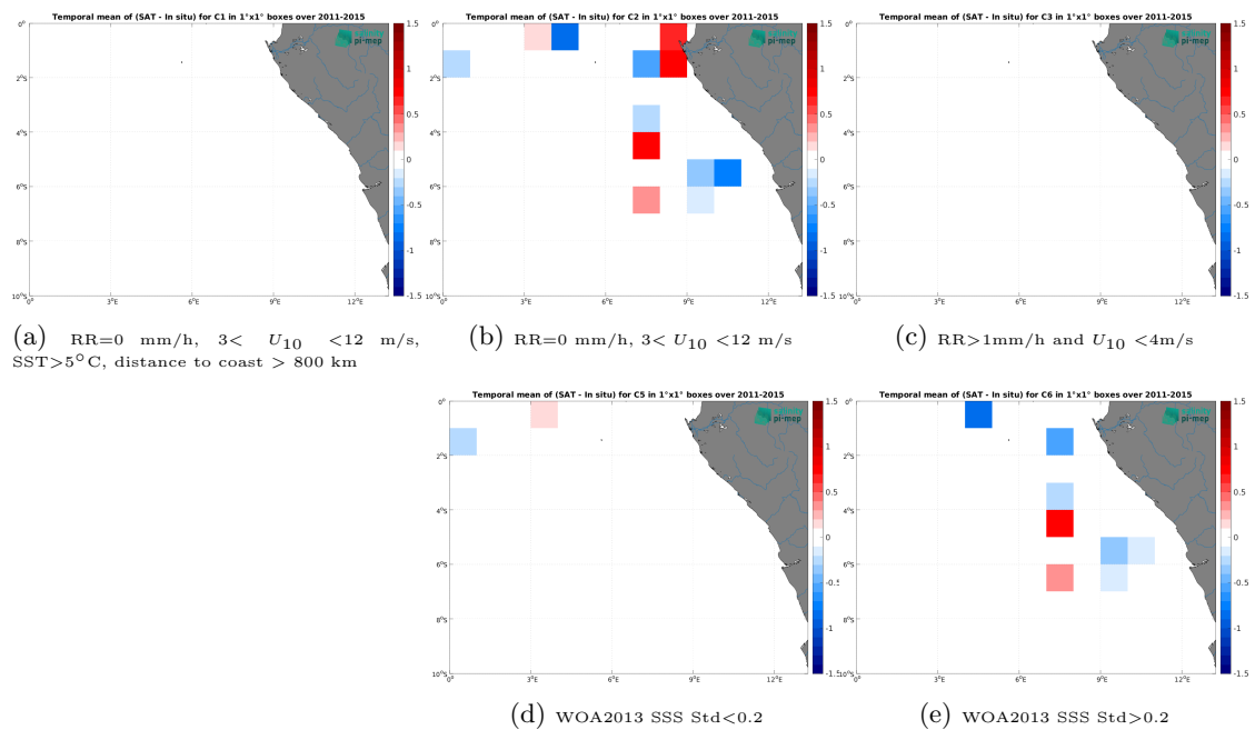
Figure 14: Temporal mean gridded over spatial boxes of size 1^\circ \times 1^\circ of \Delta SSS (Aquarius SSS L3 OR v5 - 7-Day running (NASA-GSFC) - TSG (GOSUD-Research-vessel)) for 5 different subdatasets corresponding to:RR=0 mm/h, 3 < U_{10} < 12 m/s, SST > 5^\circ\text{C} , distance to coast > 800 km (a), RR=0 mm/h, 3 < U_{10} < 12 m/s (b), RR > 1 mm/h and U_{10} < 4 m/s (c), WOA2013 SSS Std < 0.2 (d), WOA2013 SSS Std > 0.2 (e).
