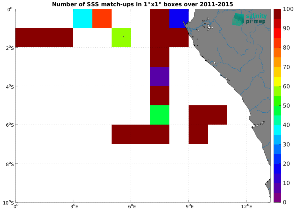
Figure 5: Number of SSS match-ups between TSG (GOSUD-Research-vessel) SSS and the Aquarius SSS L3 OR v5 - 7-Day running (NASA-GSFC) SSS product for the Congo river plume Pi-MEP region over 1^\circ \times 1^\circ boxes and for the full satellite product period.
