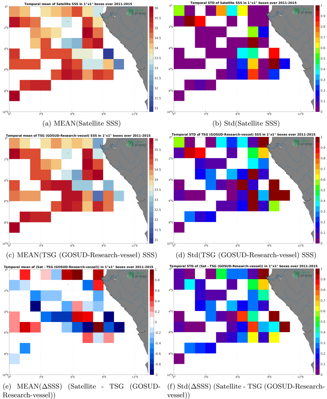
Figure 6: Temporal mean (left) and Std (right) of SSS from Aquarius SSS L3 OR v5 - 7-Day running (NASA-GSFC) (top), TSG (GOSUD-Research-vessel) (middle), and of \Delta SSS (Satellite - TSG (GOSUD-Research-vessel)). Only match-up pairs are used to generate these maps.
