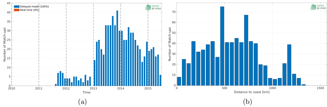
Figure 1: Number of match-ups between Argo and Aquarius SSS L3 OR v5 - 7-Day running (NASA-GSFC) SSS as a function of time (a) and as function of the distance to coast (b) over the Congo river plume Pi-MEP region and for the full satellite product period.
