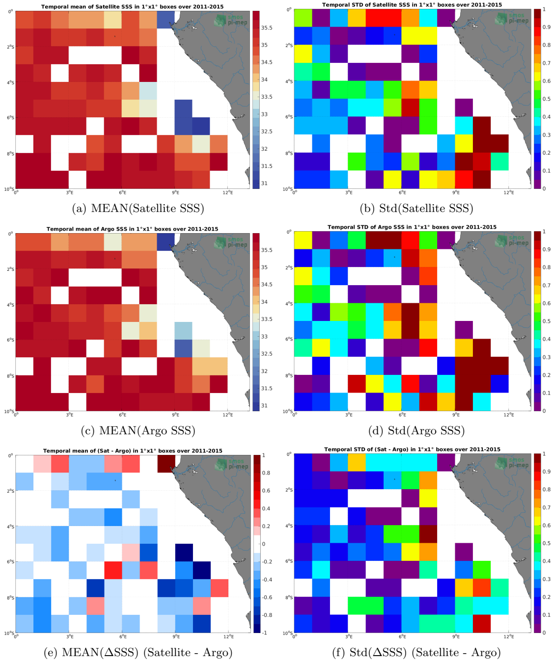
Figure 6: Temporal mean (left) and Std (right) of SSS from Aquarius SSS L3 OR v5 - 7-Day running (NASA-GSFC) (top), Argo (middle), and of \Delta SSS (Satellite - Argo). Only match-up pairs are used to generate these maps.
