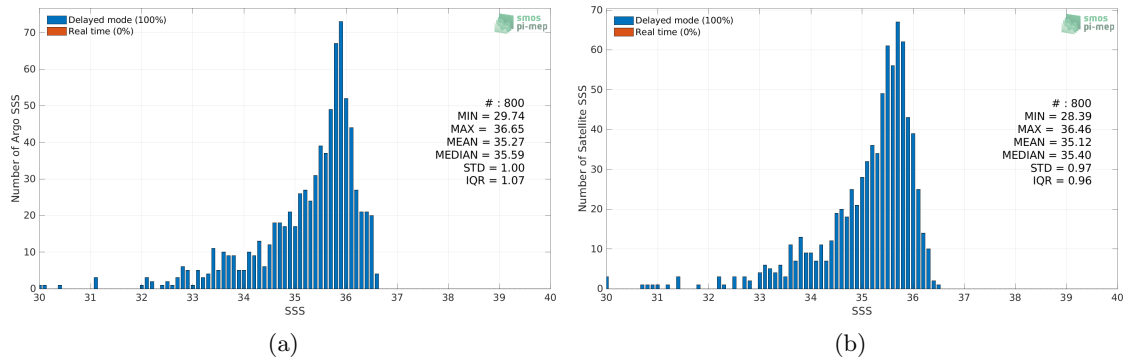
Figure 2: Histograms of SSS from Argo (a) and Aquarius SSS L3 OR v5 - 7-Day running (NASA-GSFC) (b) considering all match-up pairs per bins of 0.1 over the Congo river plume Pi-MEP region and for the full satellite product period.
