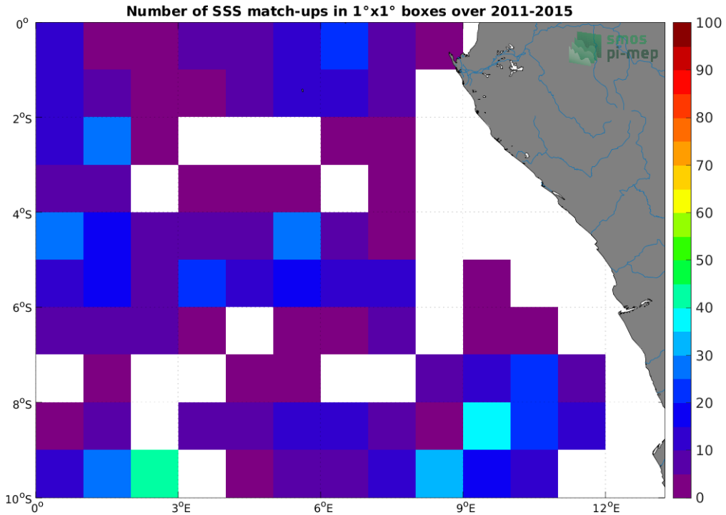
Figure 4: Number of SSS match-ups between Argo SSS and the Aquarius SSS L3 OR v5 - 7-Day running (NASA-GSFC) SSS product for the Congo river plume Pi-MEP region over 1^\circ \times 1^\circ boxes and for the full satellite product period.
