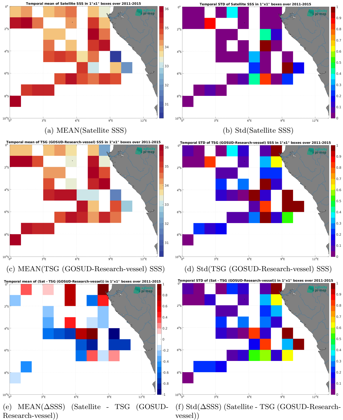
Figure 7: Temporal mean (left) and Std (right) of SSS from Aquarius SSS L3 OR v5 - 7-Day running - Rain mask (NASA-GSFC) (top), TSG (GOSUD-Research-vessel) (middle), and of \Delta SSS (Satellite - TSG (GOSUD-Research-vessel)). Only match-up pairs are used to generate these maps.
