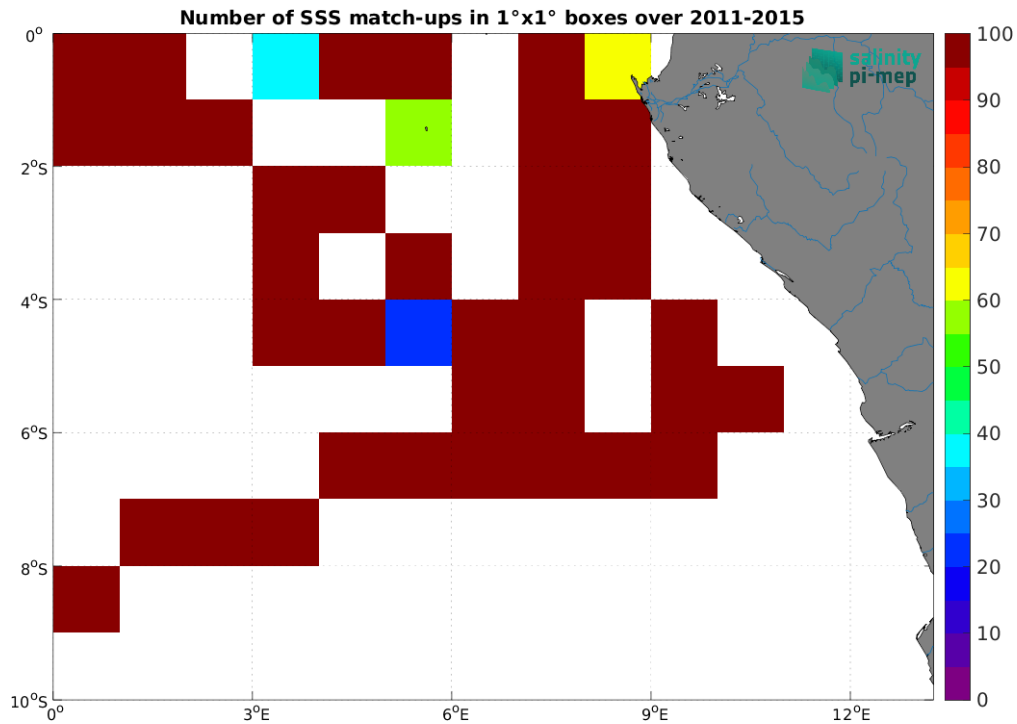
Figure 5: Number of SSS match-ups between TSG (GOSUD-Research-vessel) SSS and the Aquarius SSS L3 OR v5 - 7-Day running - Rain mask (NASA-GSFC) SSS product for the Congo river plume Pi-MEP region over 1^\circ \times 1^\circ boxes and for the full satellite product period.
