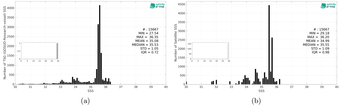
Figure 3: Histograms of SSS from TSG (GOSUD-Research-vessel) (a) and Aquarius SSS L3 OR v5 - 7-Day running - Rain mask (NASA-GSFC) (b) considering all match-up pairs per bins of 0.1 over the Congo river plume Pi-MEP region and for the full satellite product period.
