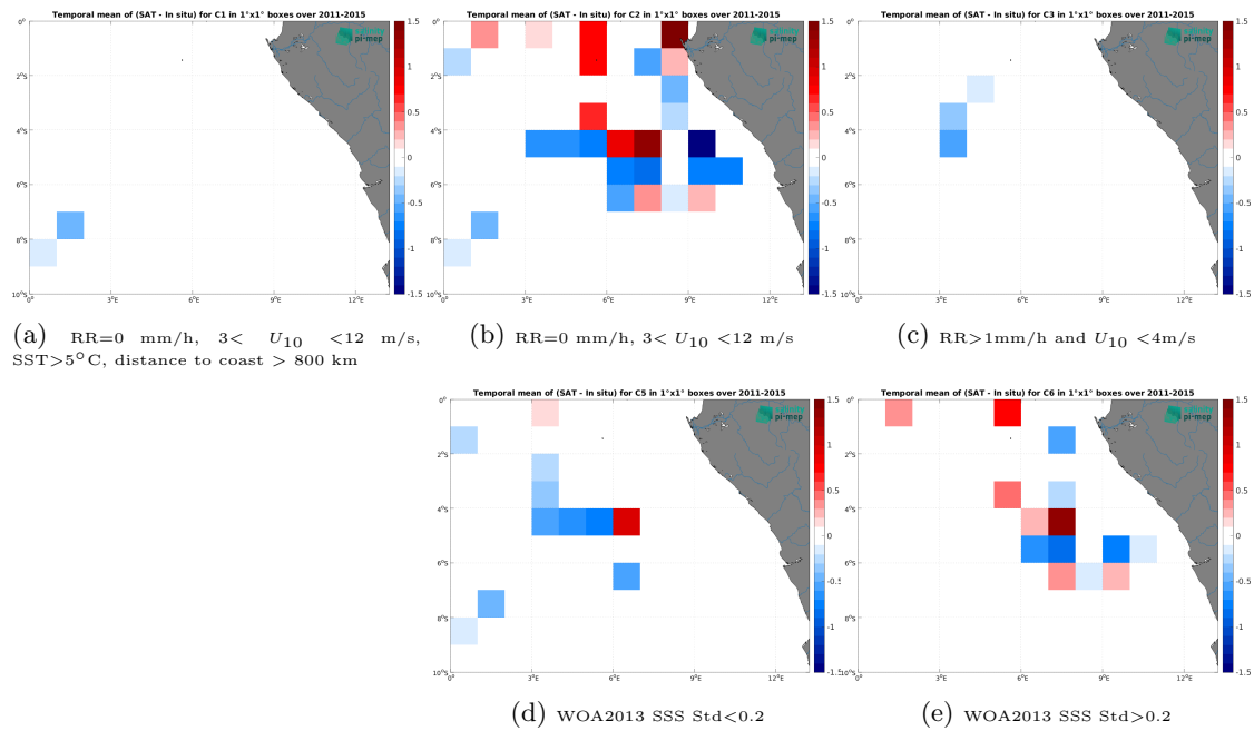
Figure 14: Temporal mean gridded over spatial boxes of size 1^\circ \times 1^\circ of \Delta SSS (Aquarius SSS L3 OR v5 - 7-Day running - Rain mask (NASA-GSFC) - TSG (GOSUD-Research-vessel)) for 5 different subdatasets corresponding to:RR=0 mm/h, 3 < U_{10} < 12 m/s, SST > 5^\circ\text{C} , distance to coast > 800 km (a), RR=0 mm/h, 3 < U_{10} < 12 m/s (b), RR > 1 mm/h and U_{10} < 4 m/s (c), WOA2013 SSS Std < 0.2 (d), WOA2013 SSS Std > 0.2 (e).
