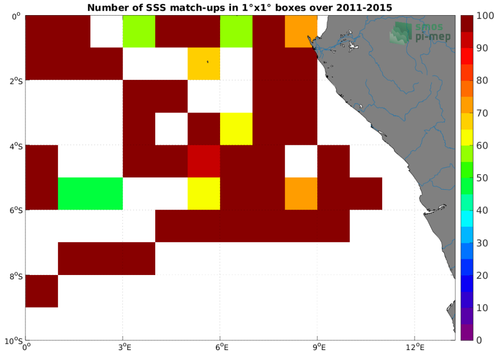
Figure 4: Number of SSS match-ups between TSG (GOSUD-Research-vessel) SSS and the Aquarius SSS L3 OR v5 - 7-Day running - Rain mask (NASA-GSFC) SSS product for the Congo river plume Pi-MEP region over 1^\circ \times 1^\circ boxes and for the full satellite product period.
