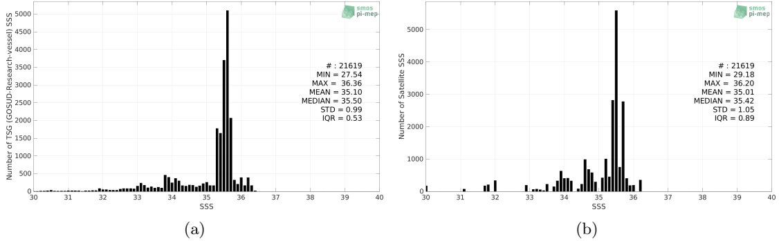
Figure 2: Histograms of SSS from TSG (GOSUD-Research-vessel) (a) and Aquarius SSS L3 OR v5 - 7-Day running - Rain mask (NASA-GSFC) (b) considering all match-up pairs per bins of 0.1 over the Congo river plume Pi-MEP region and for the full satellite product period.
