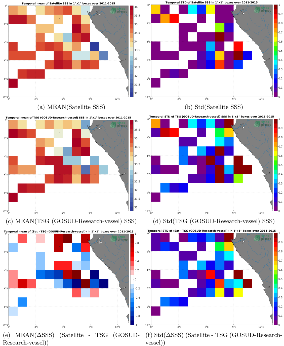
Figure 6: Temporal mean (left) and Std (right) of SSS from Aquarius SSS L3 OR v5 - 7-Day running - Rain mask (NASA-GSFC) (top), TSG (GOSUD-Research-vessel) (middle), and of \Delta SSS (Satellite - TSG (GOSUD-Research-vessel)). Only match-up pairs are used to generate these maps.
