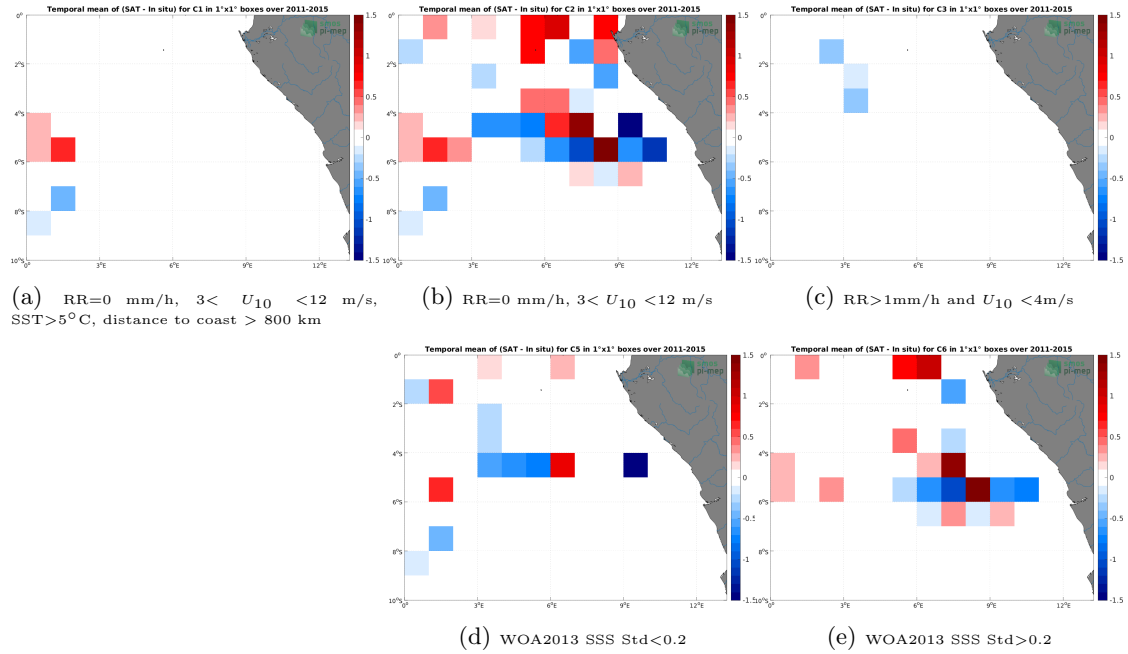
Figure 12: Temporal mean gridded over spatial boxes of size 1^\circ \times 1^\circ of \Delta SSS (Aquarius SSS L3 OR v5 - 7-Day running - Rain mask (NASA-GSFC) - TSG (GOSUD-Research-vessel)) for 5 different subdatasets corresponding to:RR=0 mm/h, 3 < U_{10} < 12 m/s, SST >5^\circ\text{C} , distance to coast > 800 km (a), RR=0 mm/h, 3 < U_{10} < 12 m/s (b), RR >1 mm/h and U_{10} < 4 m/s (c), WOA2013 SSS Std <0.2 (d), WOA2013 SSS Std >0.2 (e).
