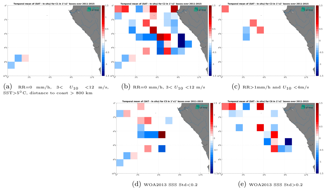
Figure 14: Temporal mean gridded over spatial boxes of size 1^\circ \times 1^\circ of \Delta SSS (Aquarius SSS L3 OR v5 - Monthly (NASA-GSFC) - TSG (GOSUD-Research-vessel)) for 5 different subdatasets corresponding to:RR=0 mm/h, 3 < U_{10} < 12 m/s, SST > 5^\circ\text{C} , distance to coast > 800 km (a), RR=0 mm/h, 3 < U_{10} < 12 m/s (b), RR > 1 mm/h and U_{10} < 4 m/s (c), WOA2013 SSS Std < 0.2 (d), WOA2013 SSS Std > 0.2 (e).
