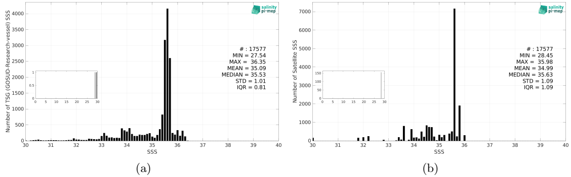
Figure 3: Histograms of SSS from TSG (GOSUD-Research-vessel) (a) and Aquarius SSS L3 OR v5 - Monthly (NASA-GSFC) (b) considering all match-up pairs per bins of 0.1 over the Congo river plume Pi-MEP region and for the full satellite product period.
