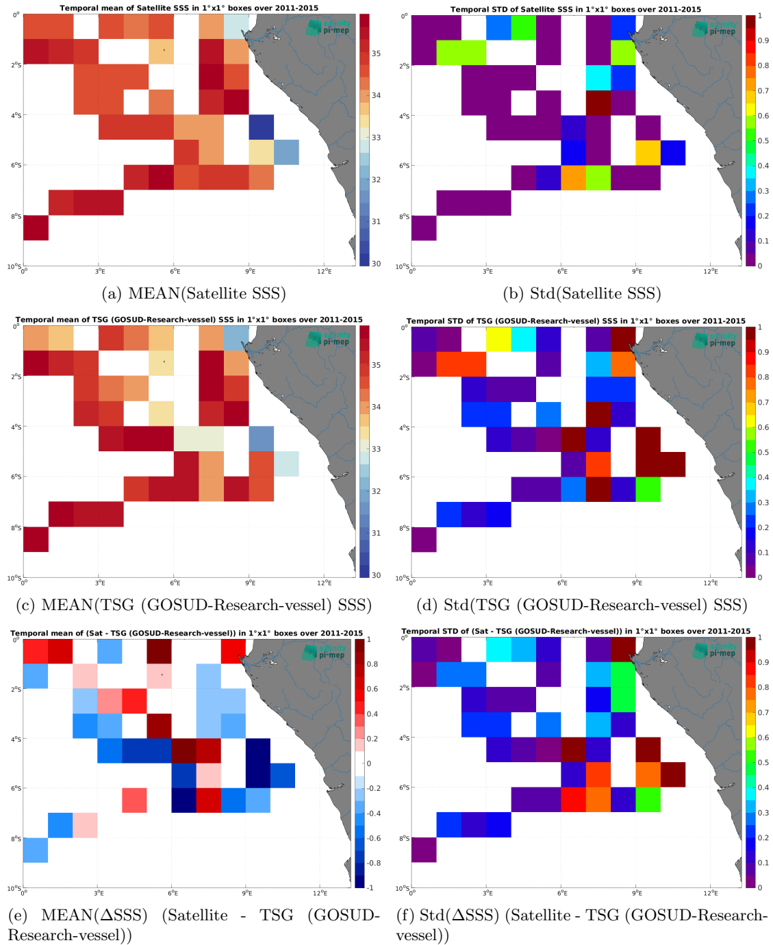
Figure 7: Temporal mean (left) and Std (right) of SSS from Aquarius SSS L3 OR v5 - Monthly (NASA-GSFC) (top), TSG (GOSUD-Research-vessel) (middle), and of \Delta SSS (Satellite - TSG (GOSUD-Research-vessel)). Only match-up pairs are used to generate these maps.
