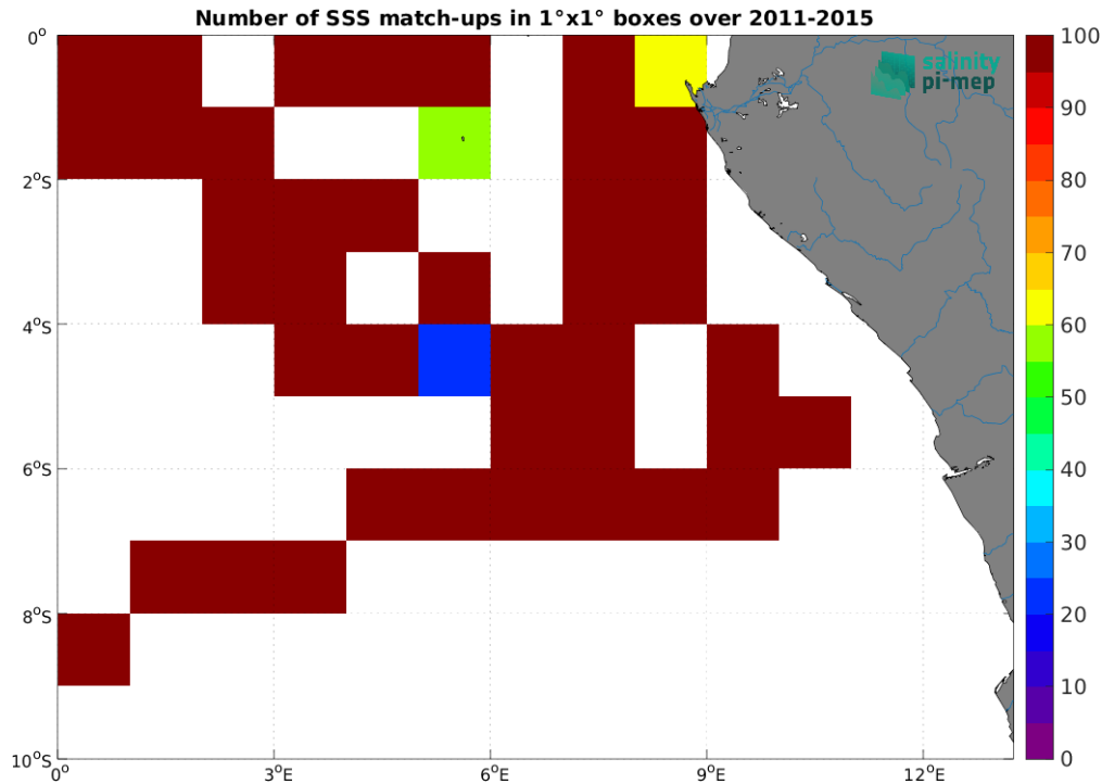
Figure 5: Number of SSS match-ups between TSG (GOSUD-Research-vessel) SSS and the Aquarius SSS L3 OR v5 - Monthly (NASA-GSFC) SSS product for the Congo river plume Pi-MEP region over 1^\circ \times 1^\circ boxes and for the full satellite product period.
