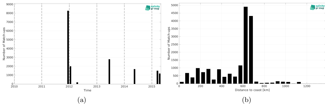
Figure 2: Number of match-ups between TSG (GOSUD-Research-vessel) and Aquarius SSS L3 OR v5 - Monthly (NASA-GSFC) SSS as a function of time (a) and as function of the distance to coast (b) over the Congo river plume Pi-MEP region and for the full satellite product period.
