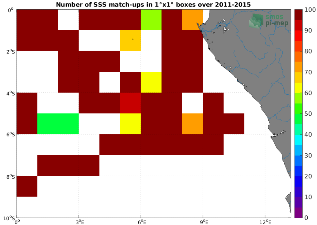
Figure 4: Number of SSS match-ups between TSG (GOSUD-Research-vessel) SSS and the Aquarius SSS L3 OR v5 - Monthly (NASA-GSFC) SSS product for the Congo river plume Pi-MEP region over 1^\circ \times 1^\circ boxes and for the full satellite product period.
