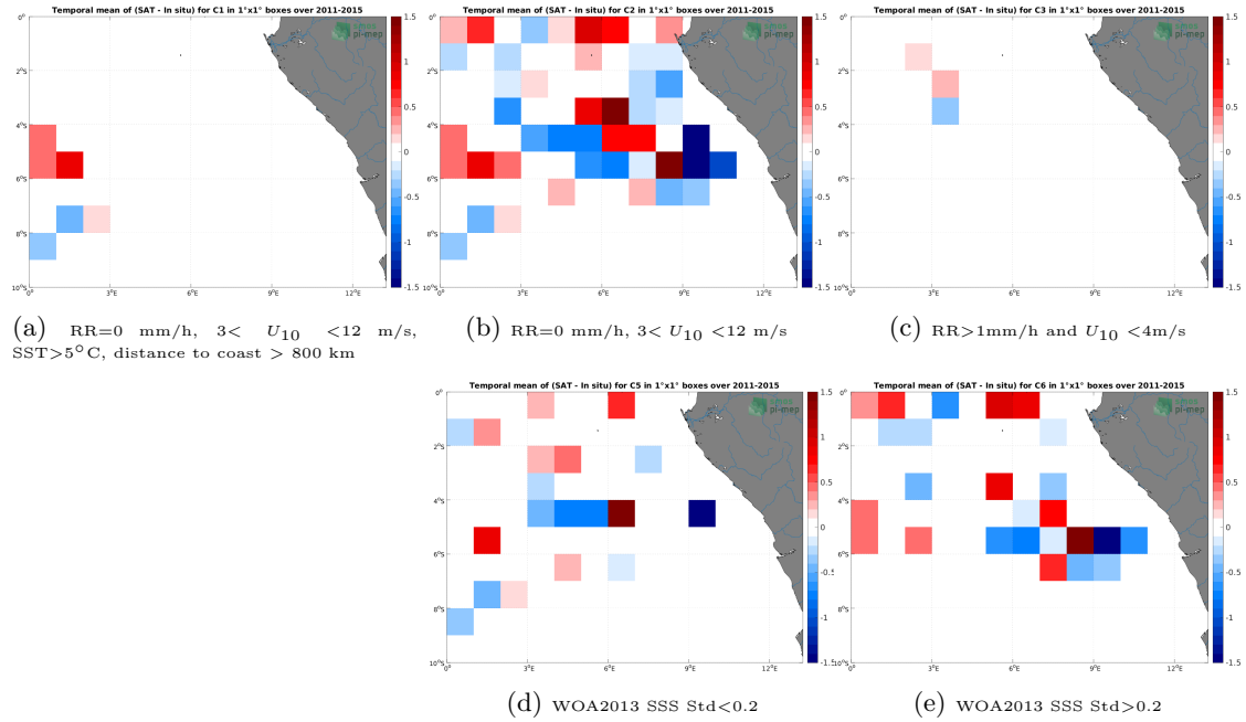
Figure 12: Temporal mean gridded over spatial boxes of size 1^\circ \times 1^\circ of \Delta SSS (Aquarius SSS L3 OR v5 - Monthly (NASA-GSFC) - TSG (GOSUD-Research-vessel)) for 5 different subdatasets corresponding to:RR=0 mm/h, 3 < U_{10} < 12 m/s, SST >5^\circ\text{C} , distance to coast > 800 km (a), RR=0 mm/h, 3 < U_{10} < 12 m/s (b), RR >1 mm/h and U_{10} < 4 m/s (c), WOA2013 SSS Std <0.2 (d), WOA2013 SSS Std >0.2 (e).
