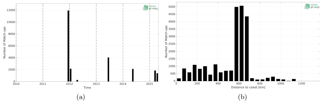
Figure 1: Number of match-ups between TSG (GOSUD-Research-vessel) and Aquarius SSS L3 OR v5 - Monthly (NASA-GSFC) SSS as a function of time (a) and as function of the distance to coast (b) over the Congo river plume Pi-MEP region and for the full satellite product period.
