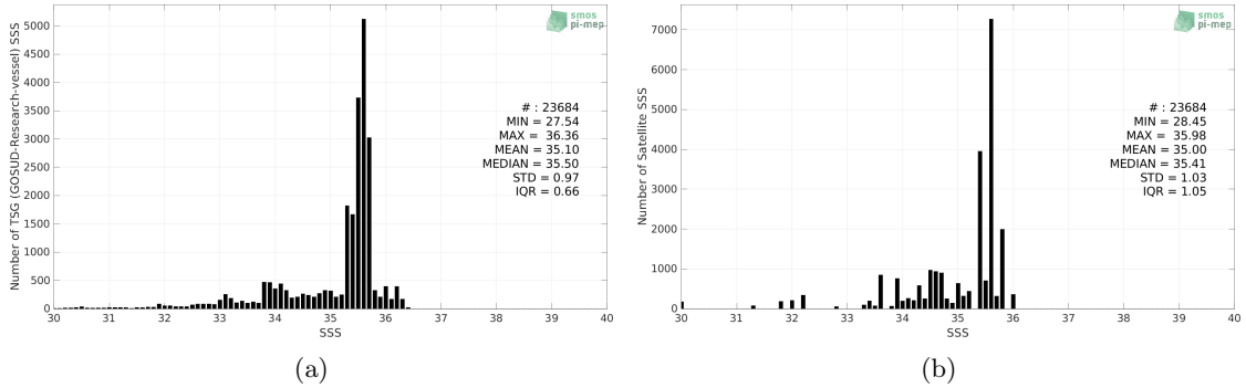
Figure 2: Histograms of SSS from TSG (GOSUD-Research-vessel) (a) and Aquarius SSS L3 OR v5 - Monthly (NASA-GSFC) (b) considering all match-up pairs per bins of 0.1 over the Congo river plume Pi-MEP region and for the full satellite product period.
