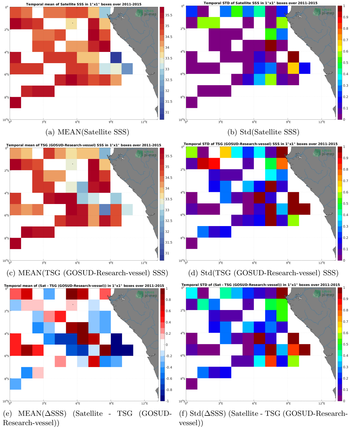
Figure 6: Temporal mean (left) and Std (right) of SSS from Aquarius SSS L3 OR v5 - Monthly (NASA-GSFC) (top), TSG (GOSUD-Research-vessel) (middle), and of \Delta SSS (Satellite - TSG (GOSUD-Research-vessel)). Only match-up pairs are used to generate these maps.
