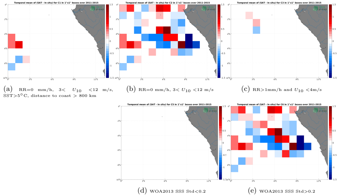
Figure 12: Temporal mean gridded over spatial boxes of size 1^{\circ}\times 1^{\circ} of \Delta SSS (Aquarius SSS L3 OR v5 - Monthly (NASA-GSFC) - TSG (GOSUD-Research-vessel)) for 5 different subdatasets corresponding to:RR=0 mm/h, 3 < U_{10} < 12 m/s, SST >5^{\circ}\text{C} , distance to coast > 800 km (a), RR=0 mm/h, 3 < U_{10} < 12 m/s (b), RR >1 mm/h and U_{10} < 4 m/s (c), WOA2013 SSS Std <0.2 (d), WOA2013 SSS Std >0.2 (e).
