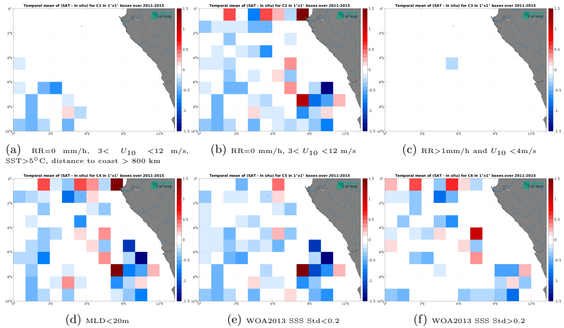
Figure 14: Temporal mean gridded over spatial boxes of size 1^\circ \times 1^\circ of \Delta SSS (Aquarius SSS L3 OR v5 - Monthly (NASA-GSFC) - Argo) for 6 different subdatasets corresponding to:RR=0 mm/h, 3 < U_{10} < 12 m/s, SST >5^\circ C, distance to coast > 800 km (a), RR=0 mm/h, 3 < U_{10} < 12 m/s (b), RR >1 mm/h and U_{10} < 4 m/s (c),MLD <20 m (d),WOA2013 SSS Std <0.2 (e),WOA2013 SSS Std >0.2 (f).
