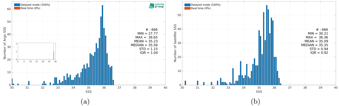
Figure 3: Histograms of SSS from Argo (a) and Aquarius SSS L3 OR v5 - Monthly (NASA-GSFC) (b) considering all match-up pairs per bins of 0.1 over the Congo river plume Pi-MEP region and for the full satellite product period.
