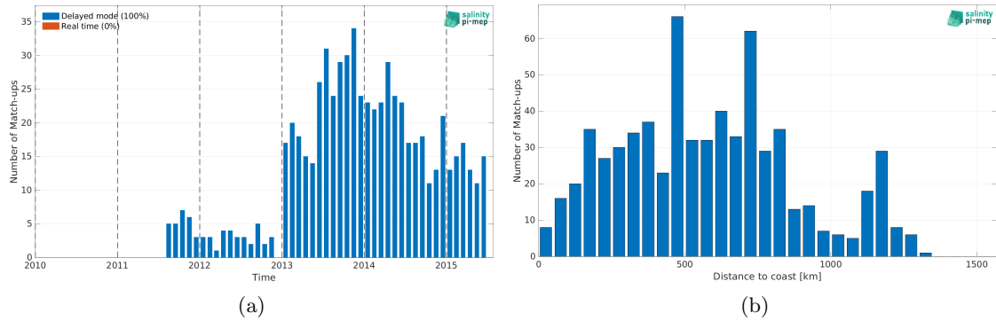
Figure 2: Number of match-ups between Argo and Aquarius SSS L3 OR v5 - Monthly (NASA-GSFC) SSS as a function of time (a) and as function of the distance to coast (b) over the Congo river plume Pi-MEP region and for the full satellite product period.
