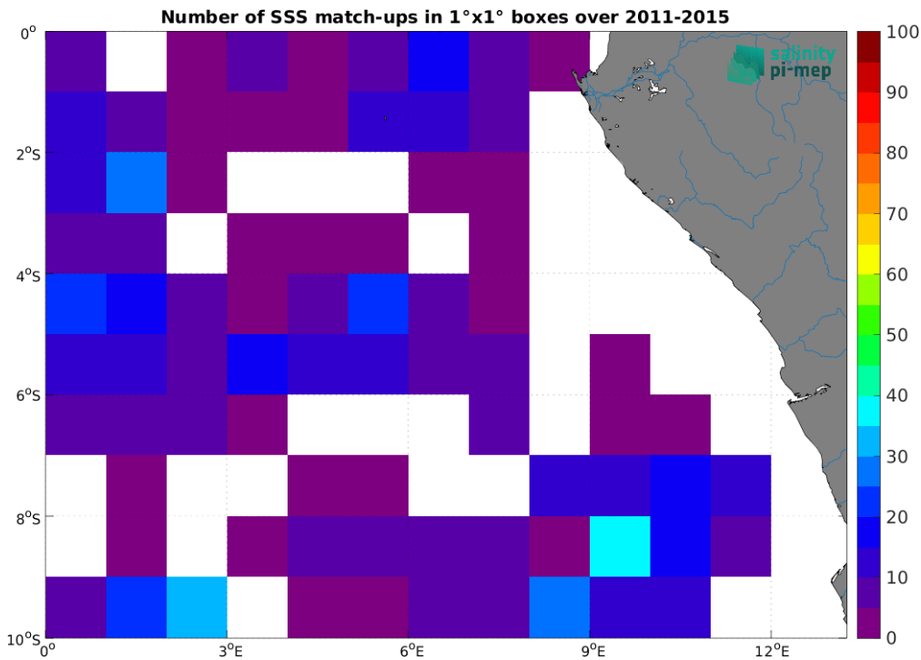
Figure 5: Number of SSS match-ups between Argo SSS and the Aquarius SSS L3 OR v5 - Monthly (NASA-GSFC) SSS product for the Congo river plume Pi-MEP region over 1^\circ \times 1^\circ boxes and for the full satellite product period.
