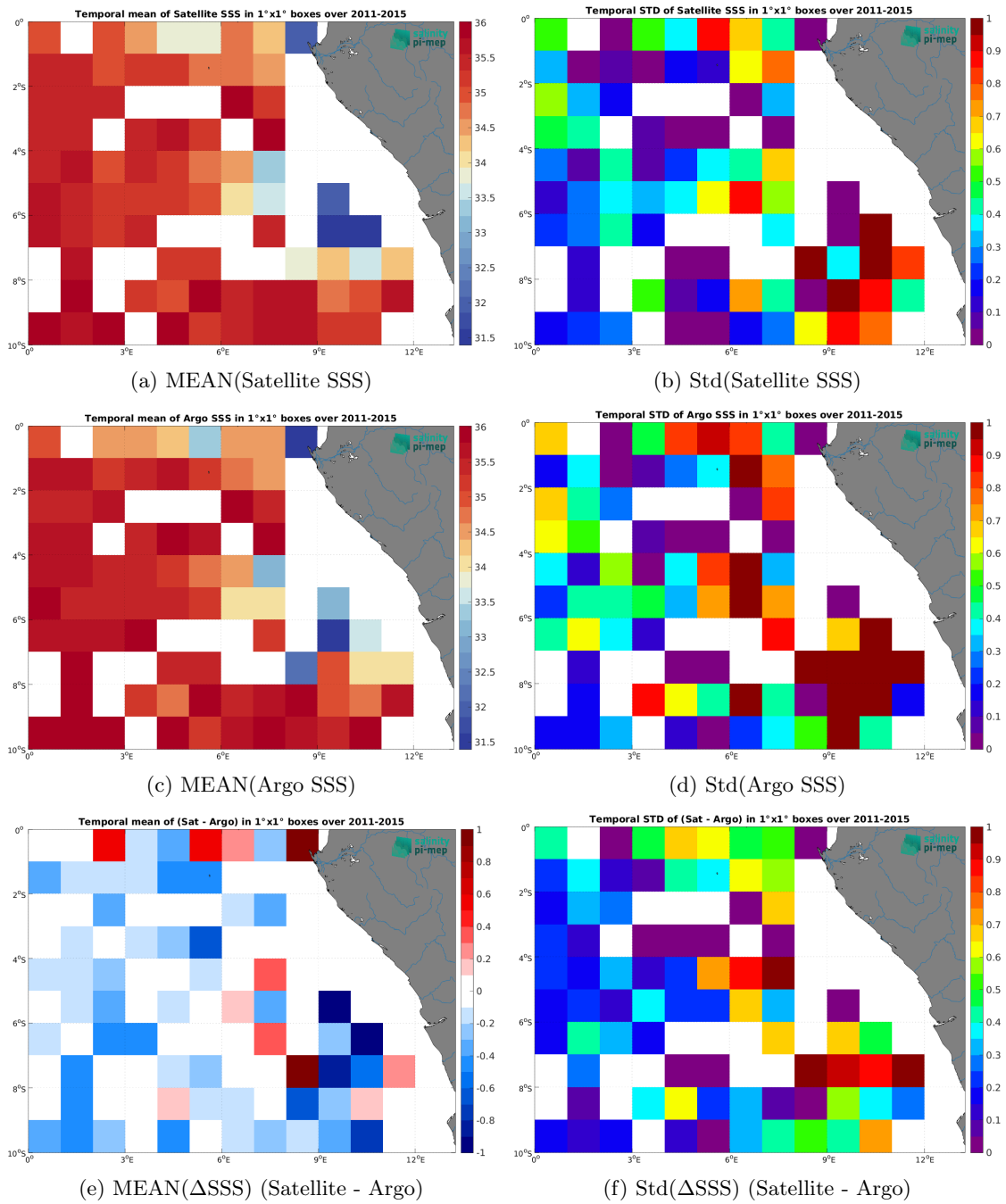
Figure 7: Temporal mean (left) and Std (right) of SSS from Aquarius SSS L3 OR v5 - Monthly (NASA-GSFC) (top), Argo (middle), and of \Delta SSS (Satellite - Argo). Only match-up pairs are used to generate these maps.
