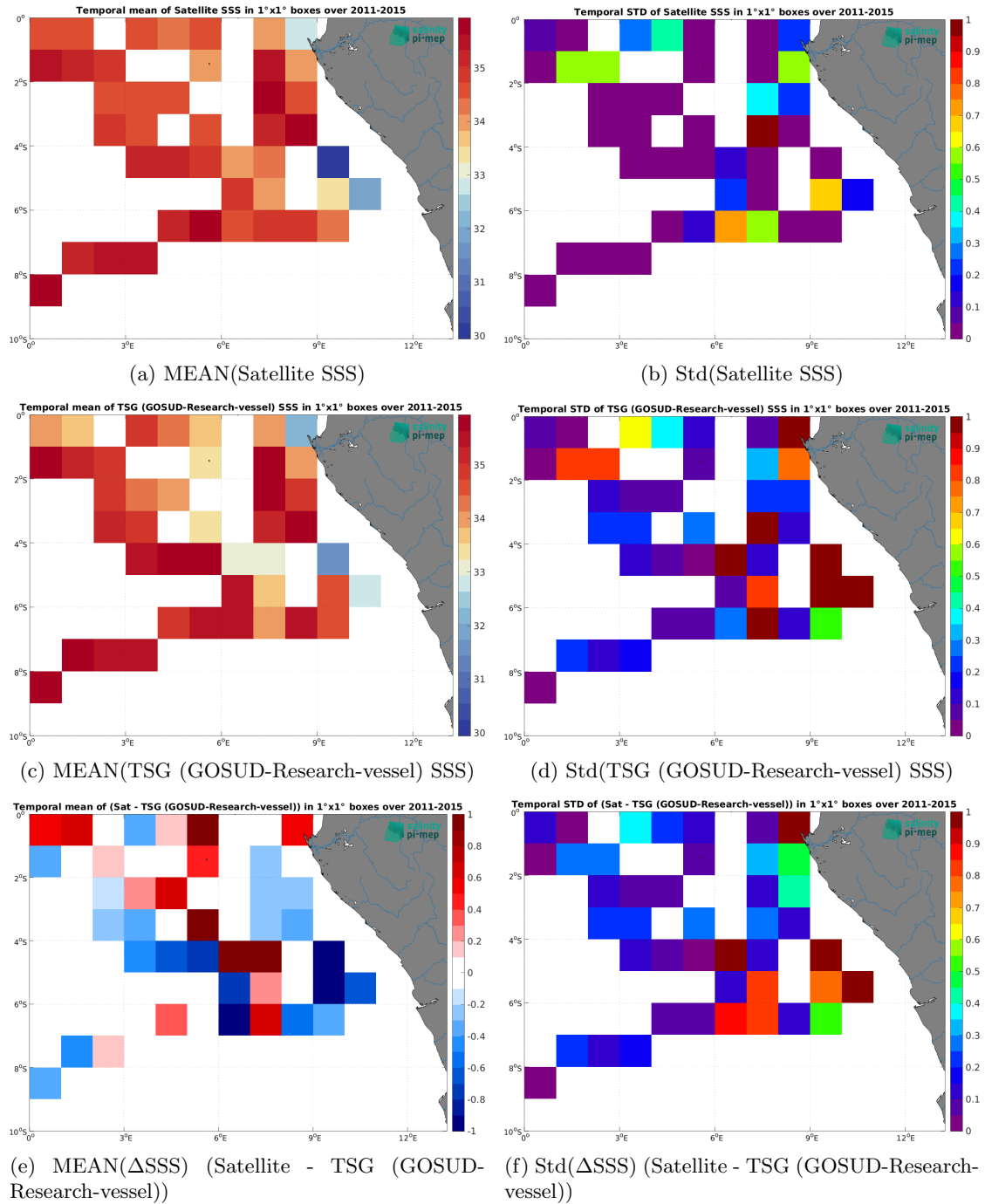
Figure 7: Temporal mean (left) and Std (right) of SSS from Aquarius SSS L3 OR v5 - Monthly - Rain mask (NASA-GSFC) (top), TSG (GOSUD-Research-vessel) (middle), and of \Delta SSS (Satellite - TSG (GOSUD-Research-vessel)). Only match-up pairs are used to generate these maps.
