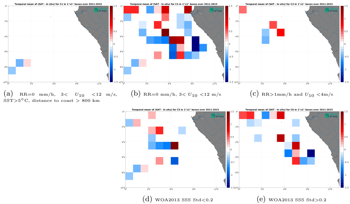
Figure 14: Temporal mean gridded over spatial boxes of size 1^\circ \times 1^\circ of \Delta SSS (Aquarius SSS L3 OR v5 - Monthly - Rain mask (NASA-GSFC) - TSG (GOSUD-Research-vessel)) for 5 different subdatasets corresponding to:RR=0 mm/h, 3 < U_{10} < 12 m/s, SST > 5^\circ\text{C} , distance to coast > 800 km (a), RR=0 mm/h, 3 < U_{10} < 12 m/s (b), RR > 1 mm/h and U_{10} < 4 m/s (c), WOA2013 SSS Std < 0.2 (d), WOA2013 SSS Std > 0.2 (e).
