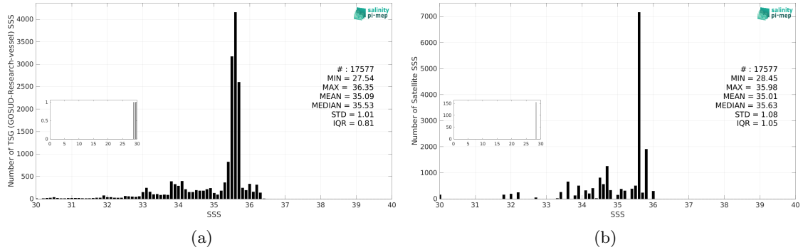
Figure 3: Histograms of SSS from TSG (GOSUD-Research-vessel) (a) and Aquarius SSS L3 OR v5 - Monthly - Rain mask (NASA-GSFC) (b) considering all match-up pairs per bins of 0.1 over the Congo river plume Pi-MEP region and for the full satellite product period.
