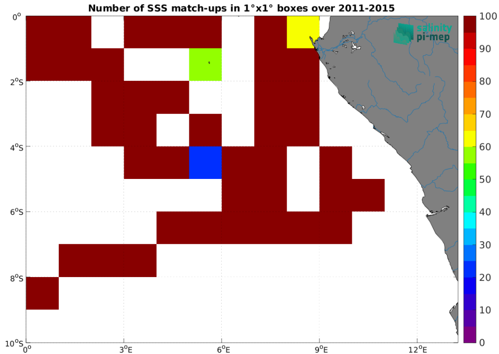
Figure 5: Number of SSS match-ups between TSG (GOSUD-Research-vessel) SSS and the Aquarius SSS L3 OR v5 - Monthly - Rain mask (NASA-GSFC) SSS product for the Congo river plume Pi-MEP region over 1^\circ \times 1^\circ boxes and for the full satellite product period.
